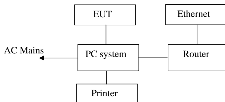
Figure 2 EUT Setup of Connect to PC mode
