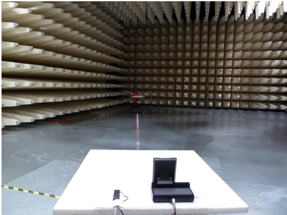
Photo 4: Radiated Emission
