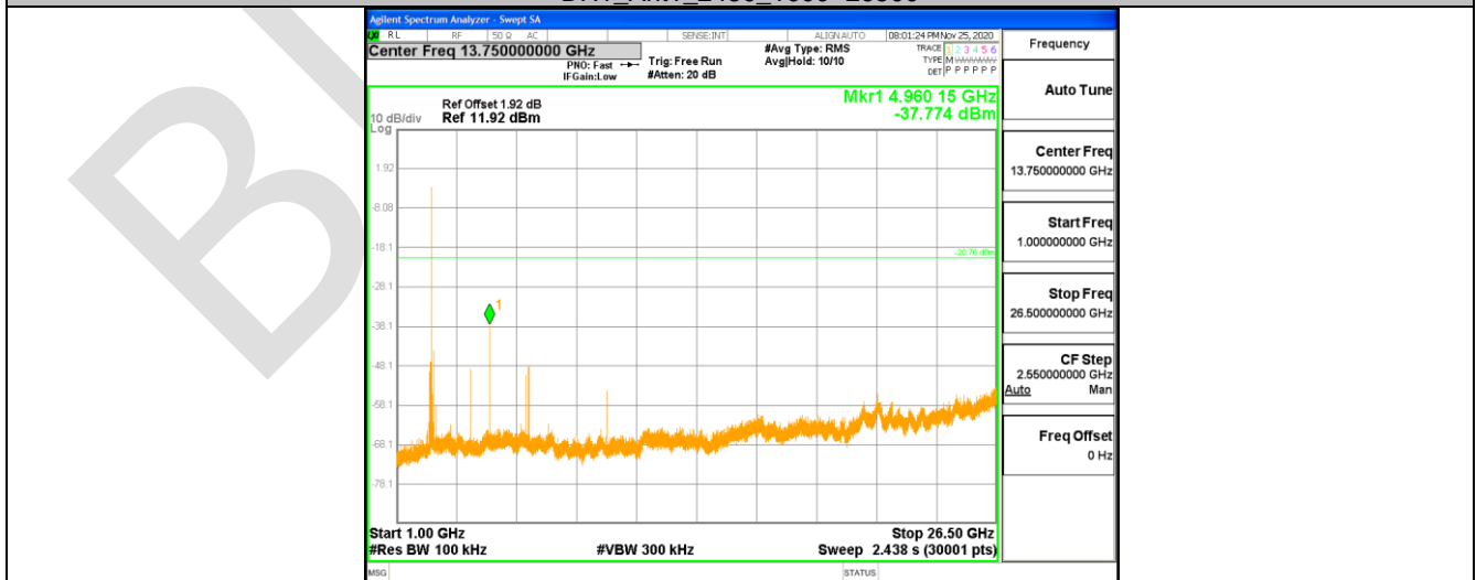
2DH1_Ant1_2402_0~Reference
