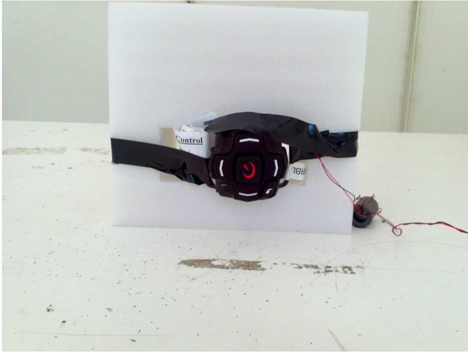
Picture 1: Radiated Emissions Test Setup at Open Area Test Site
