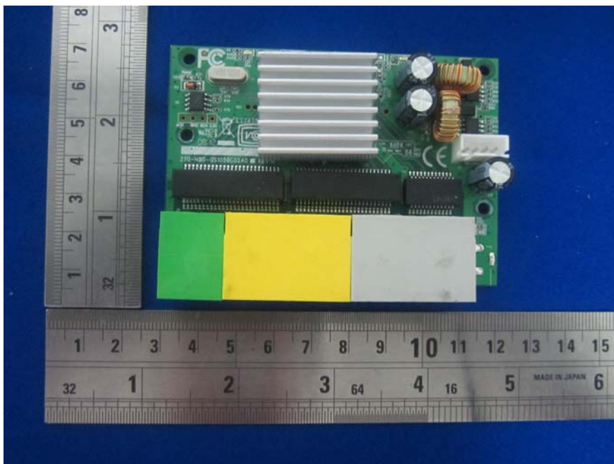
EUT – Main Board Top With Radiator View
