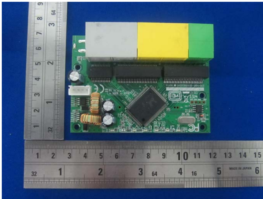
EUT –Main Board Top Without Radiator View
