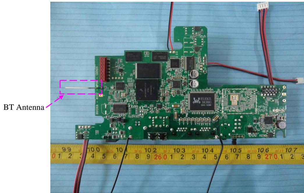
EUT – Main Board 2 Top View (Base)
