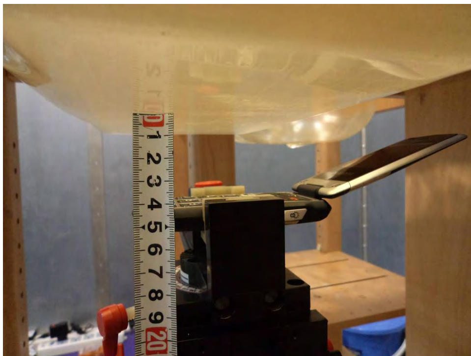
Head Setup Photo (The distance between flat phantom and EUT antenna location is 4.5cm )
