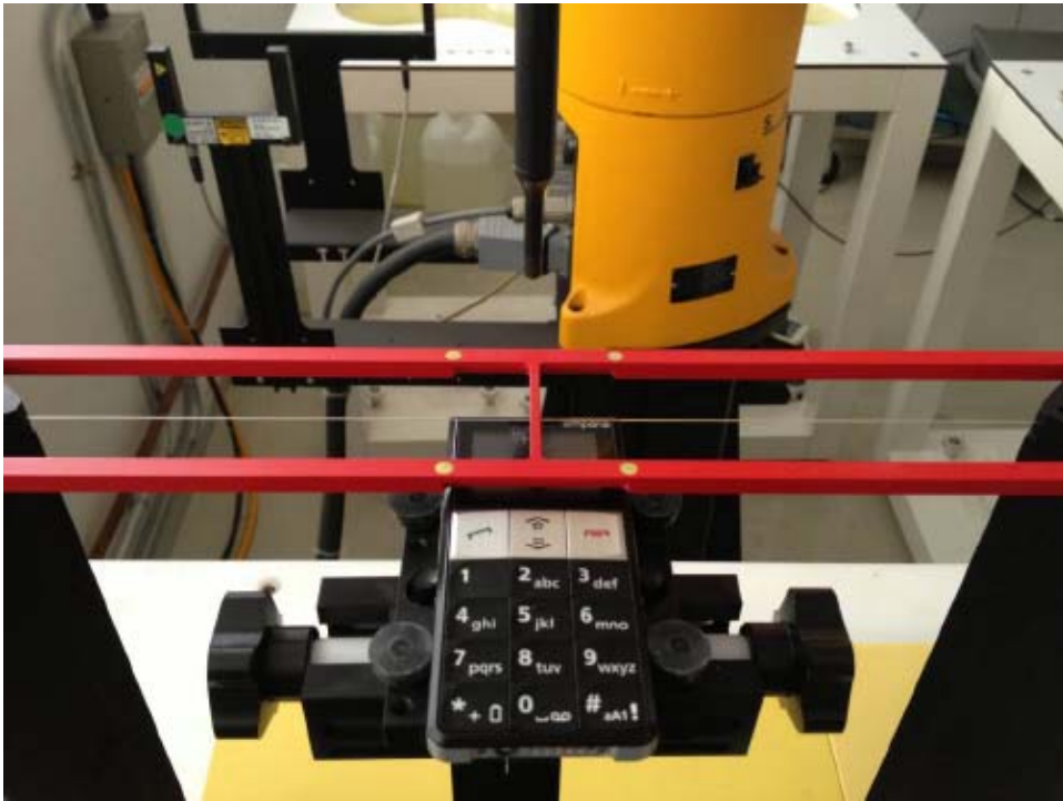
Photo 1: HAC RF Set-up
