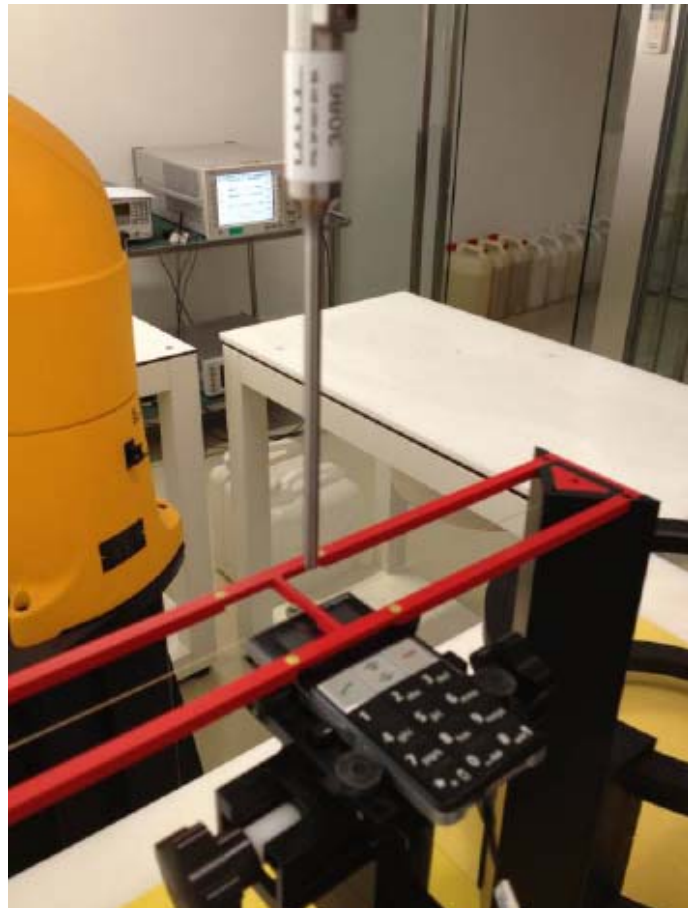
Photo 2: HAC T-Coil Set-up
