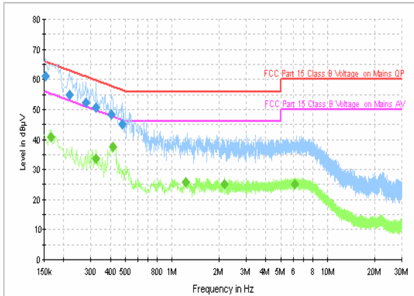
ESH2-Z5 Scan-FCC
