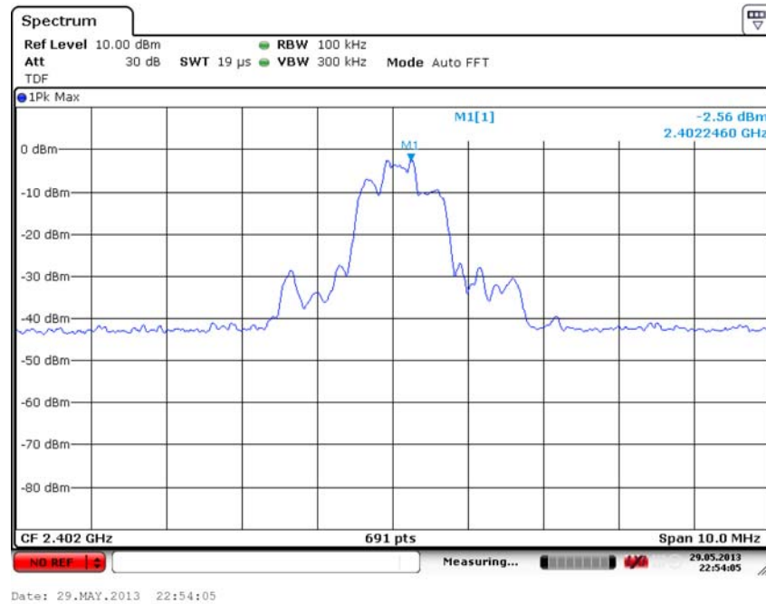
Fig. 25 Conducted Spurious Emission (8DPSK, Ch0, Center Frequency)
