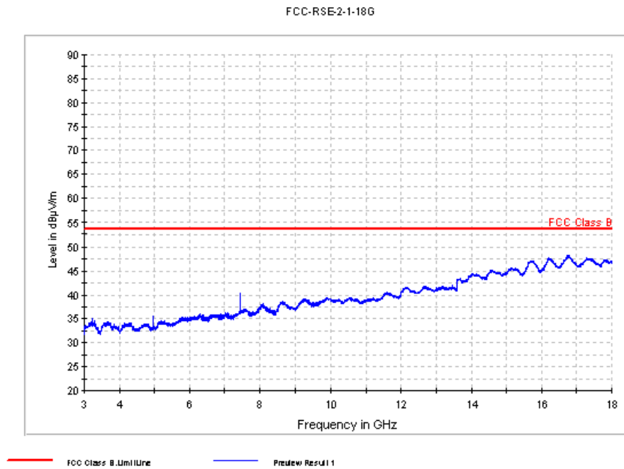
Fig. 43 Radiated Spurious Emission ( \pi/4 DQPSK, Ch78, 3 GHz ~18 GHz)
