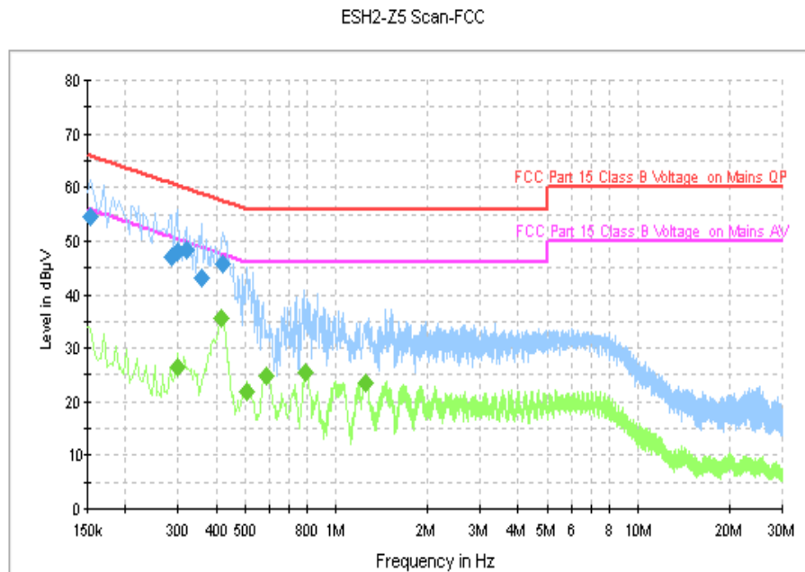
Fig. 70 AC Power line Conducted Emission ( \pi/4 DQPSK, Ch39)
