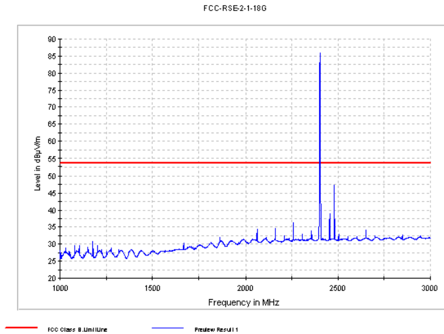
Fig. 45 Radiated Spurious Emission (8DPSK, Ch0, 1 GHz ~3 GHz)
