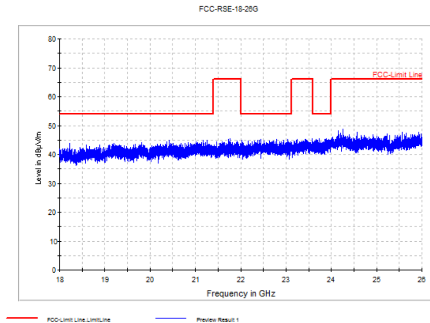
Fig. 50 Radiated Spurious Emission (All channel, 18 GHz ~26 GHz)
