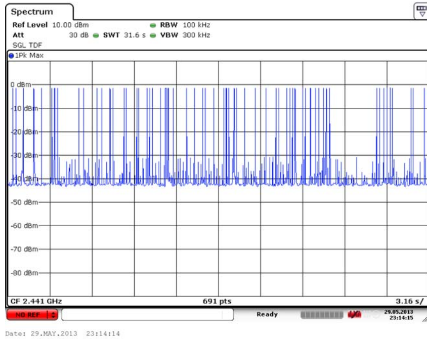
Fig. 55 Number of Transmissions (GFSK, Ch39)
