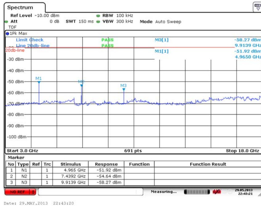
Fig. 18 Conducted Spurious Emission (GFSK, Ch78, 3GHz-18 GHz)
