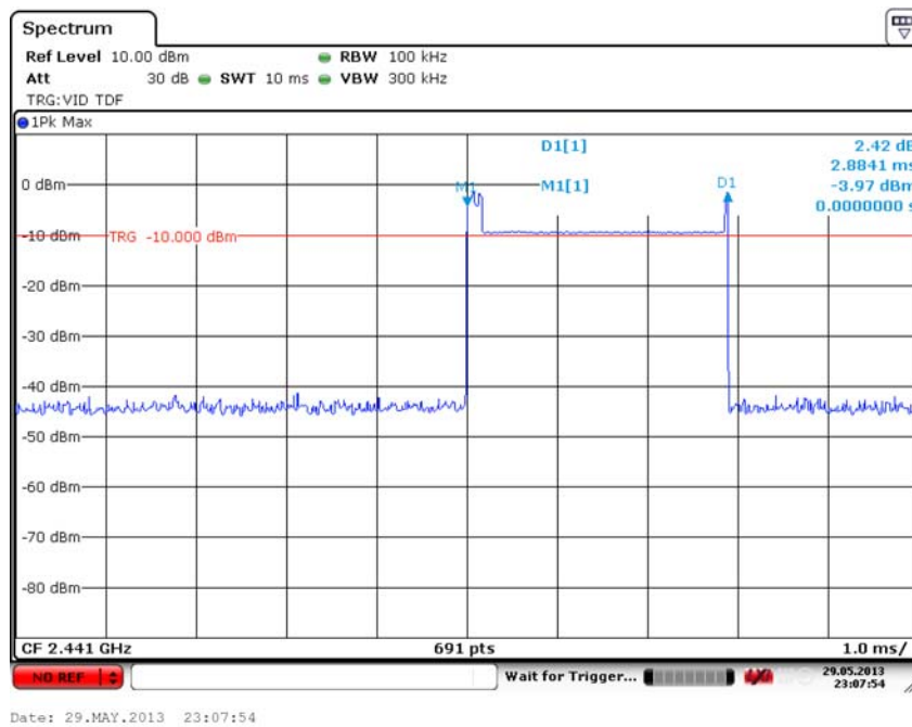
Fig. 54 Time of Occupancy(Dwell Time) (GFSK, Ch39)
