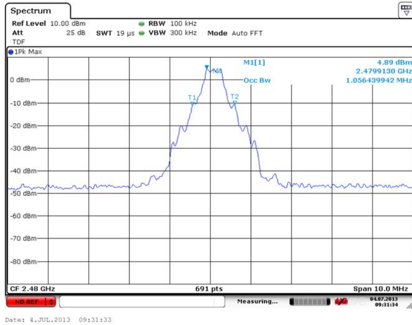
Fig. 74 Occupied Bandwidth (GFSK, Ch78)
