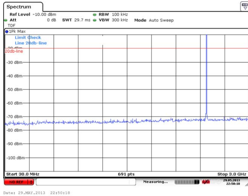
Fig. 23 Conducted Spurious Emission ( \pi/4 DQPSK, Ch78, 30 MHz-3 GHz)
