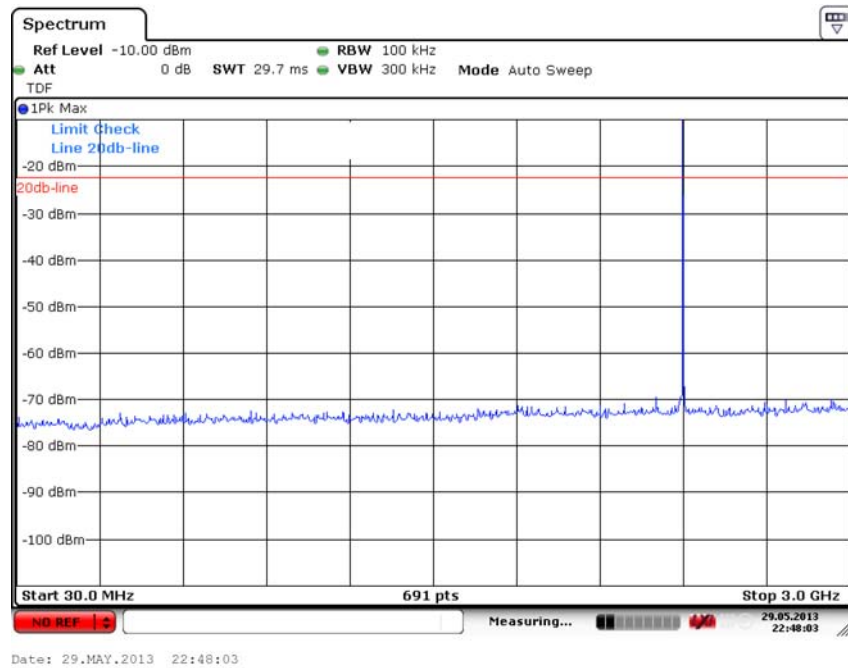
Fig. 20 Conducted Spurious Emission ( \pi/4 DQPSK, Ch0, 30 MHz-3 GHz)
