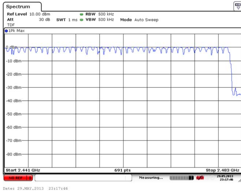
Fig. 63 Hopping channel ch39~78 ( \pi/4 DQPSK, Ch39)
