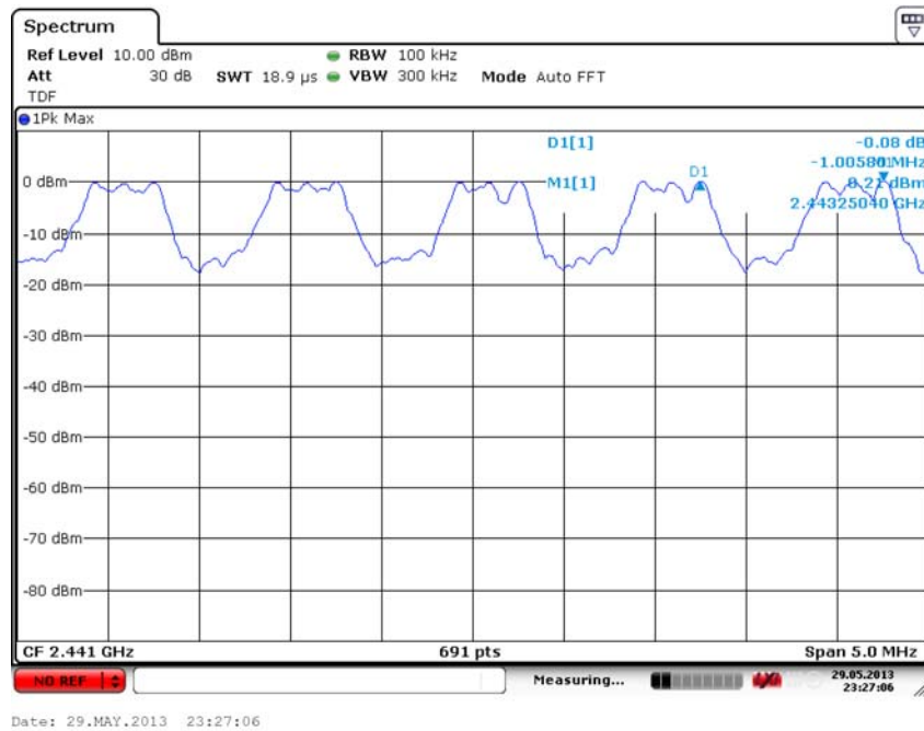
Fig. 66 Carrier Frequency Separation (GFSK, Ch39)
