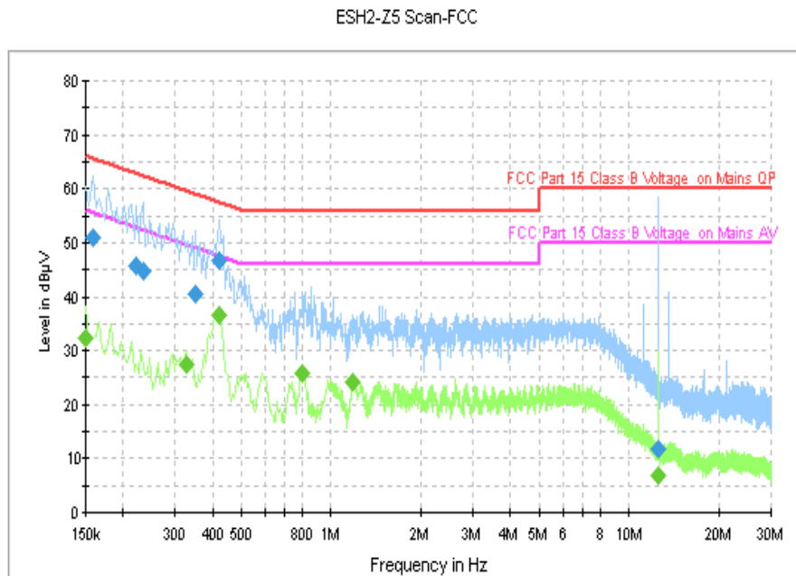
Fig. 69 AC Power line Conducted Emission (GFSK, Ch39)
