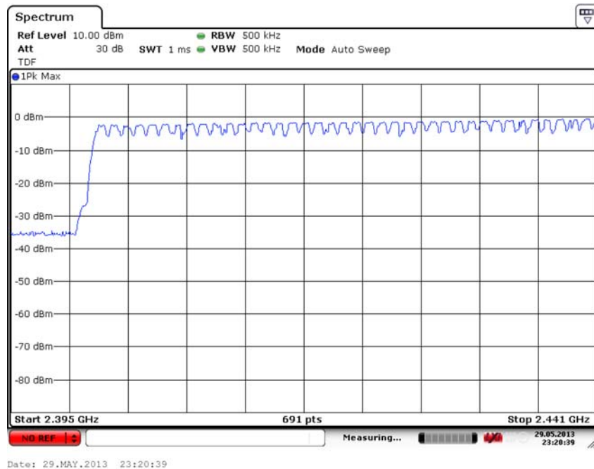
Fig. 64 Hopping channel ch0~39 (8DPSK, Ch39)
