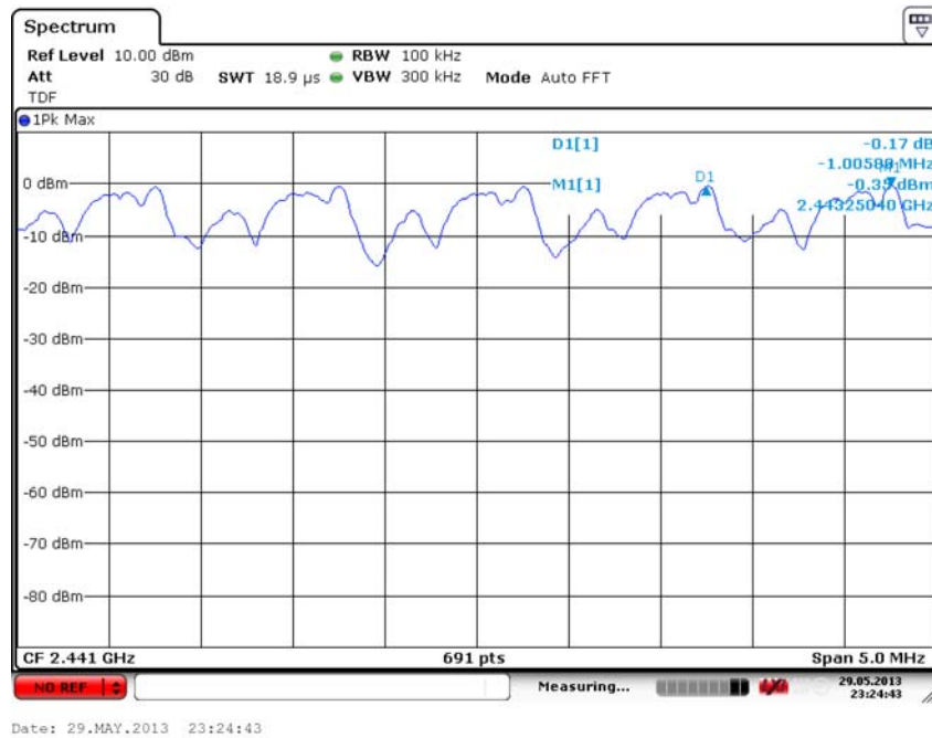
Fig. 68 Carrier Frequency Separation (8DPSK, Ch39)
