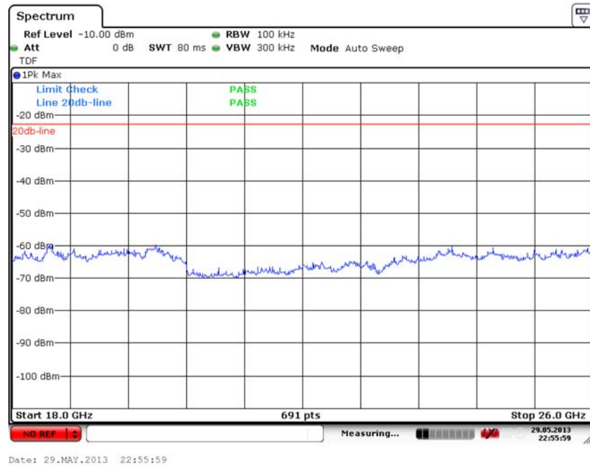
Fig. 31 Conducted Spurious Emission (All channel, 18 GHz-26 GHz)
