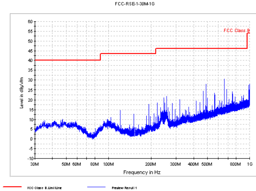
Fig. 41 Radiated Spurious Emission ( \pi/4 DQPSK, Ch78, 30 MHz ~1 GHz)
