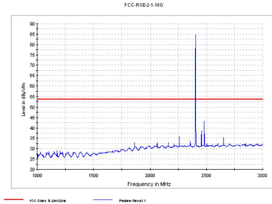
Fig. 33 Radiated Spurious Emission (GFSK, Ch0, 1 GHz ~3 GHz)
