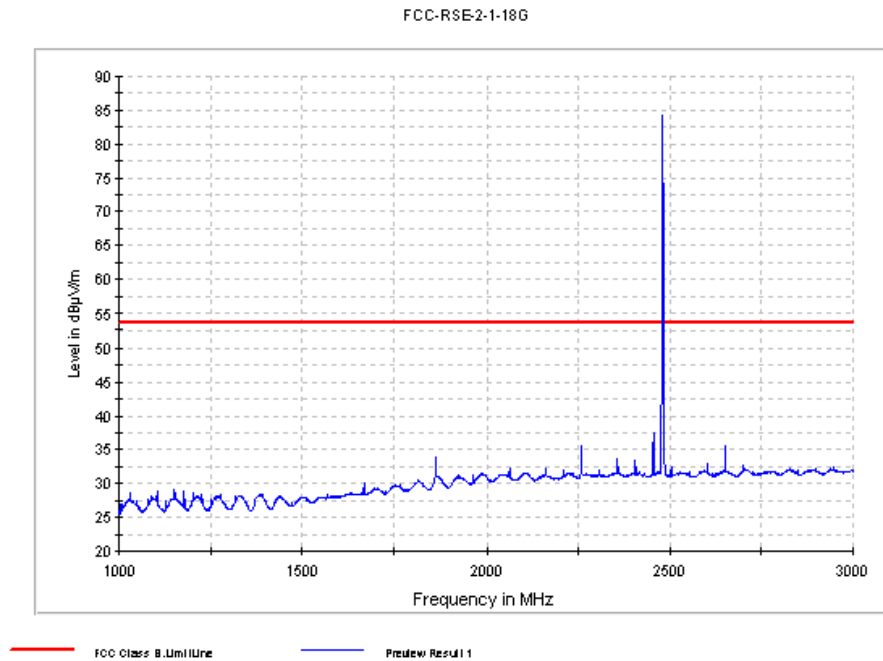
Fig. 42 Radiated Spurious Emission ( \pi/4 DQPSK, Ch78, 1 GHz ~3 GHz)
