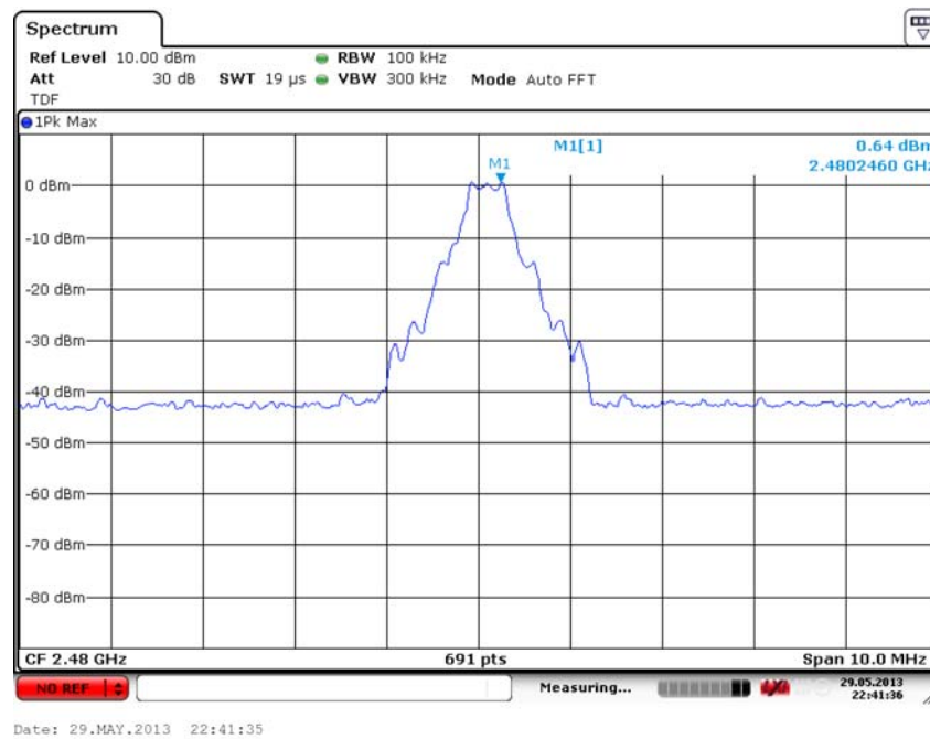
Fig. 16 Conducted Spurious Emission (GFSK, Ch78, Center Frequency)
