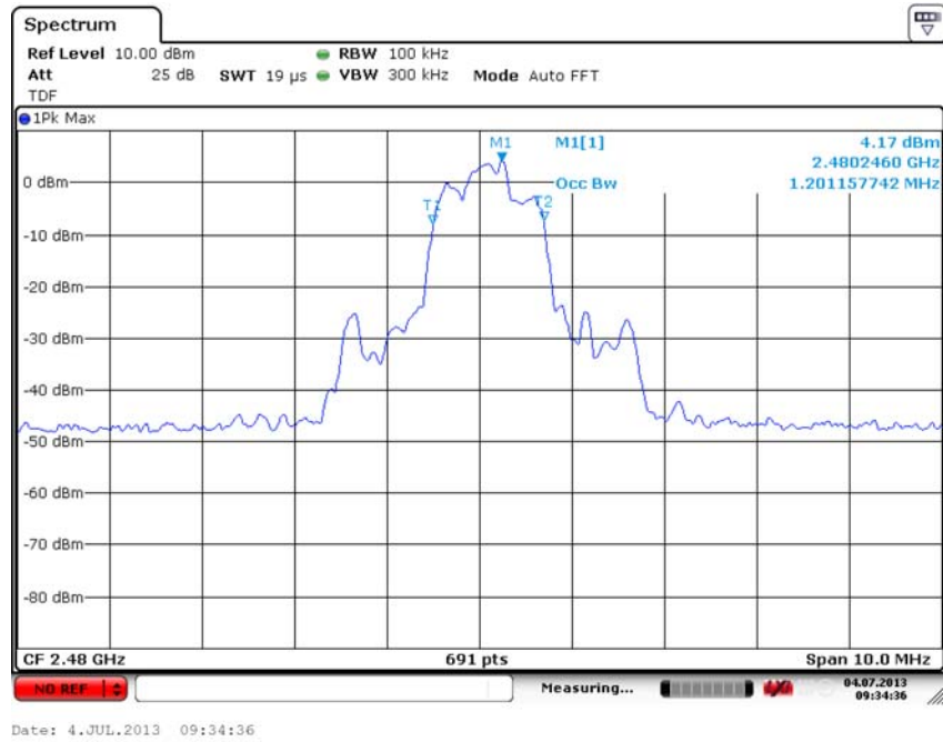
Fig. 80 Occupied Bandwidth (8DPSK, Ch78)
