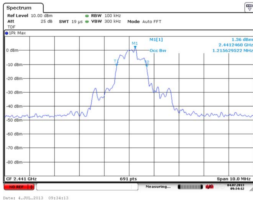
Fig. 79 Occupied Bandwidth (8DPSK, Ch39)
