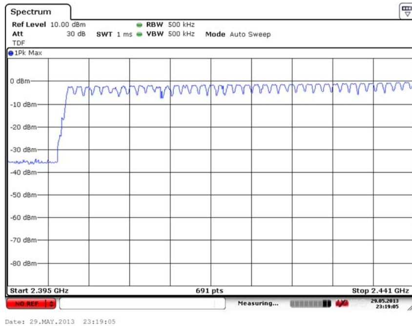
Fig. 62 Hopping channel ch0~39 ( \pi/4 DQPSK, Ch39)
