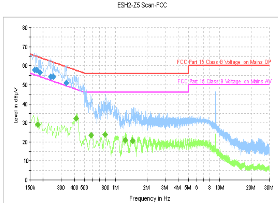
Fig. 71 AC Power line Conducted Emission (8DPSK, Ch39)
