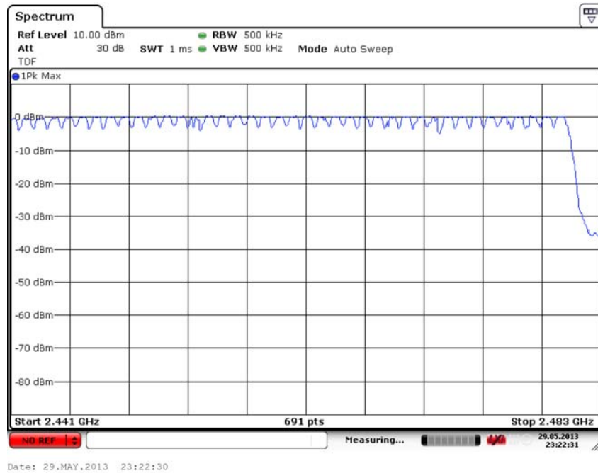
Fig. 65 Hopping channel ch39~78 (8DPSK, Ch39)
