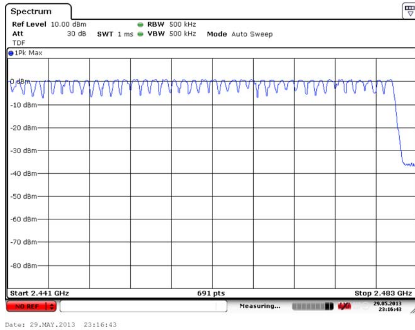
Fig. 61 Hopping channel ch39~78 (GFSK, Ch39)
