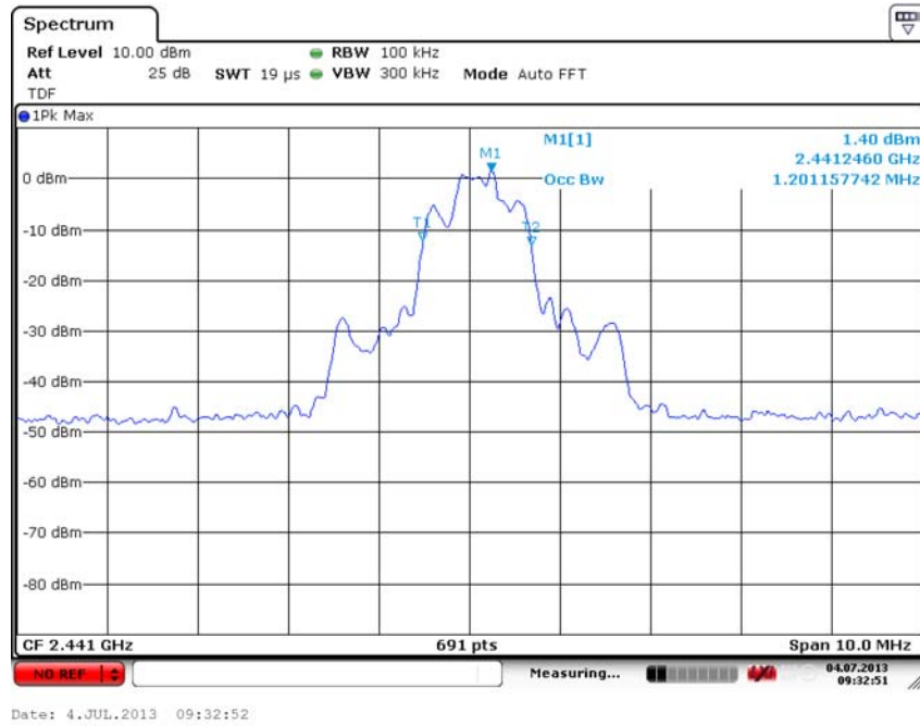
Fig. 76 Occupied Bandwidth ( \pi/4 DQPSK, Ch39)
