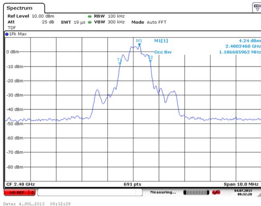
Fig. 77 Occupied Bandwidth ( \pi/4 DQPSK, Ch78)
