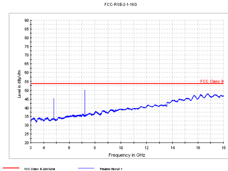
Fig. 46 Radiated Spurious Emission (8DPSK, Ch0, 3 GHz ~18 GHz)
