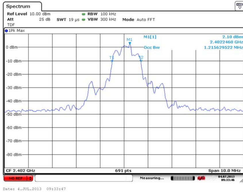
Fig. 78 Occupied Bandwidth (8DPSK, Ch0)
