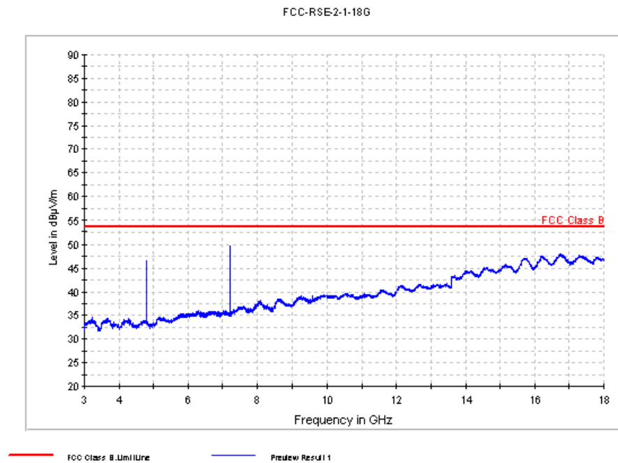
Fig. 34 Radiated Spurious Emission (GFSK, Ch0, 3 GHz ~18 GHz)
