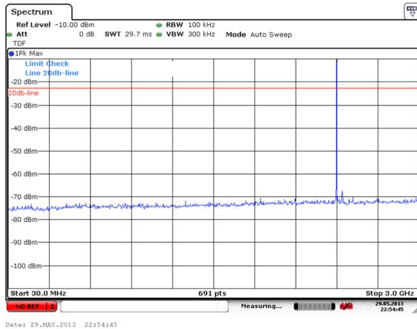
Fig. 26 Conducted Spurious Emission (8DPSK, Ch0, 30 MHz-3 GHz)
