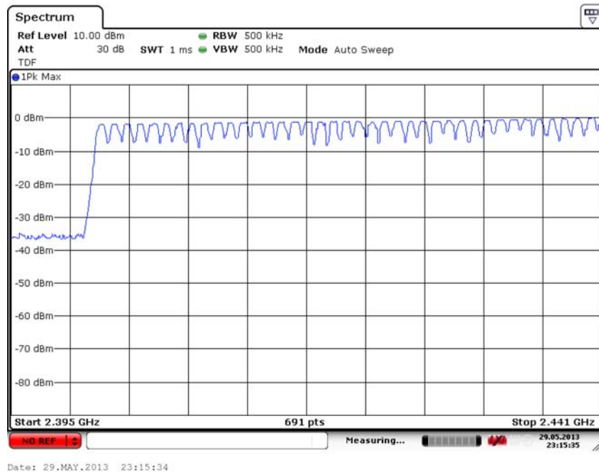
Fig. 60 Hopping channel ch0~39 (GFSK, Ch39)
