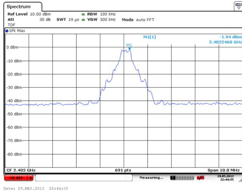
Fig. 13 Conducted Spurious Emission (GFSK, Ch0, Center Frequency)
