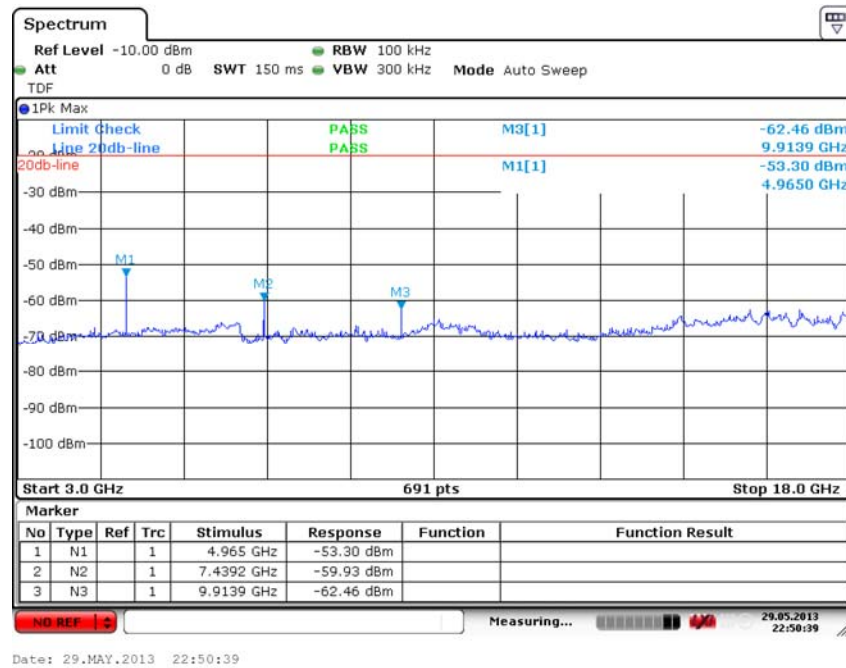
Fig. 24 Conducted Spurious Emission ( \pi/4 DQPSK, Ch78, 3GHz-18 GHz)
