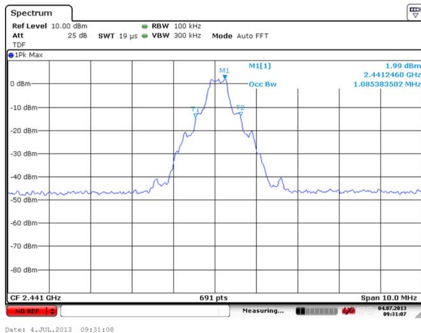
Fig. 73 Occupied Bandwidth (GFSK, Ch39)
