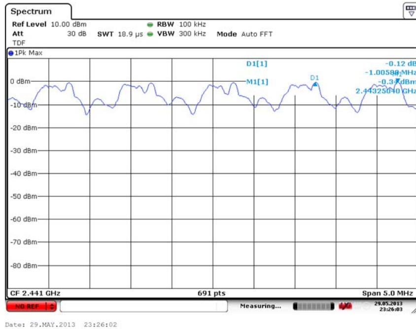
Fig. 67 Carrier Frequency Separation ( \pi/4 DQPSK, Ch39)
