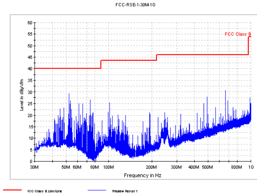
Fig. 35 Radiated Spurious Emission (GFSK, Ch78, 30 MHz ~1 GHz)
