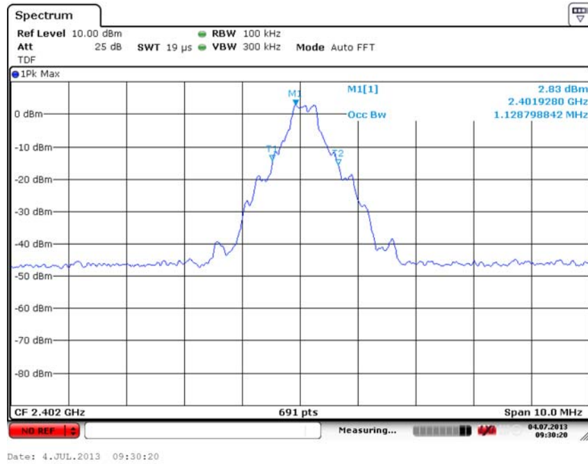
Fig. 72 Occupied Bandwidth (GFSK, Ch0)
