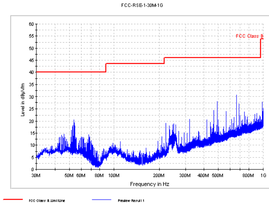
Fig. 44 Radiated Spurious Emission (8DPSK, Ch0, 30 MHz ~1 GHz)
