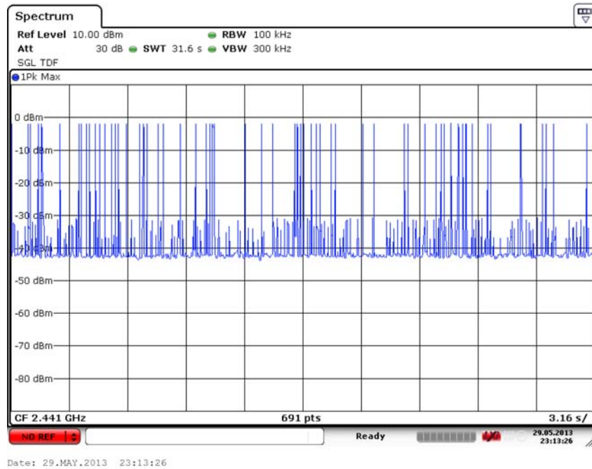
Fig. 57 Number of Transmissions ( \pi/4 DQPSK, Ch39)
