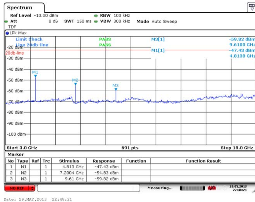
Fig. 21 Conducted Spurious Emission ( \pi/4 DQPSK, Ch0, 3GHz-18 GHz)
