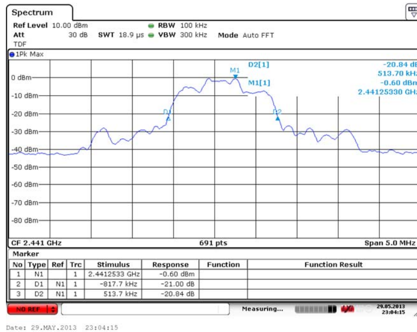
Fig. 53 Occupied 20dB Bandwidth (8DPSK, Ch 39)
