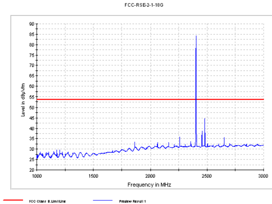
Fig. 39 Radiated Spurious Emission ( \pi/4 DQPSK, Ch0, 1 GHz ~3 GHz)
