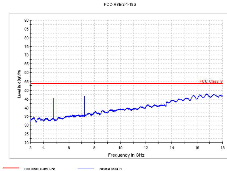
Fig. 40 Radiated Spurious Emission ( \pi/4 DQPSK, Ch0, 3 GHz ~18 GHz)
