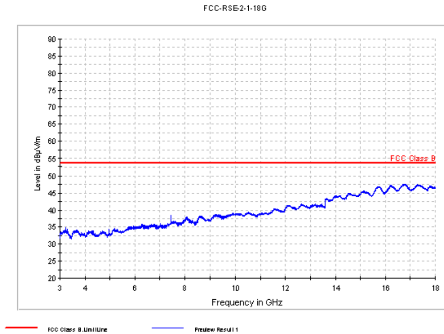
Fig. 49 Radiated Spurious Emission (8DPSK, Ch78, 3 GHz ~18 GHz)
