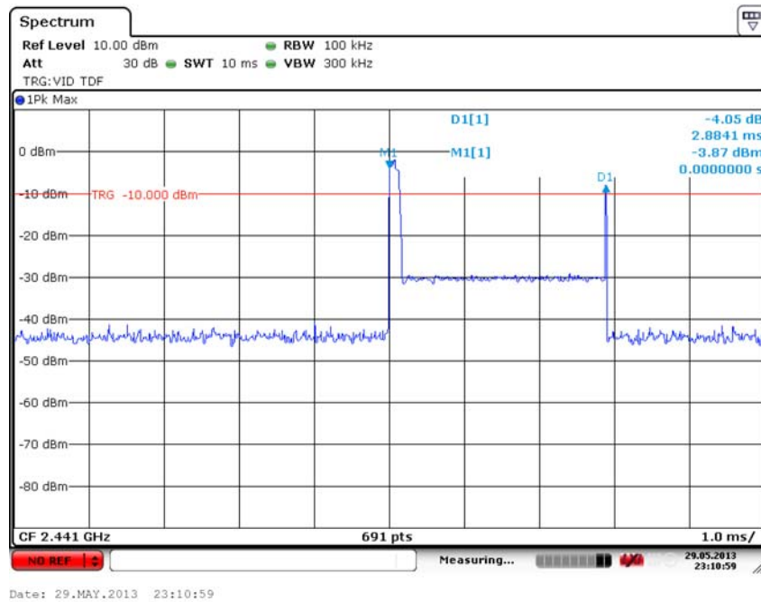
Fig. 58 Time of Occupancy(Dwell Time) (8DPSK, Ch39)
