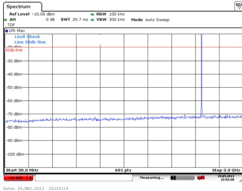
Fig. 29 Conducted Spurious Emission (8DPSK, Ch78, 30 MHz-3 GHz)
