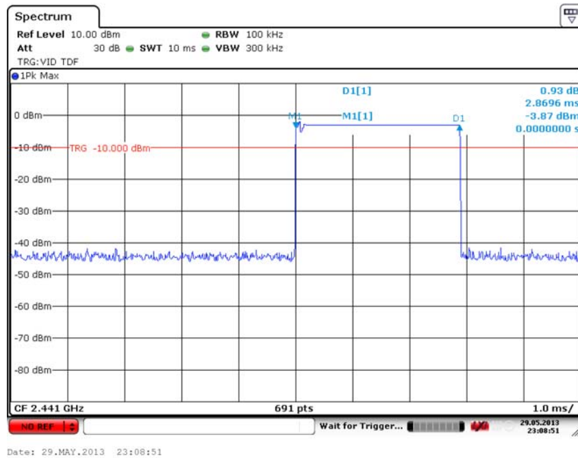
Fig. 56 Time of Occupancy(Dwell Time) ( \pi/4 DQPSK, Ch39)
