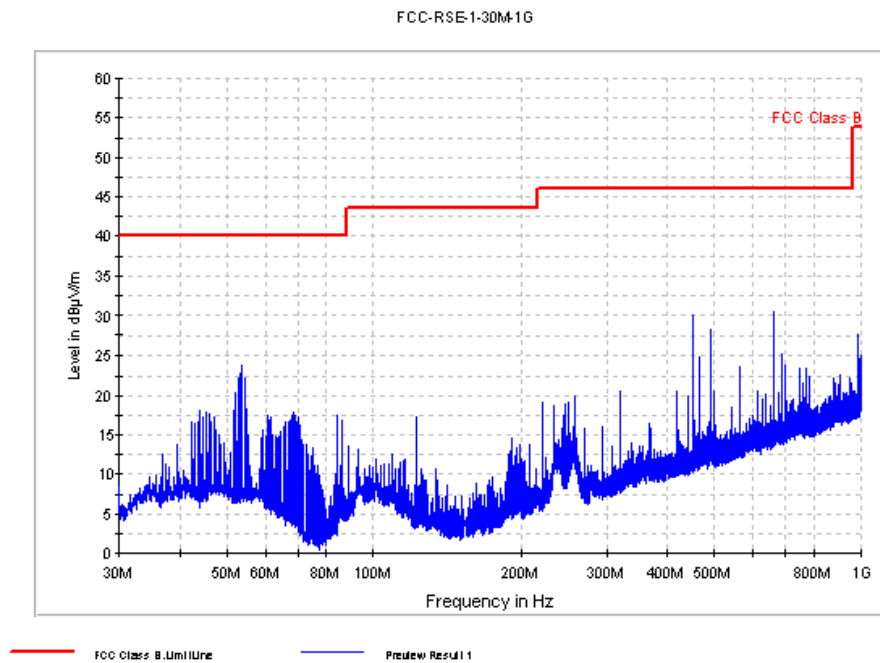
Fig. 38 Radiated Spurious Emission ( \pi/4 DQPSK, Ch0, 30 MHz ~1 GHz)
