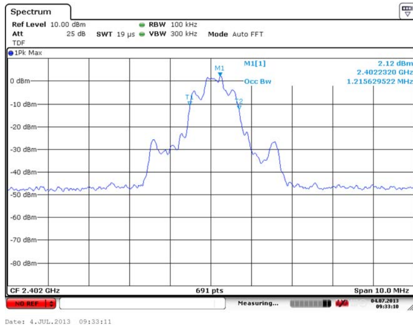
Fig. 75 Occupied Bandwidth ( \pi/4 DQPSK, Ch0)
