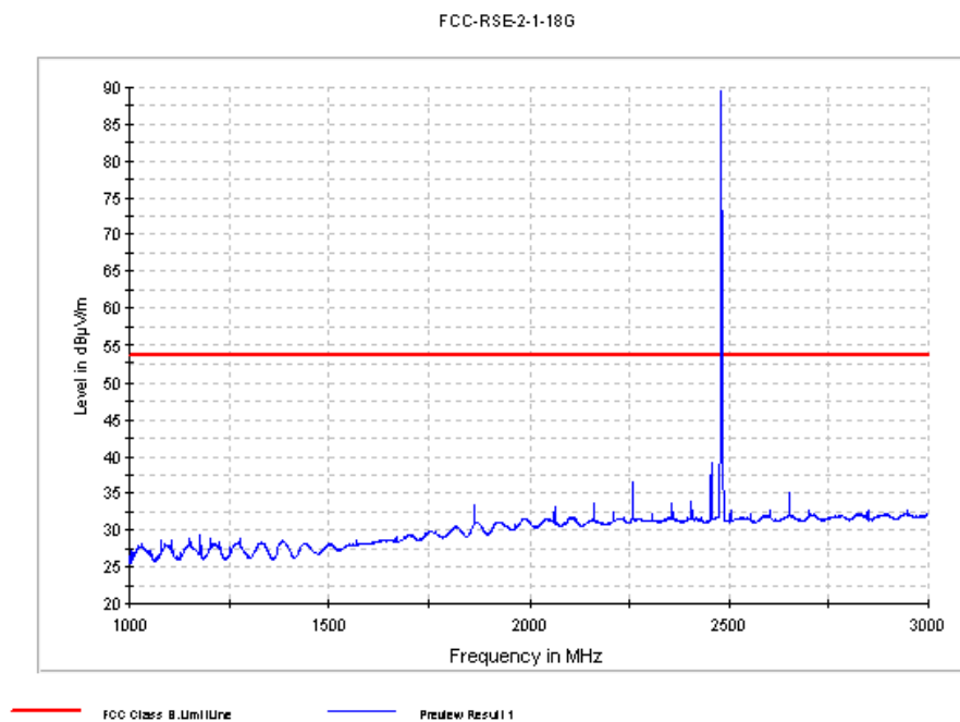
Fig. 36 Radiated Spurious Emission (GFSK, Ch78, 1 GHz ~3 GHz)
