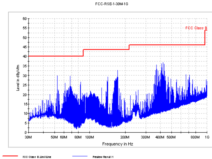
Fig. 47 Radiated Spurious Emission (8DPSK, Ch78, 30 MHz ~1 GHz)
