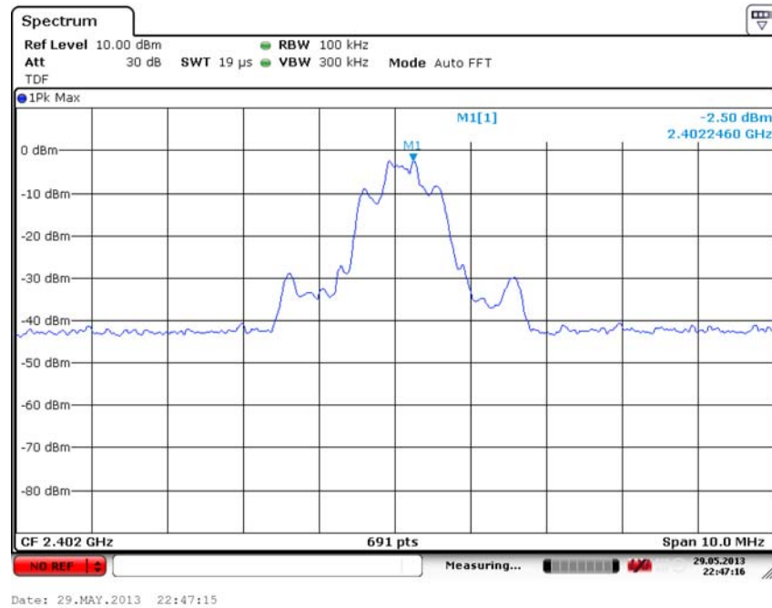
Fig. 19 Conducted Spurious Emission ( \pi/4 DQPSK, Ch0, Center Frequency)
