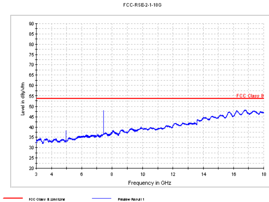
Fig. 37 Radiated Spurious Emission (GFSK, Ch78, 3 GHz ~18 GHz)
