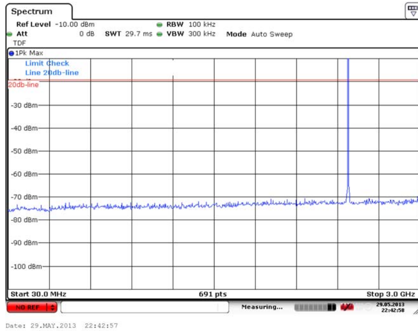
Fig. 17 Conducted Spurious Emission (GFSK, Ch78, 30 MHz-3 GHz)
