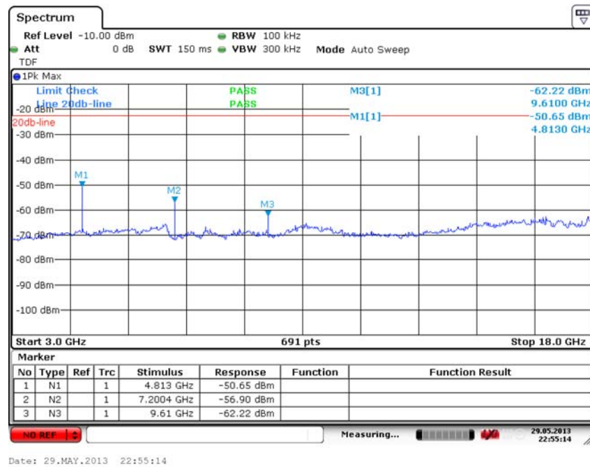
Fig. 27 Conducted Spurious Emission (8DPSK, Ch0, 3GHz-18 GHz)
