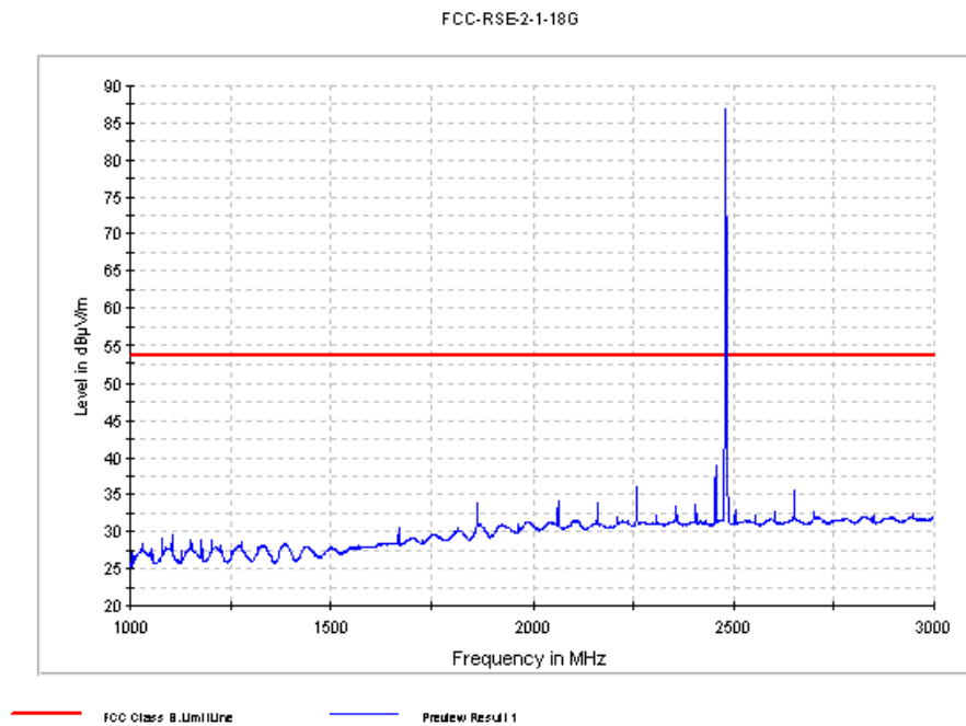
Fig. 48 Radiated Spurious Emission (8DPSK, Ch78, 1 GHz ~3 GHz)
