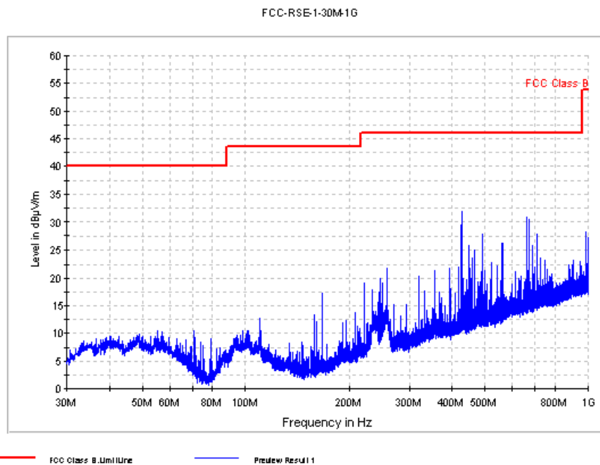
Fig. 32 Radiated Spurious Emission (GFSK, Ch0, 30 MHz ~1 GHz)
