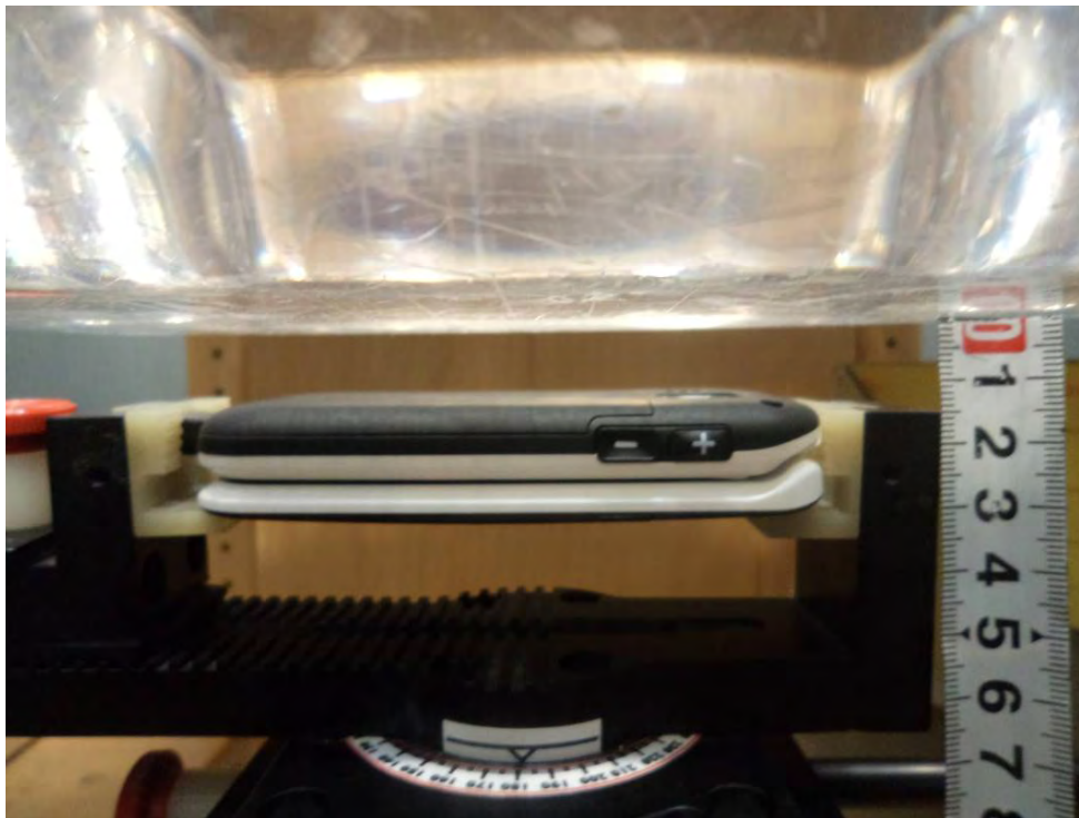
Body-worn Back Setup with headset Photo (GSM)
