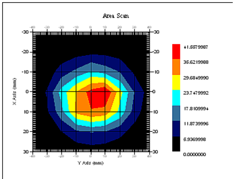
1900 MHz System Validation with Body Tissue
