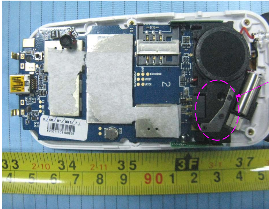
EUT – Main Board Cover off View
