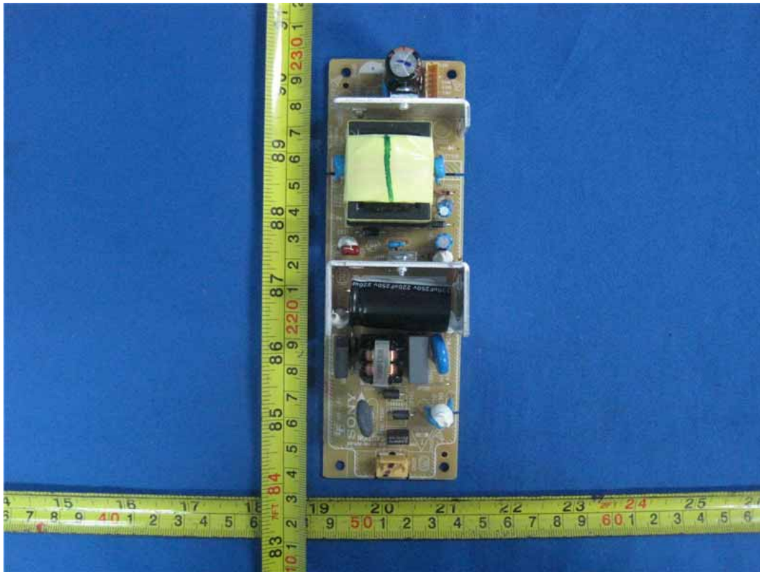
Figure 13 Frontside of the Power Board
