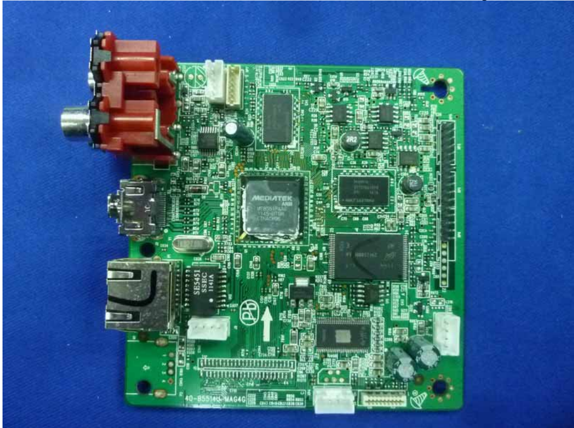
Figure 15 (KEM-470AAB)Component Side of the PCB
