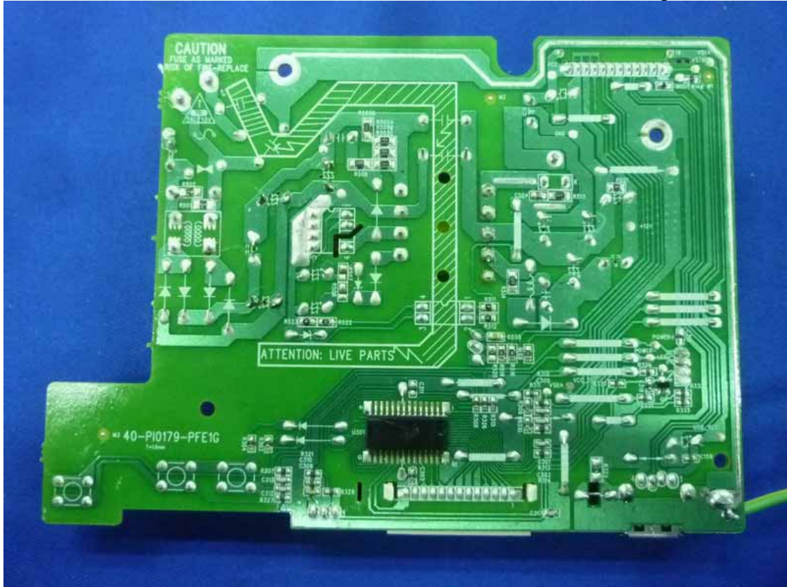
Figure 13 (KEM-470AAB)Component Side of the PCB
