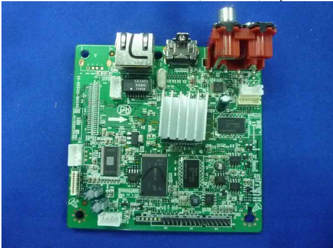
Figure 14 (KEM-470AAB)Component Side of the PCB
