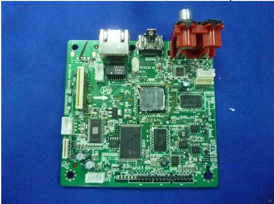
Figure 22 (KEM480AAA)Component Side of the PCB
