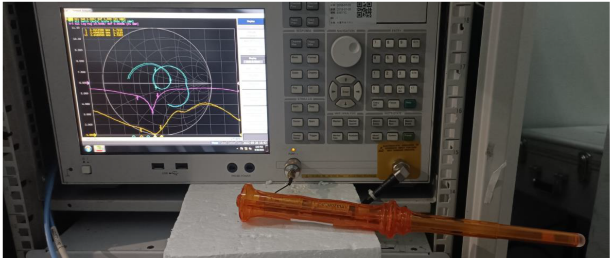
S11 test
