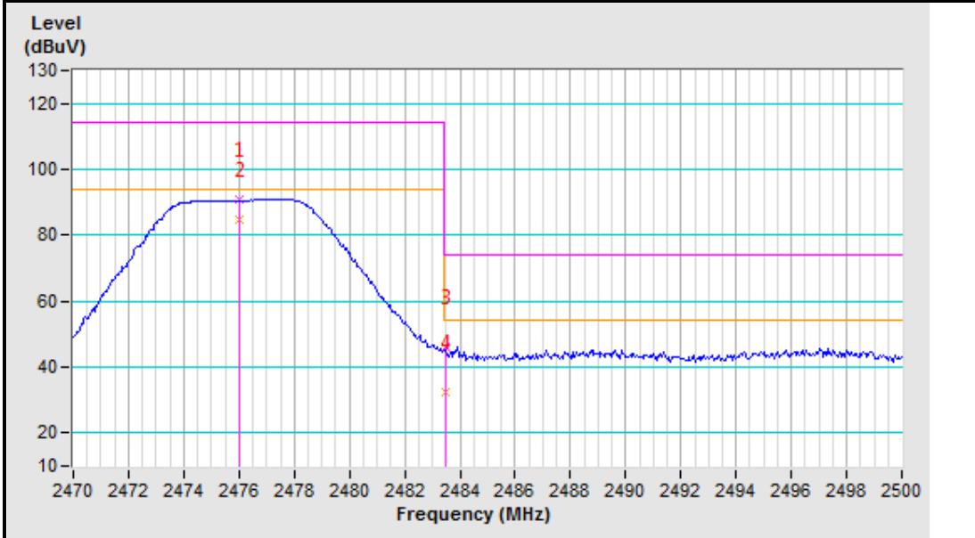
2483.5MHz Vertical
