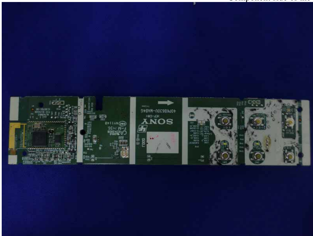
Figure 8 Component side of the Main Board
