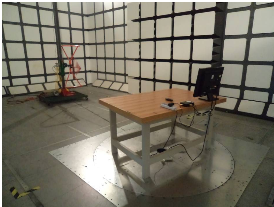
Radiated Emission - Rear View (30 MHz-1000 MHz)
