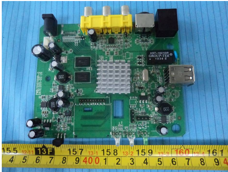
EUT – Main Board without RF ModuleView
