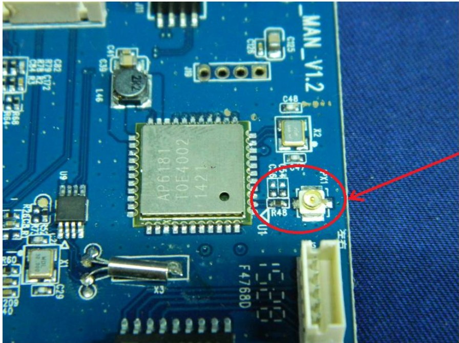
wifi Antenna
