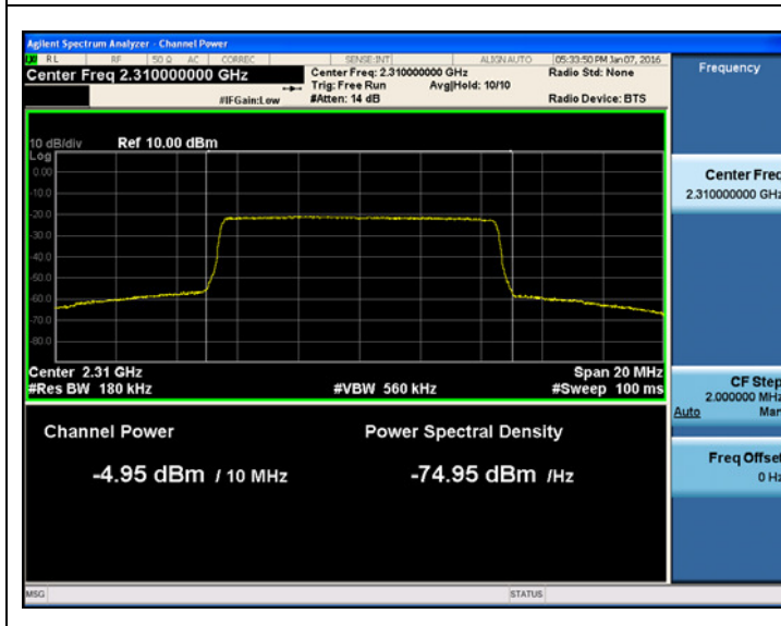
[WCS AGC threshold Uplink LTE 10MHz]
