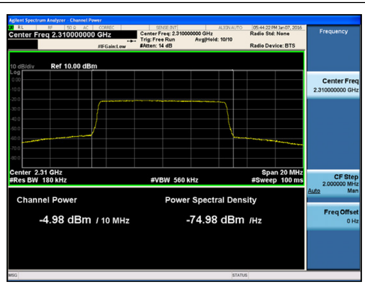
[WCS +3dB above the threshold Uplink LTE 10MHz]
