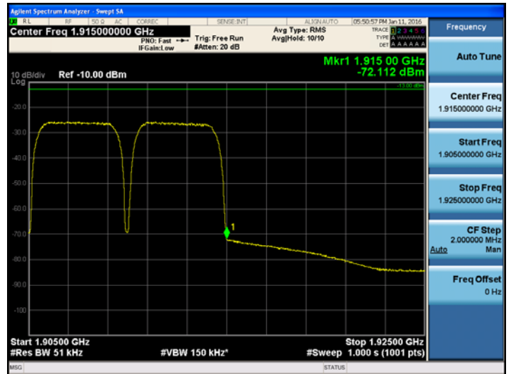
[PCS 1900 CDMA Uplink High]
