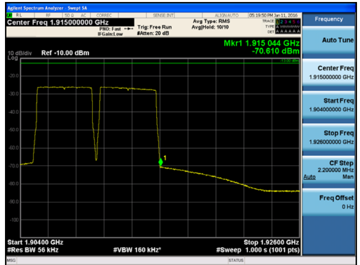
[PCS 1900 LTE 10MHz Uplink High]
