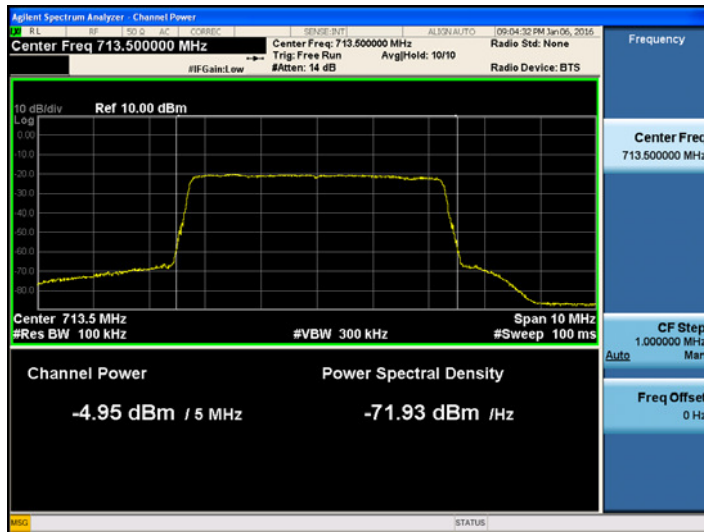
[700 Band AGC threshold Uplink LTE 5 MHz High]
