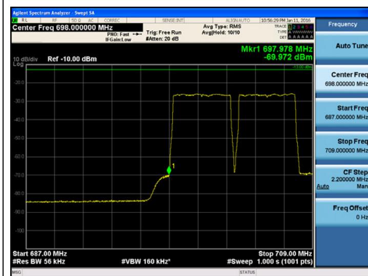
[700 Band LTE 5 MHz Uplink Low]
