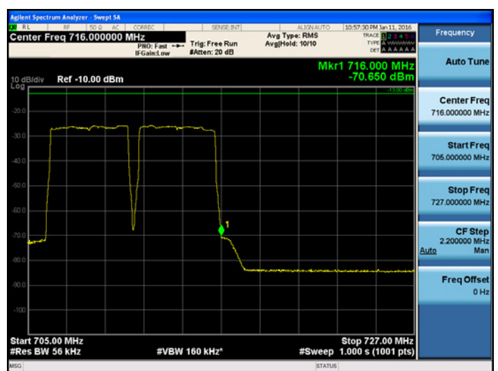
[700 Band LTE 5 MHz Uplink High]
