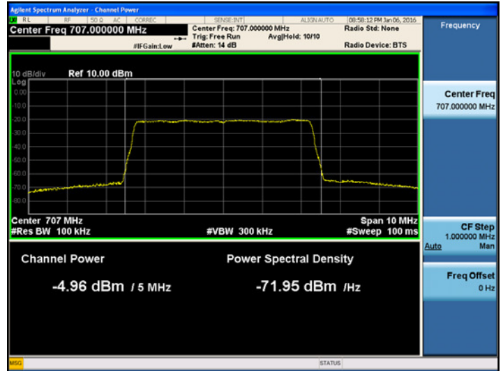
[700 Band AGC threshold Uplink LTE 5 MHz Mid]
