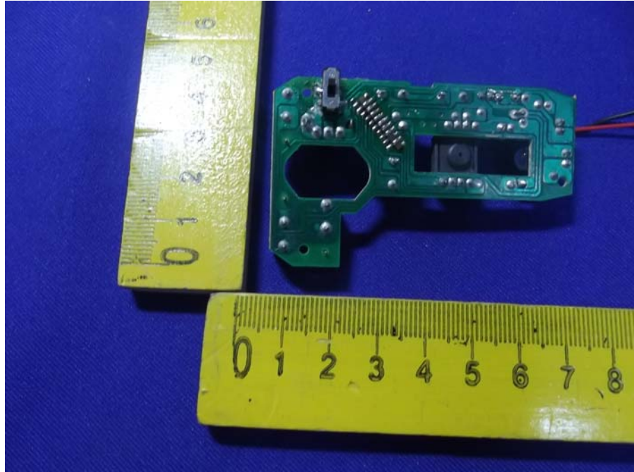
Figure 4 PCB of the EUT View
