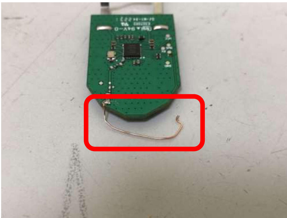
Detail of Antenna
