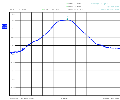
Figure 8.3-1: Output power on low channel
