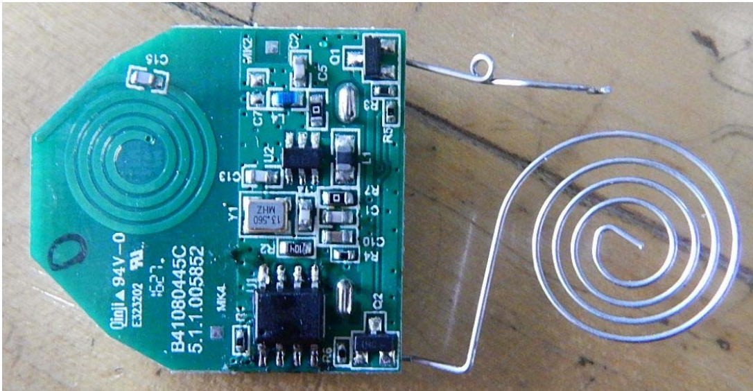
Figure 1-2: Main PCB bottom view
