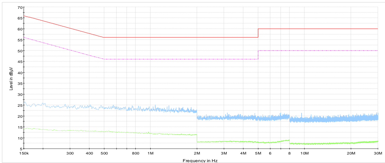
Conducted emissions on neutral line — CISPR 22 Mains QP Class B - - - CISPR 22 Mains AV Class B Preview Result 1-PK+ Preview Result 2-AVG
