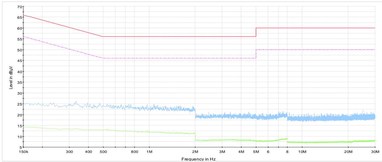
Conducted emissions on phase line — CISPR 22 Mains QP Class B - - - CISPR 22 Mains AV Class B Preview Result 1-PK+ Preview Result 2-AVG
