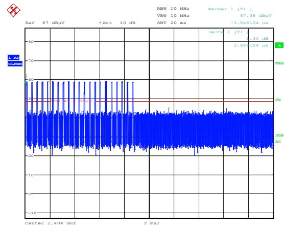
Plot 8.2-2: Number of pulses
