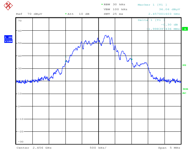
Plot 8.2-2: 20 dB bandwidth Mid channel
