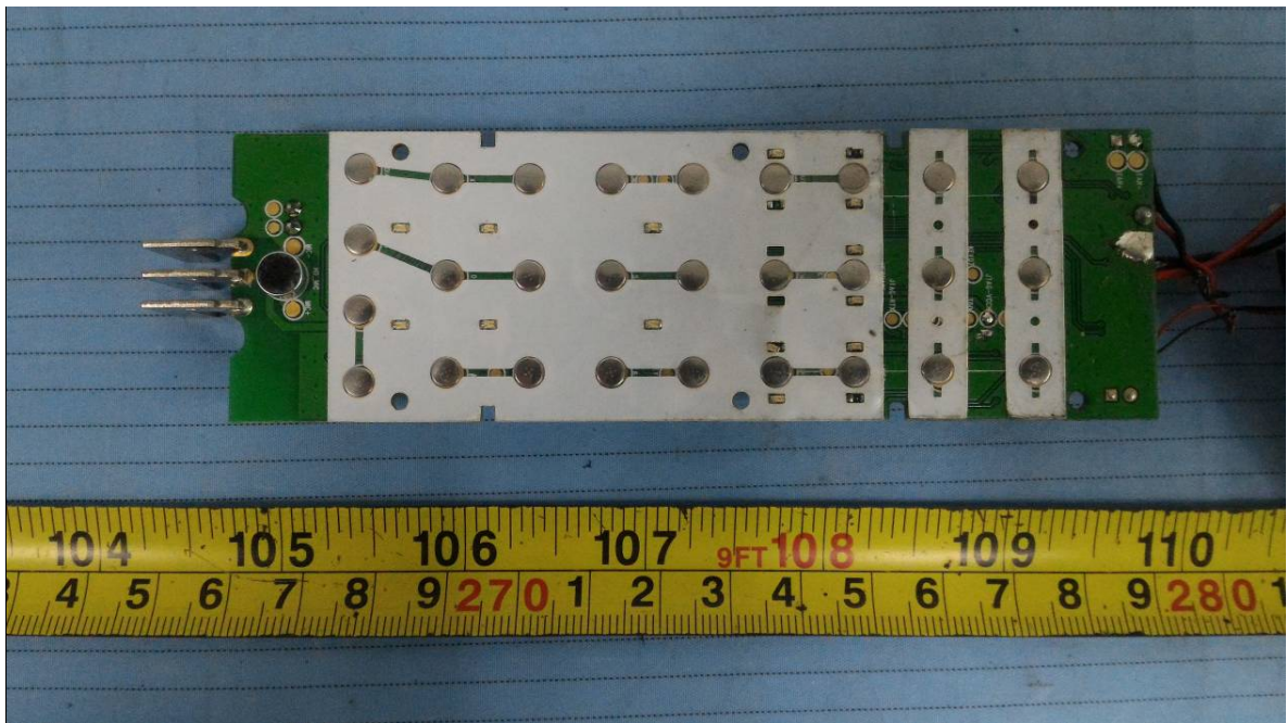
EUT – Main Board 1 Bottom View (Model: M203106 & M20356 (with 6 memory keys))
