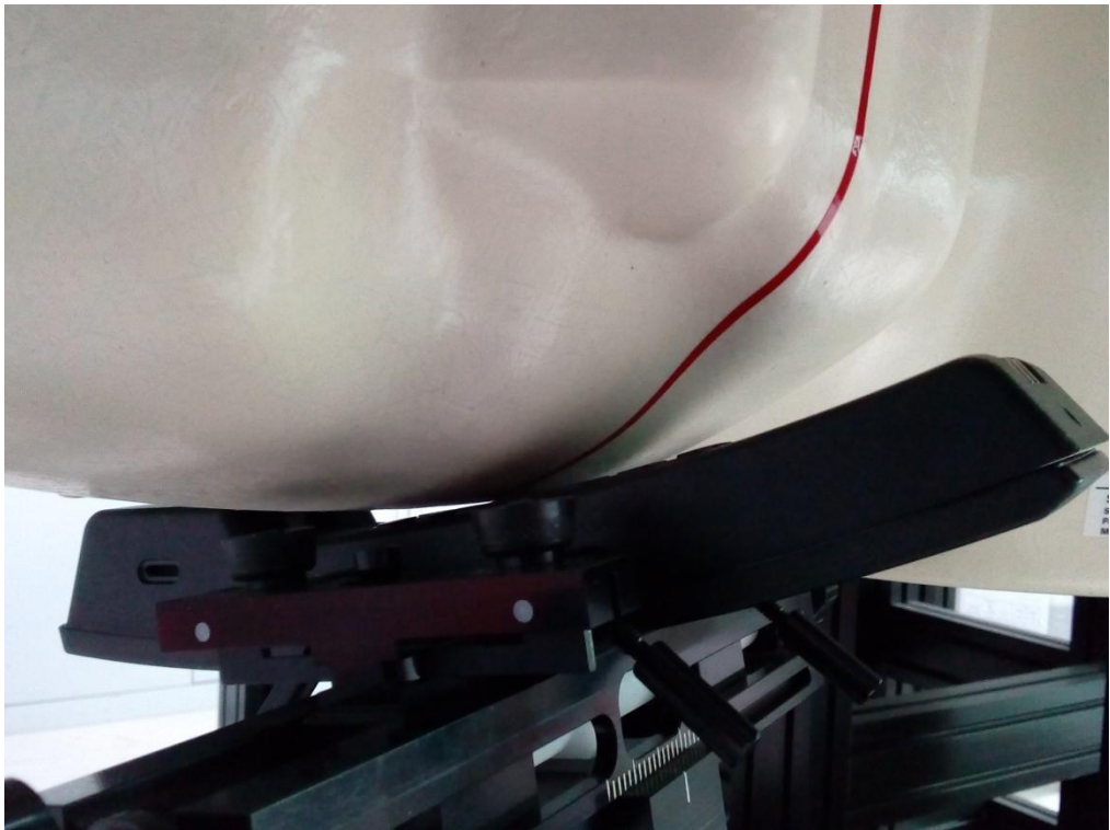
Head Right Cheek Setup Photo
