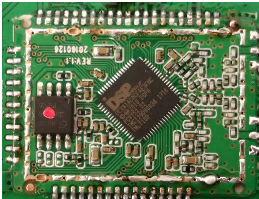
EUT – PCB-4 Module View
