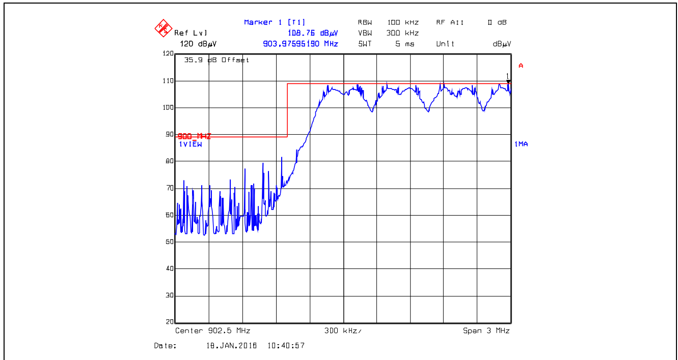
Plot 5.5.4.2.12. Band-Edge RF Radiated Emissions at 3 m, Vertical Polarization Pseudorandom Hopping Mode, Low End of Frequency Band, 902.5 MHz, GFSK, Data Rate at 400 kbps
