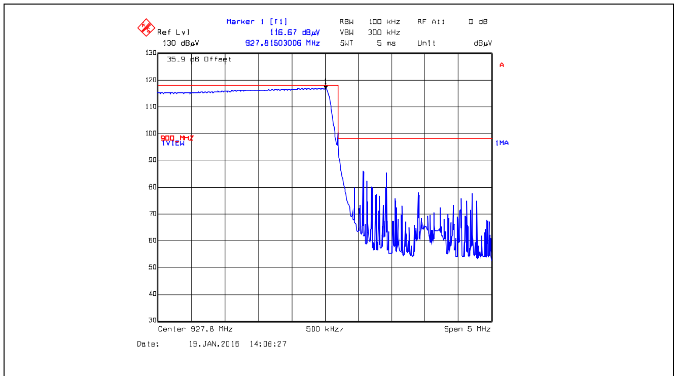
Plot 5.5.4.4.2.6. Band-Edge RF Radiated Emissions at 3 m, Horizontal Polarization Pseudorandom Hopping Mode, High End of Frequency Band, 927.8 MHz, FSK, Data rate at 10 Kbps
