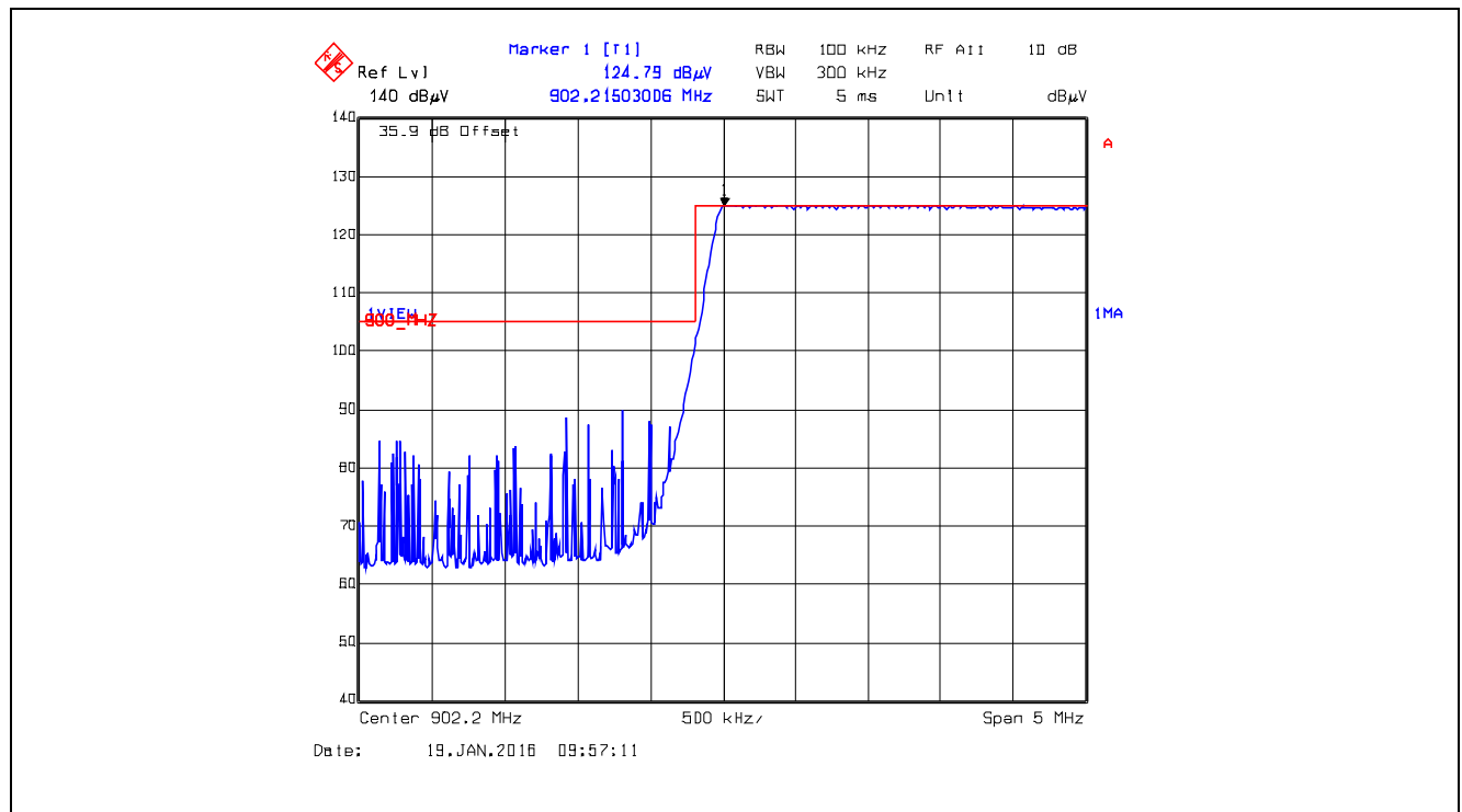
Plot 5.5.4.5.2.4. Band-Edge RF Radiated Emissions at 3 m, Vertical Polarization Pseudorandom Hopping Mode, Low End of Frequency Band, 902.2 MHz FSK, Data rate at 10 Kbps
