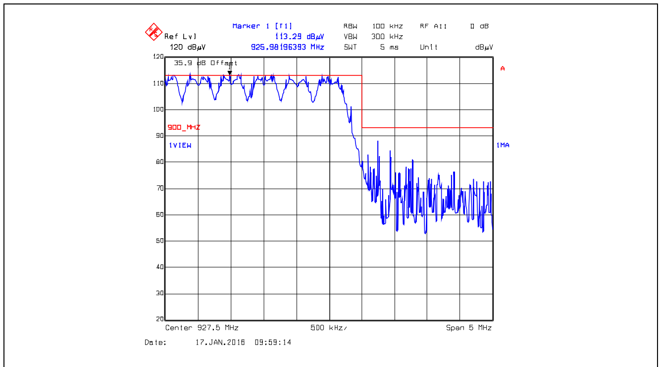
Plot 5.5.4.1.2.14. Band-Edge RF Radiated Emissions at 3 m, Horizontal Polarization Pseudorandom Hopping Mode, High End of Frequency Band, 927.5 MHz, GFSK, Data Rate at 400 kbps
