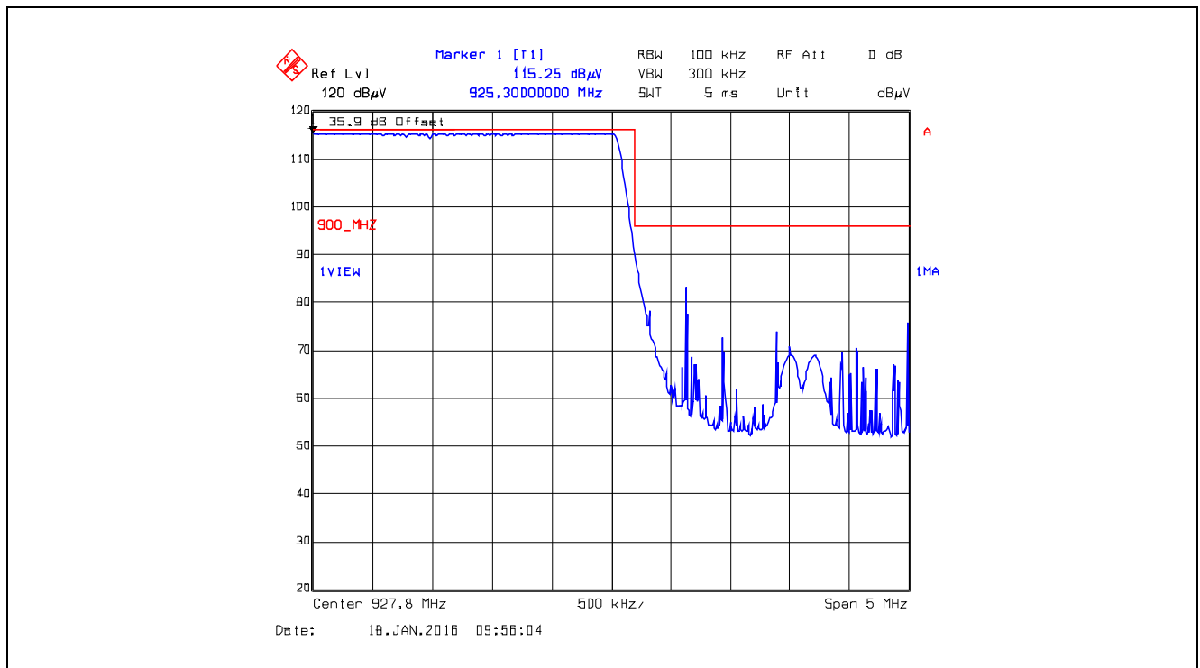
Plot 5.5.4.2.2.6. Band-Edge RF Radiated Emissions at 3 m, Horizontal Polarization Pseudorandom Hopping Mode, High End of Frequency Band, 927.8 MHz, FSK, Data rate at 10 Kbps
