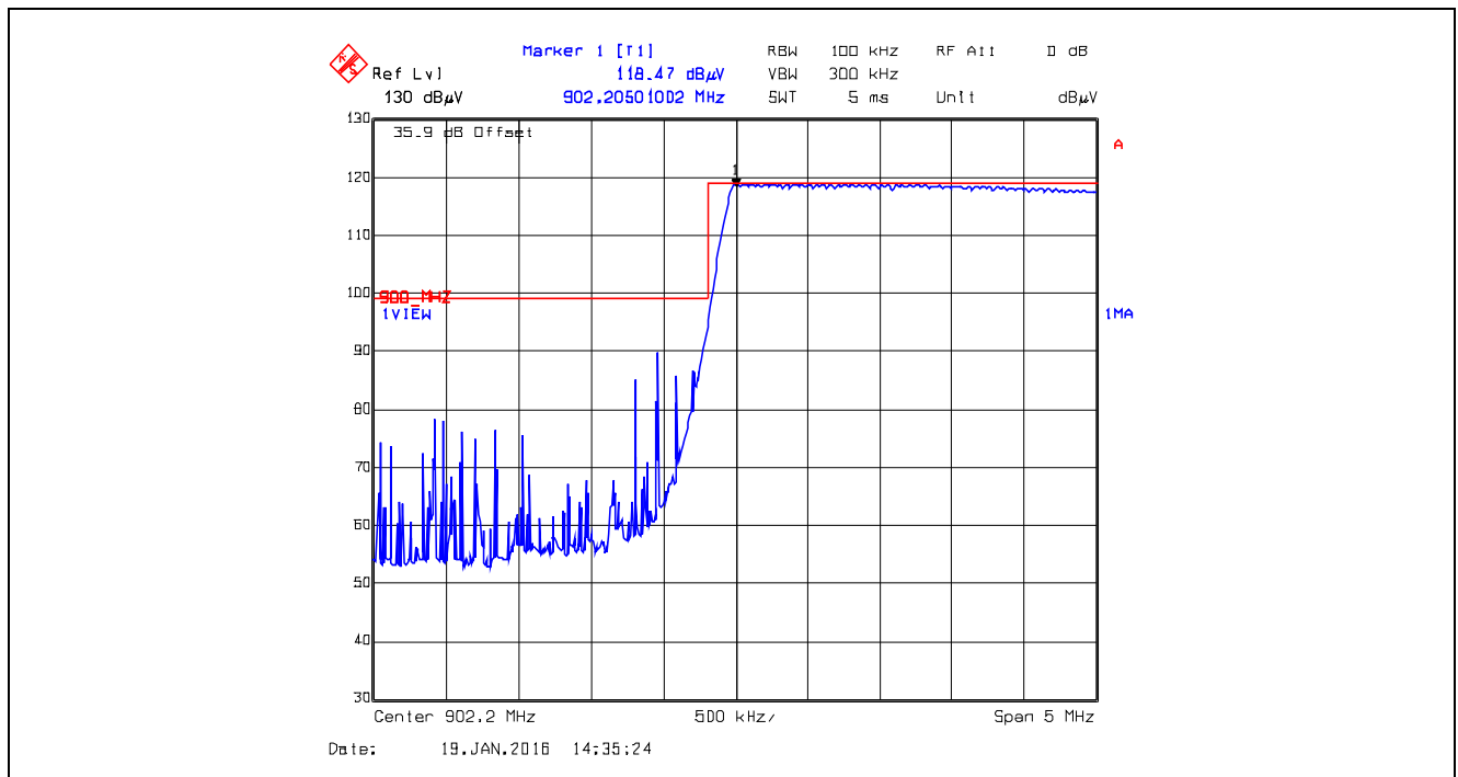
Plot 5.5.4.4.2.4. Band-Edge RF Radiated Emissions at 3 m, Vertical Polarization Pseudorandom Hopping Mode, Low End of Frequency Band, 902.2 MHz FSK, Data rate at 10 Kbps
