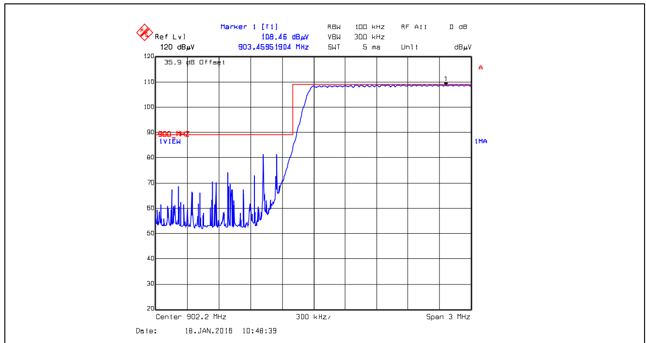
Plot 5.5.4.2.4. Band-Edge RF Radiated Emissions at 3 m, Vertical Polarization Pseudorandom Hopping Mode, Low End of Frequency Band, 902.2 MHz FSK, Data rate at 10 Kbps
