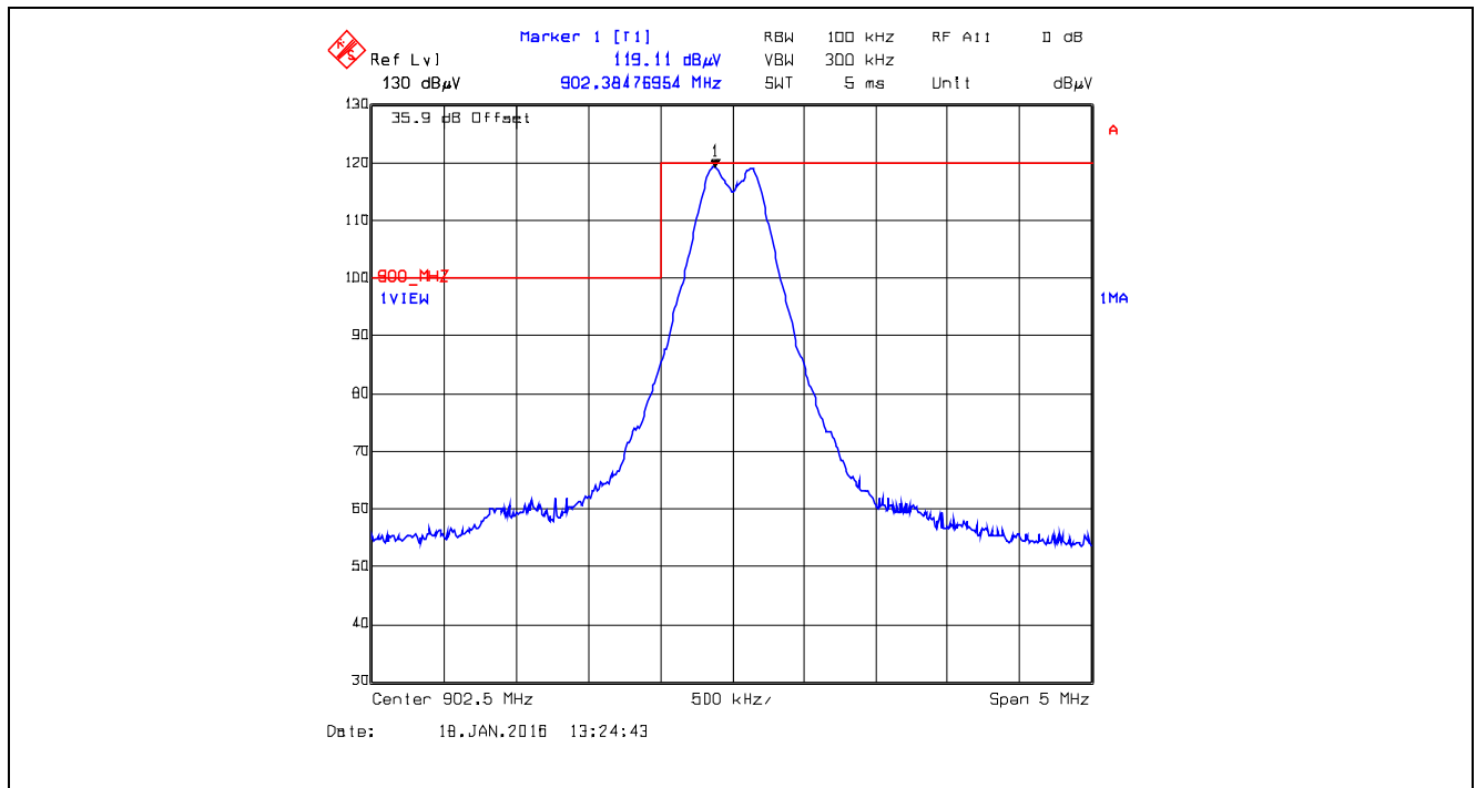
Plot 5.5.4.3.2.11. Band-Edge RF Radiated Emissions at 3 m, Vertical Polarization Single Frequency Mode, Low End of Frequency Band, 902.5 MHz, GFSK, Data Rate at 400 kbps
