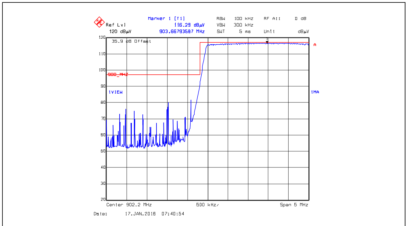
Plot 5.5.4.1.2.2. Band-Edge RF Radiated Emissions at 3 m, Horizontal Polarization Pseudorandom Hopping Mode, Low End of Frequency Band, 902.2 MHz, FSK, Data rate at 10 Kbps
