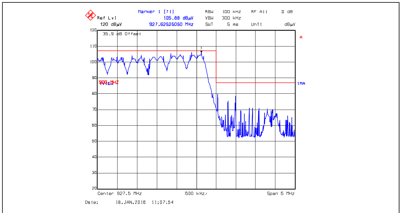
Plot 5.5.4.2.16. Band-Edge RF Radiated Emissions at 3 m, Vertical Polarization Pseudorandom Hopping Mode, High End of Frequency Band, 927.5 MHz, GFSK, Data Rate at 400 kbps
