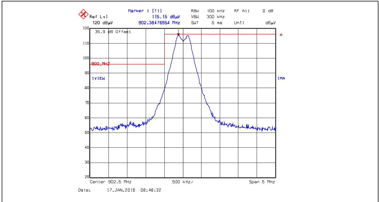
Plot 5.5.4.1.2.11. Band-Edge RF Radiated Emissions at 3 m, Vertical Polarization Single Frequency Mode, Low End of Frequency Band, 902.5 MHz, GFSK, Data Rate at 400 kbps
