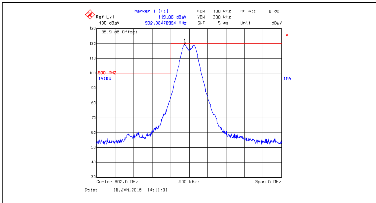
Plot 5.5.4.3.2.9. Band-Edge RF Radiated Emissions at 3 m, Horizontal Polarization Single Frequency Mode, Low End of Frequency Band, 902.5 MHz, GFSK, Data Rate at 400 kbps
