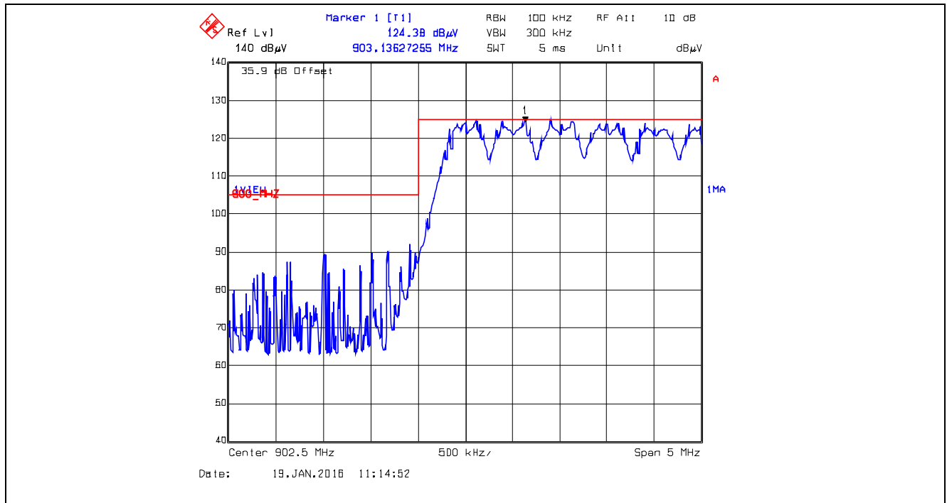
Plot 5.5.4.5.2.10. Band-Edge RF Radiated Emissions at 3 m, Horizontal Polarization Pseudorandom Hopping Mode, Low End of Frequency Band, 902.5 MHz, GFSK, Data Rate at 400 kbps
