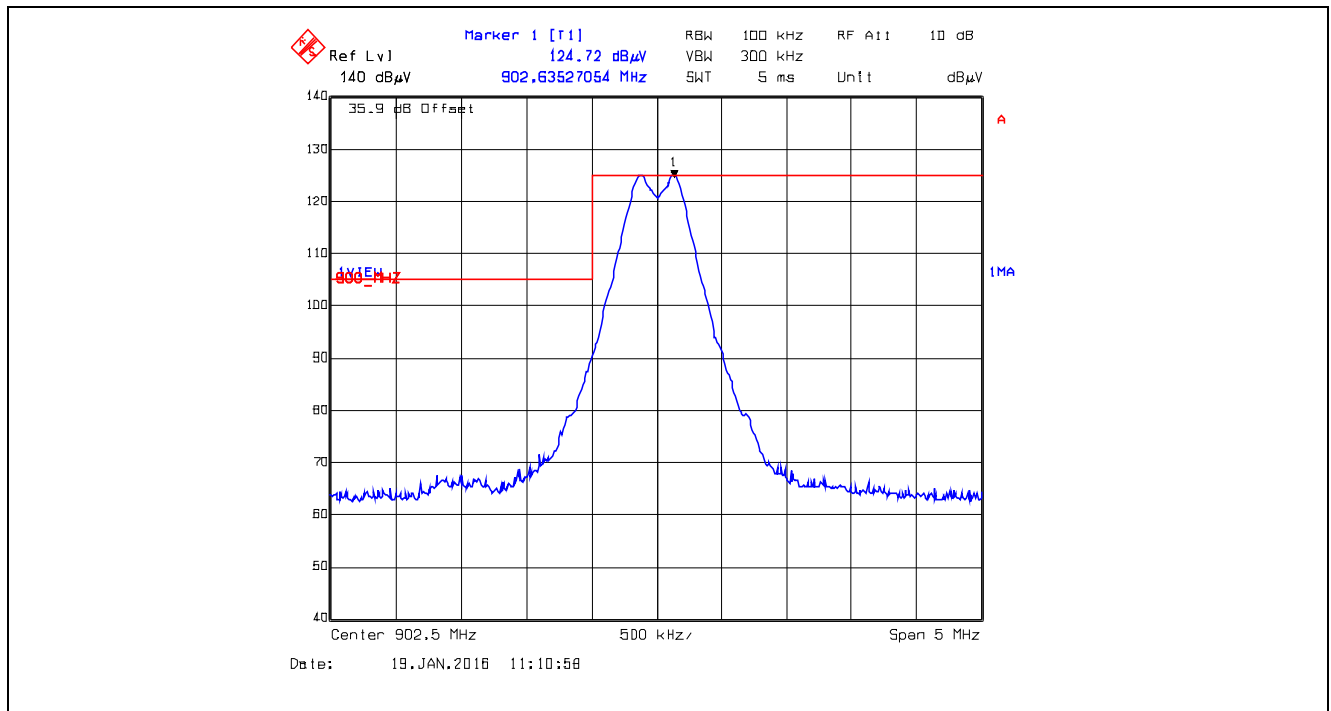
Plot 5.5.4.5.2.9. Band-Edge RF Radiated Emissions at 3 m, Horizontal Polarization Single Frequency Mode, Low End of Frequency Band, 902.5 MHz, GFSK, Data Rate at 400 kbps
