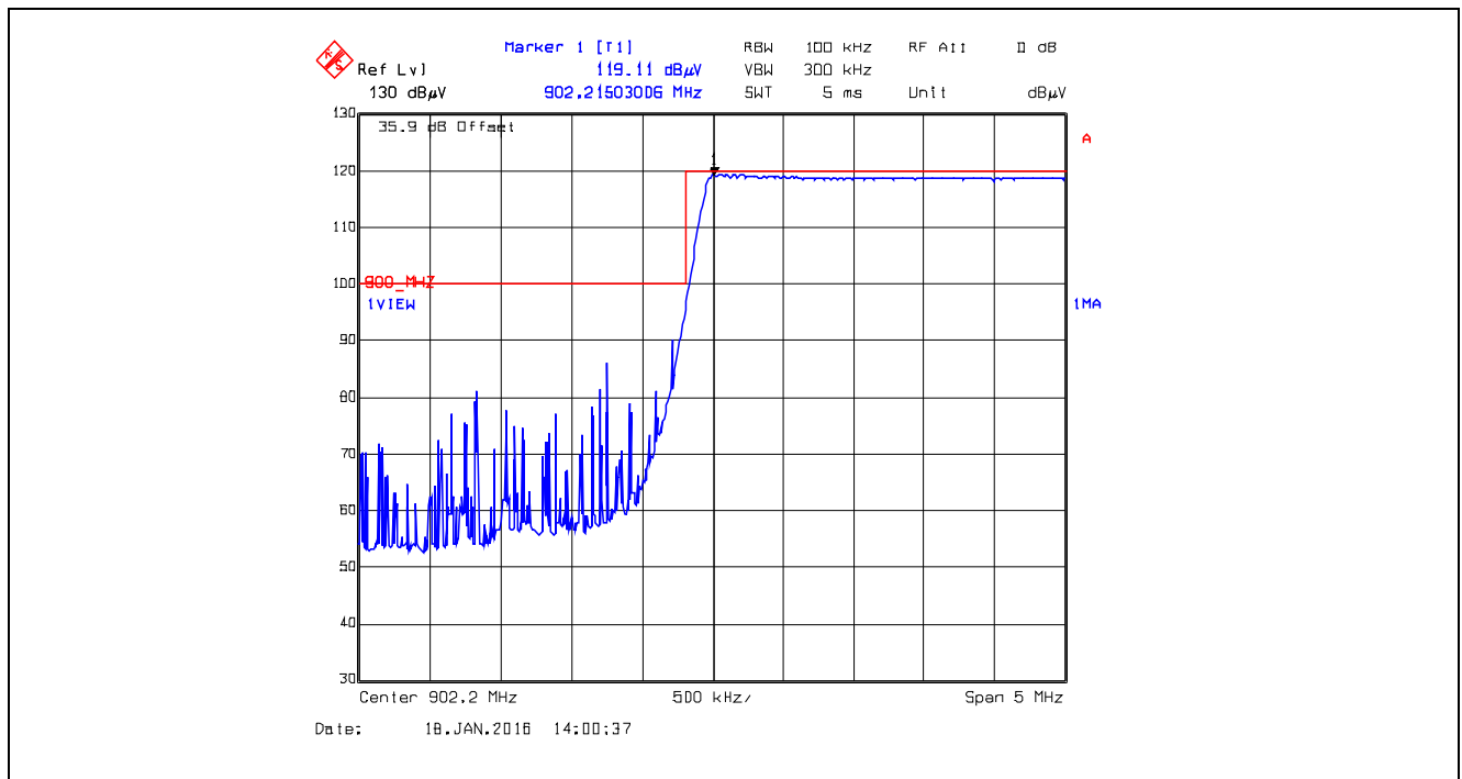
Plot 5.5.4.3.2.2. Band-Edge RF Radiated Emissions at 3 m, Horizontal Polarization Pseudorandom Hopping Mode, Low End of Frequency Band, 902.2 MHz, FSK, Data rate at 10 Kbps
