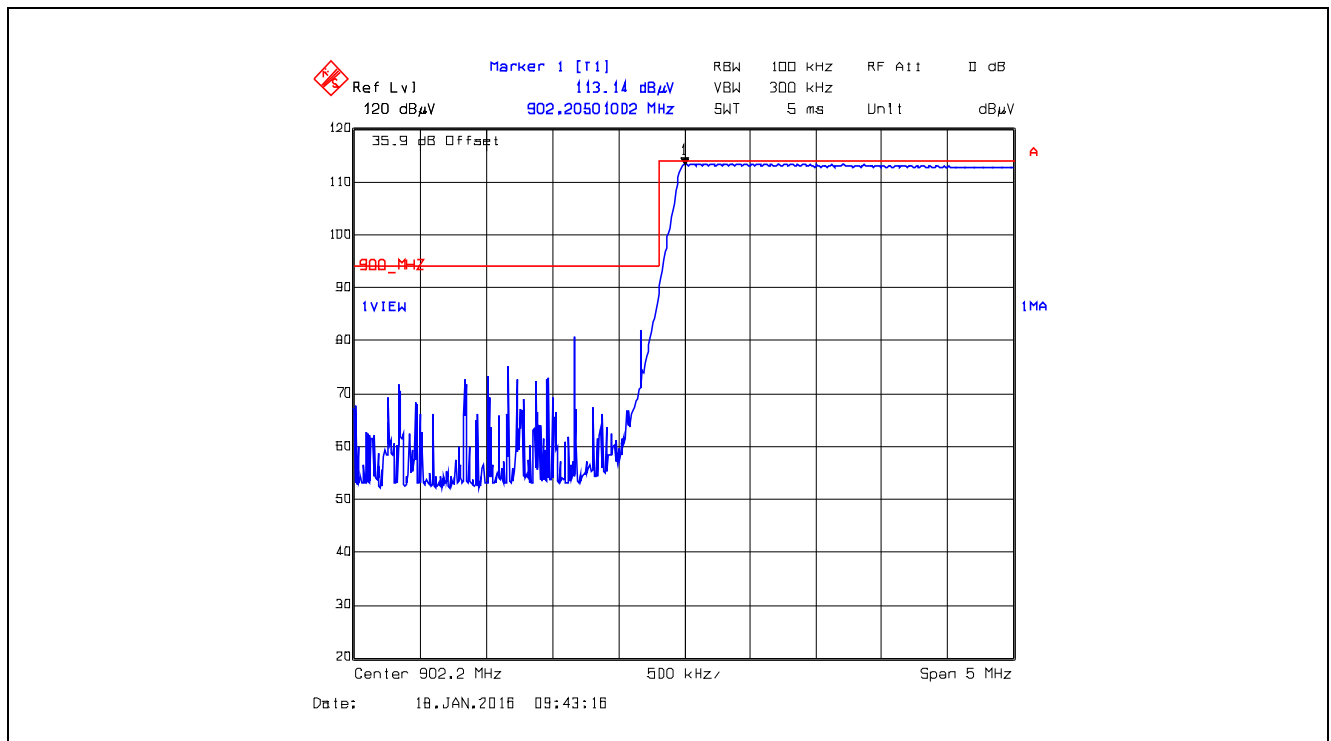
Plot 5.5.4.2.2.2. Band-Edge RF Radiated Emissions at 3 m, Horizontal Polarization Pseudorandom Hopping Mode, Low End of Frequency Band, 902.2 MHz, FSK, Data rate at 10 Kbps
