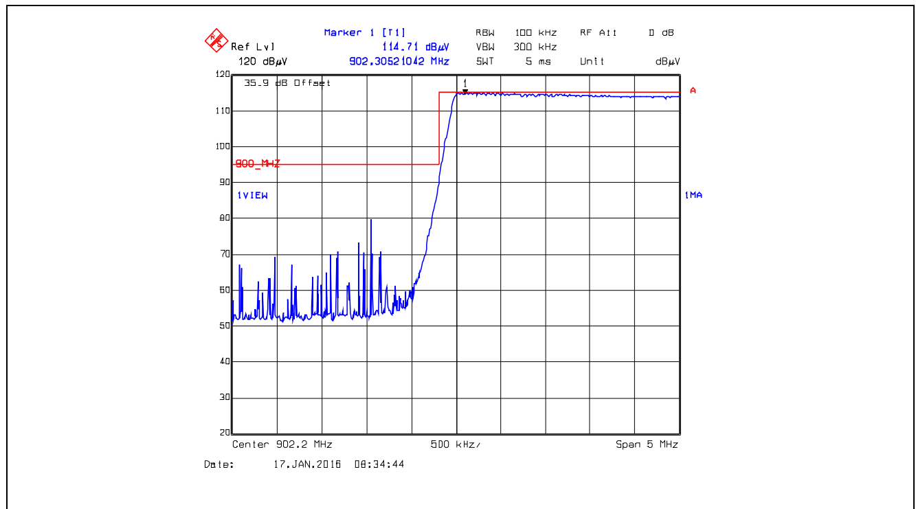
Plot 5.5.4.1.2.4. Band-Edge RF Radiated Emissions at 3 m, Vertical Polarization Pseudorandom Hopping Mode, Low End of Frequency Band, 902.2 MHz FSK, Data rate at 10 Kbps
