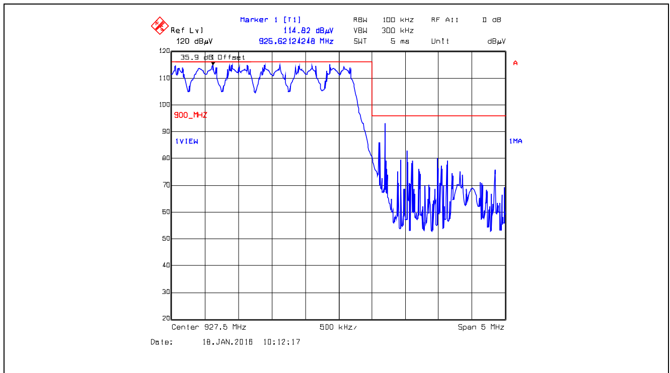
Plot 5.5.4.2.2.14. Band-Edge RF Radiated Emissions at 3 m, Horizontal Polarization Pseudorandom Hopping Mode, High End of Frequency Band, 927.5 MHz, GFSK, Data Rate at 400 kbps
