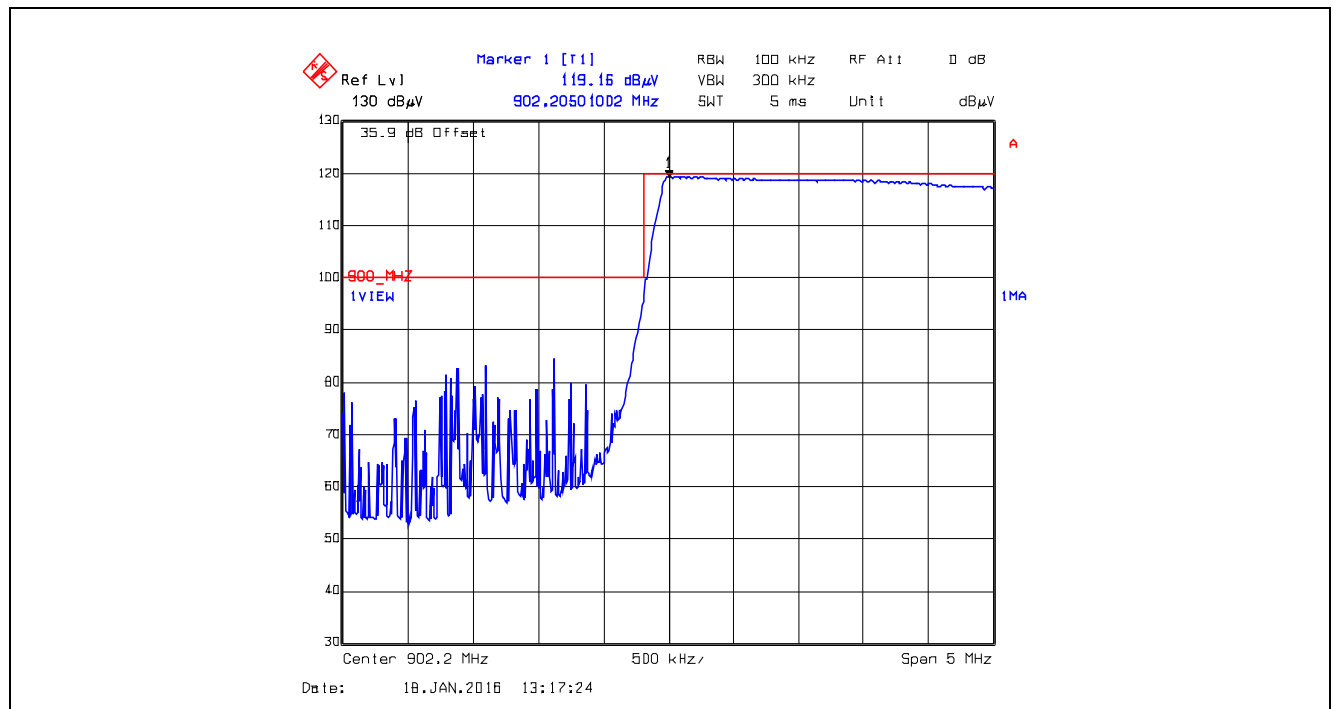
Plot 5.5.4.3.2.4. Band-Edge RF Radiated Emissions at 3 m, Vertical Polarization Pseudorandom Hopping Mode, Low End of Frequency Band, 902.2 MHz FSK, Data rate at 10 Kbps
