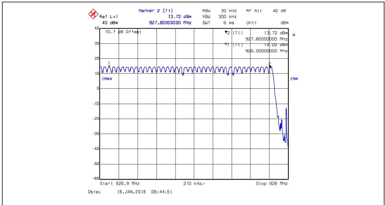
Plot 5.3.4.41. Number of Hopping Frequencies, DSSS8, Data Rate at 10 kbps 37 Hopping Channels from 926 – 927.8 MHz
