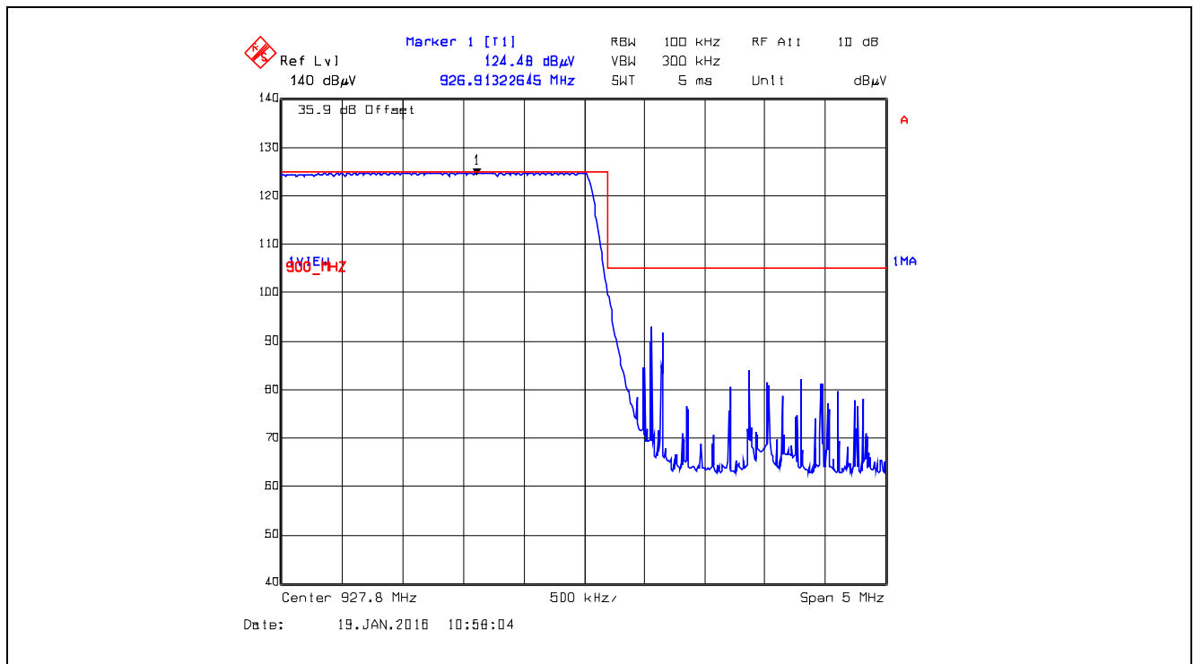
Plot 5.5.4.5.2.6. Band-Edge RF Radiated Emissions at 3 m, Horizontal Polarization Pseudorandom Hopping Mode, High End of Frequency Band, 927.8 MHz, FSK, Data rate at 10 Kbps
