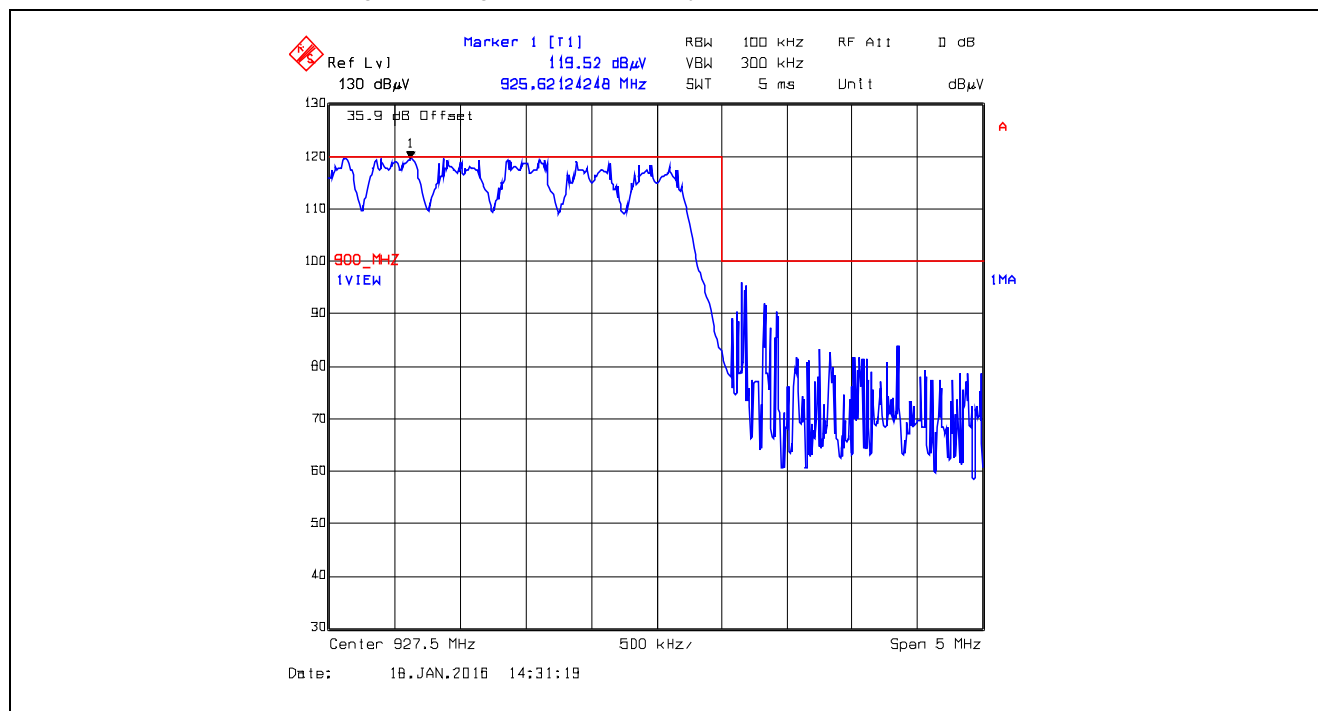
Plot 5.5.4.3.2.14. Band-Edge RF Radiated Emissions at 3 m, Horizontal Polarization Pseudorandom Hopping Mode, High End of Frequency Band, 927.5 MHz, GFSK, Data Rate at 400 kbps
