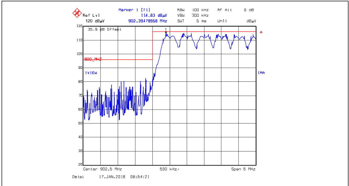
Plot 5.5.4.1.2.12. Band-Edge RF Radiated Emissions at 3 m, Vertical Polarization Pseudorandom Hopping Mode, Low End of Frequency Band, 902.5 MHz, GFSK, Data Rate at 400 kbps
