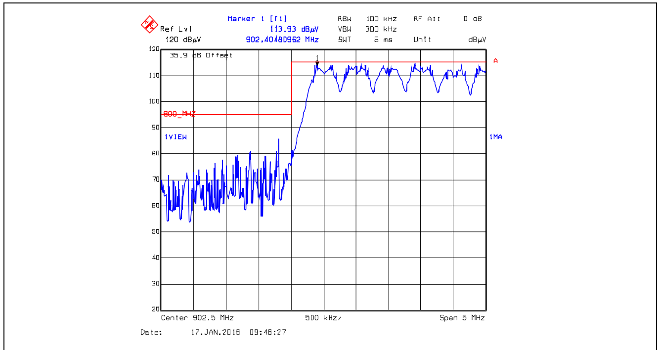
Plot 5.5.4.1.2.10. Band-Edge RF Radiated Emissions at 3 m, Horizontal Polarization Pseudorandom Hopping Mode, Low End of Frequency Band, 902.5 MHz, GFSK, Data Rate at 400 kbps
