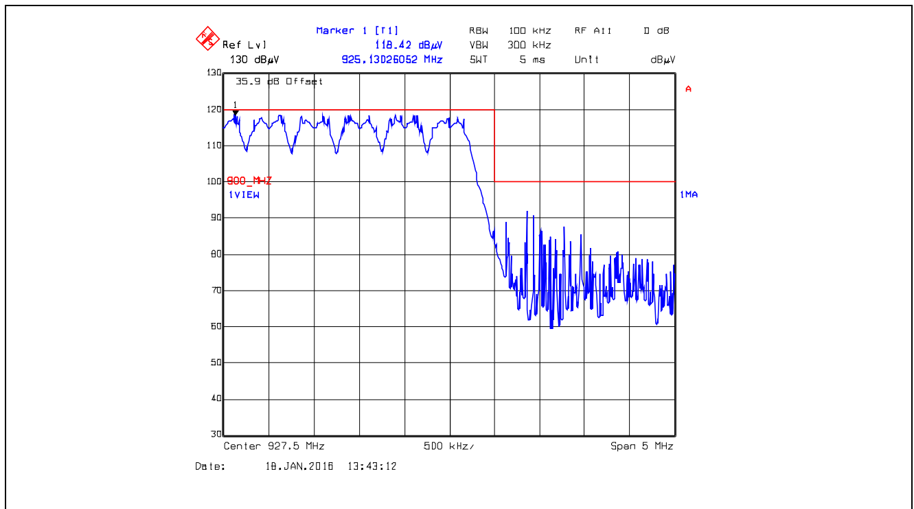
Plot 5.5.4.3.2.16. Band-Edge RF Radiated Emissions at 3 m, Vertical Polarization Pseudorandom Hopping Mode, High End of Frequency Band, 927.5 MHz, GFSK, Data Rate at 400 kbps
