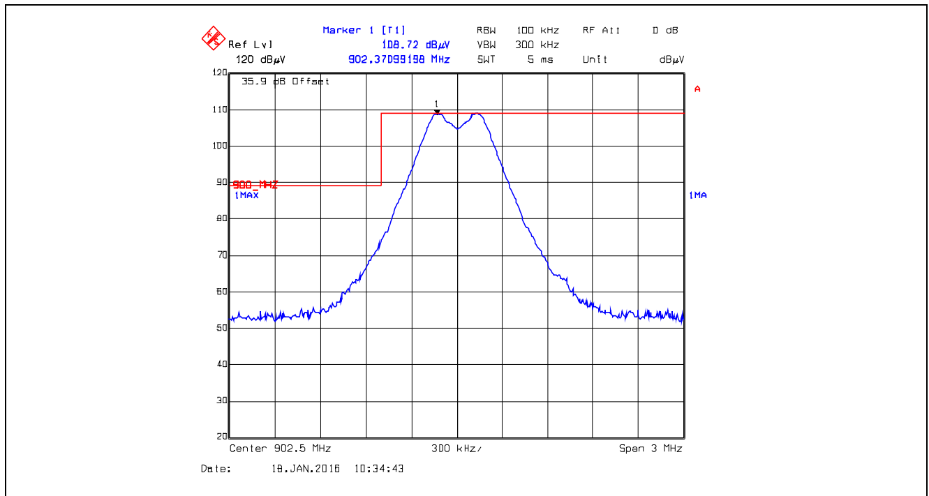
Plot 5.5.4.2.11. Band-Edge RF Radiated Emissions at 3 m, Vertical Polarization Single Frequency Mode, Low End of Frequency Band, 902.5 MHz, GFSK, Data Rate at 400 kbps
