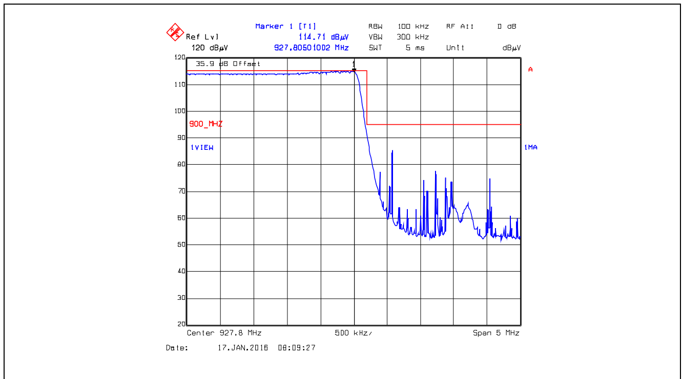
Plot 5.5.4.1.2.6. Band-Edge RF Radiated Emissions at 3 m, Horizontal Polarization Pseudorandom Hopping Mode, High End of Frequency Band, 927.8 MHz, FSK, Data rate at 10 Kbps
