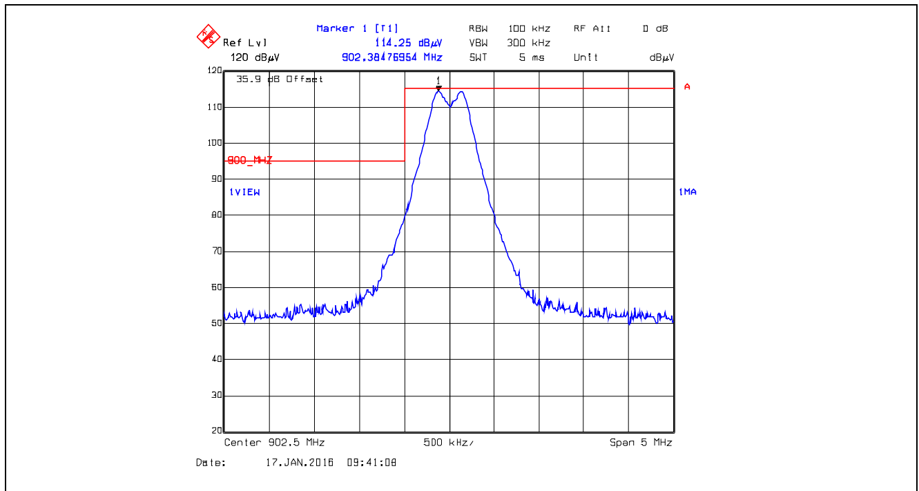
Plot 5.5.4.1.2.9. Band-Edge RF Radiated Emissions at 3 m, Horizontal Polarization Single Frequency Mode, Low End of Frequency Band, 902.5 MHz, GFSK, Data Rate at 400 kbps
