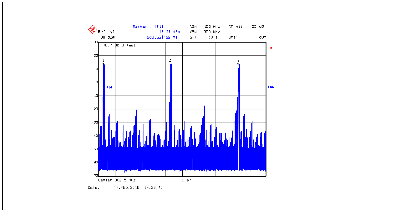
Plot 5.3.4.54. Time of Occupancy, 902.5 MHz, DSSS8, Data Rate at 400 kbps Average time of occupancy = 3 x (T on) in 10 seconds = 3 * 50.10 = 150.3 ms < 400ms
