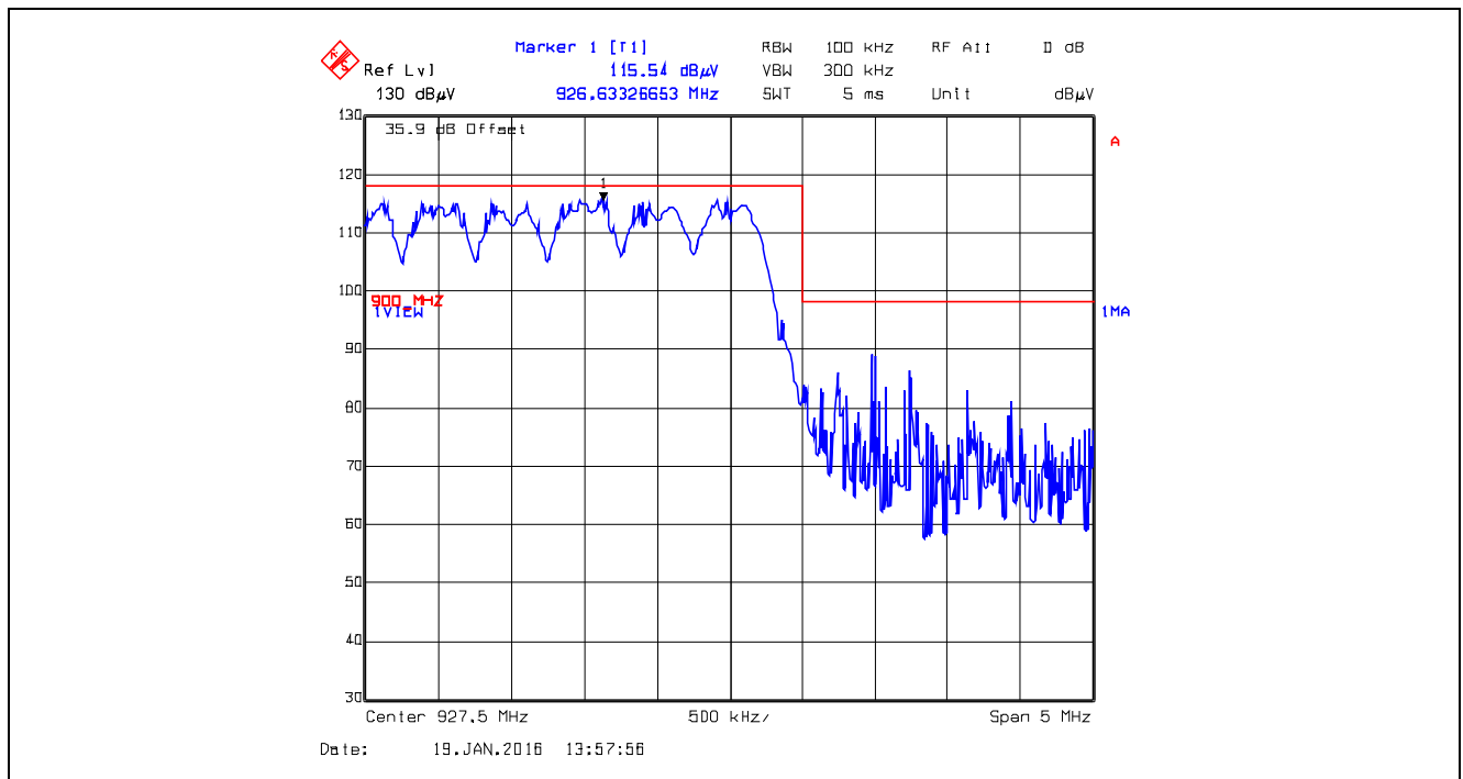
Plot 5.5.4.4.2.14. Band-Edge RF Radiated Emissions at 3 m, Horizontal Polarization Pseudorandom Hopping Mode, High End of Frequency Band, 927.5 MHz, GFSK, Data Rate at 400 kbps
