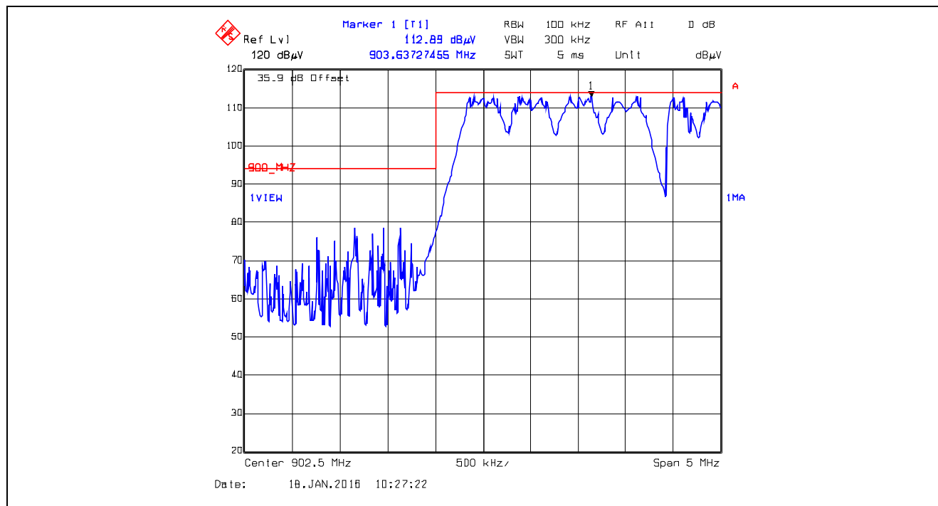
Plot 5.5.4.2.10. Band-Edge RF Radiated Emissions at 3 m, Horizontal Polarization Pseudorandom Hopping Mode, Low End of Frequency Band, 902.5 MHz, GFSK, Data Rate at 400 kbps
