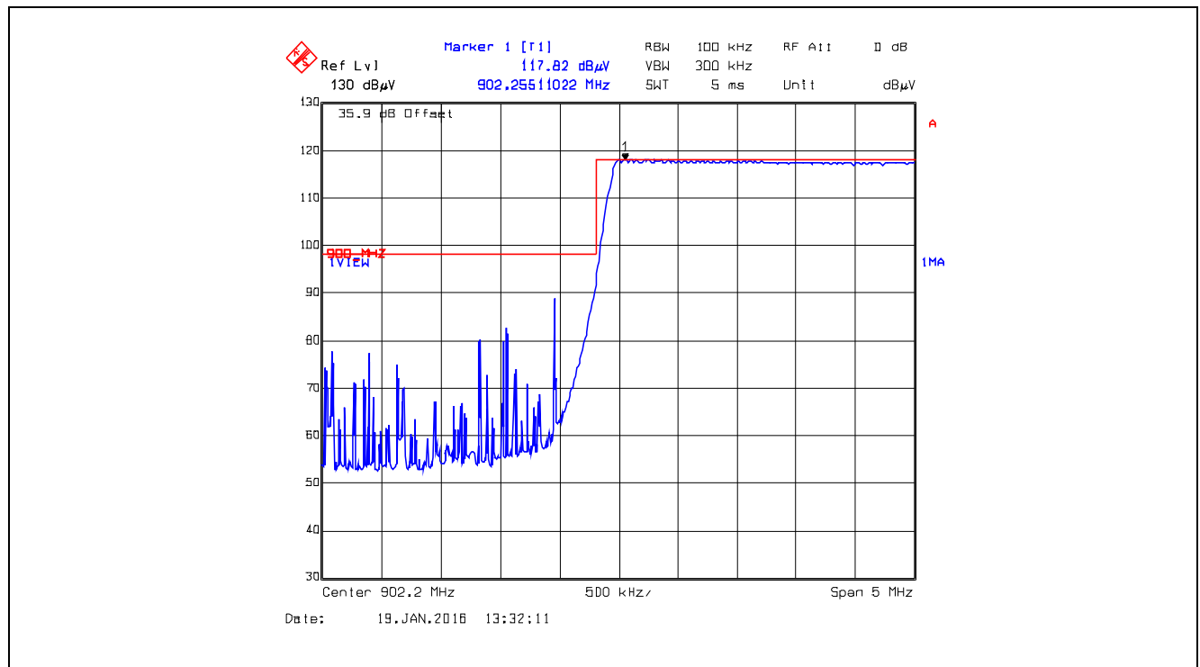
Plot 5.5.4.4.2.2. Band-Edge RF Radiated Emissions at 3 m, Horizontal Polarization Pseudorandom Hopping Mode, Low End of Frequency Band, 902.2 MHz, FSK, Data rate at 10 Kbps
