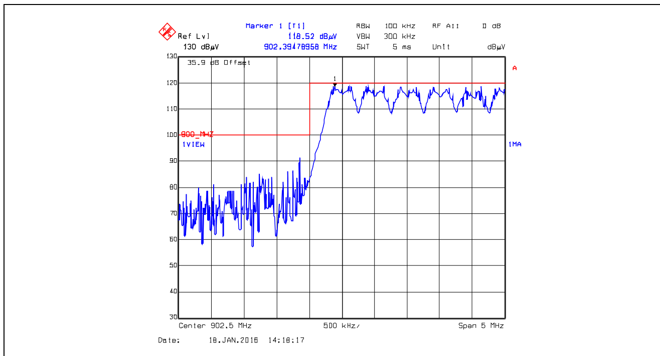
Plot 5.5.4.3.2.10. Band-Edge RF Radiated Emissions at 3 m, Horizontal Polarization Pseudorandom Hopping Mode, Low End of Frequency Band, 902.5 MHz, GFSK, Data Rate at 400 kbps
