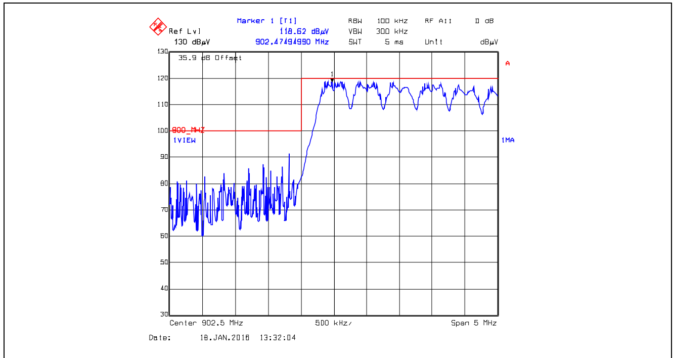
Plot 5.5.4.3.2.12. Band-Edge RF Radiated Emissions at 3 m, Vertical Polarization Pseudorandom Hopping Mode, Low End of Frequency Band, 902.5 MHz, GFSK, Data Rate at 400 kbps
