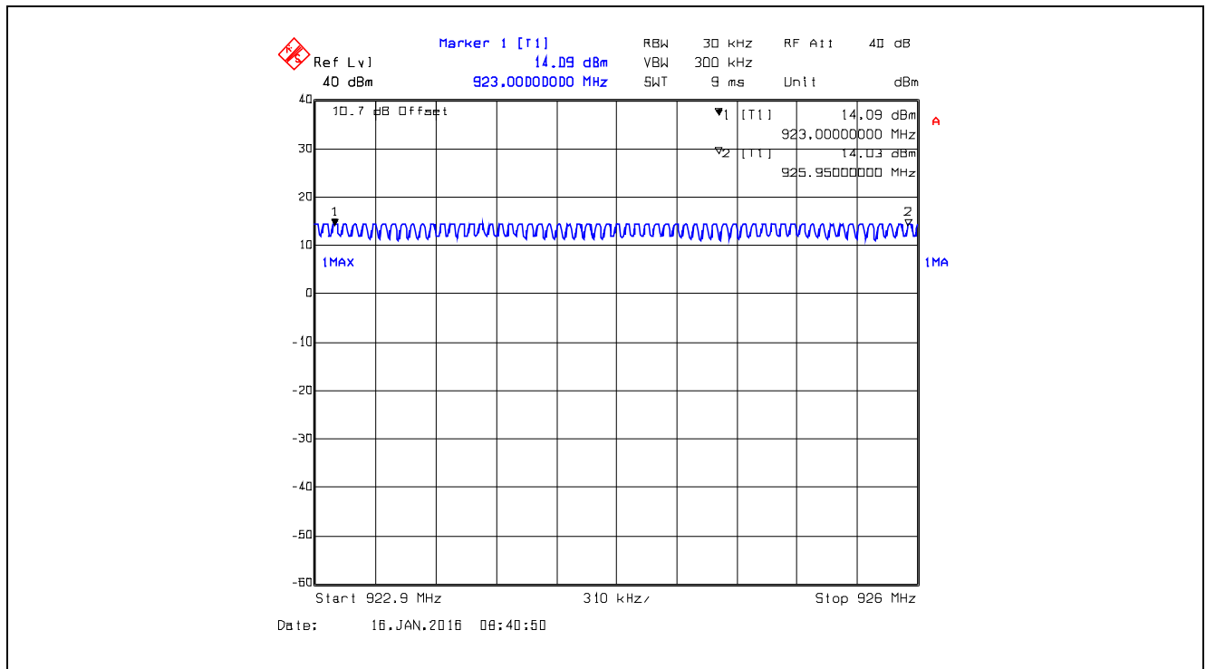
Plot 5.3.4.40. Number of Hopping Frequencies, DSSS8, Data Rate at 10 kbps 60 Hopping Channels from 923 – 926 MHz
