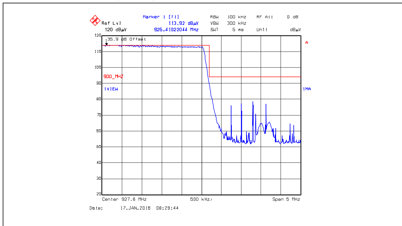
Plot 5.5.4.1.2.8. Band-Edge RF Radiated Emissions at 3 m, Vertical Polarization Pseudorandom Hopping Mode, High End of Frequency Band, 927.8 MHz, FSK, Data rate at 10 Kbps
