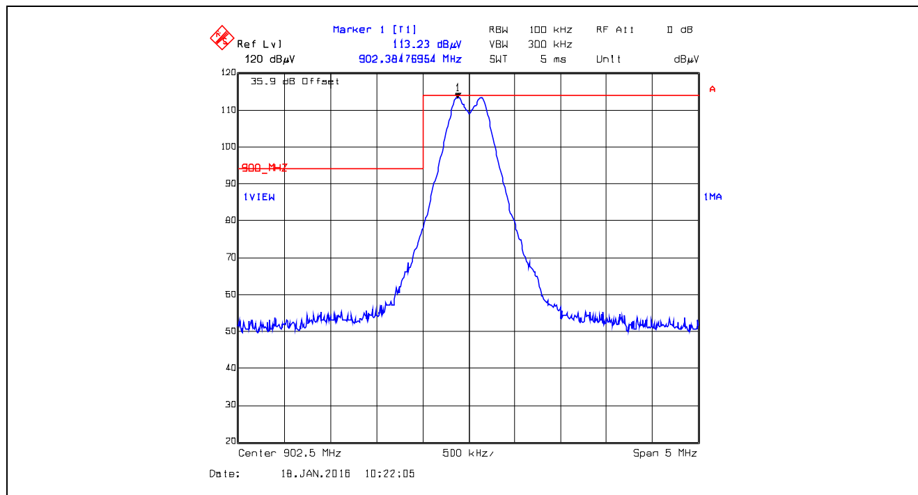
Plot 5.5.4.2.9. Band-Edge RF Radiated Emissions at 3 m, Horizontal Polarization Single Frequency Mode, Low End of Frequency Band, 902.5 MHz, GFSK, Data Rate at 400 kbps
