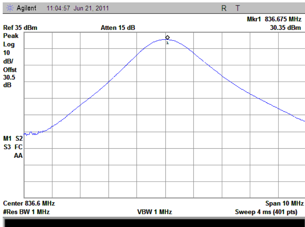
(Plot C2: GPRS 850MHz Channel = 190 Multislot Config: 2 Down, 3Up)
