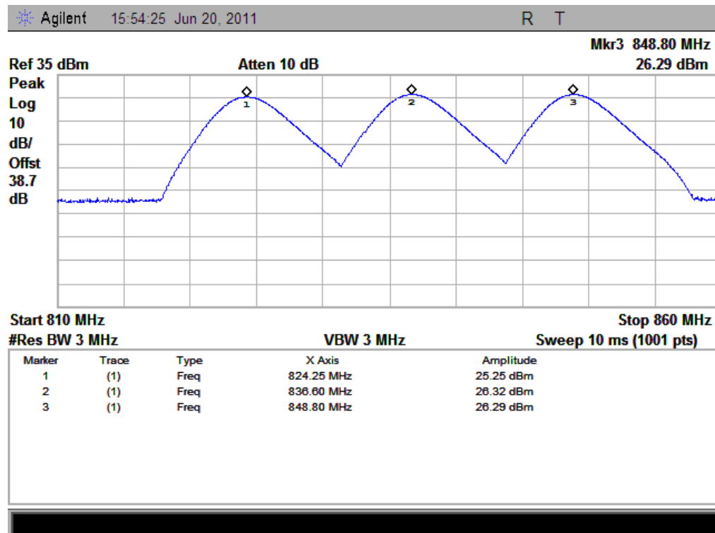
(Plot A: GPRS 850MHz Channel = 128,190,251 Multislot Config: 1 Down, 4Up)
