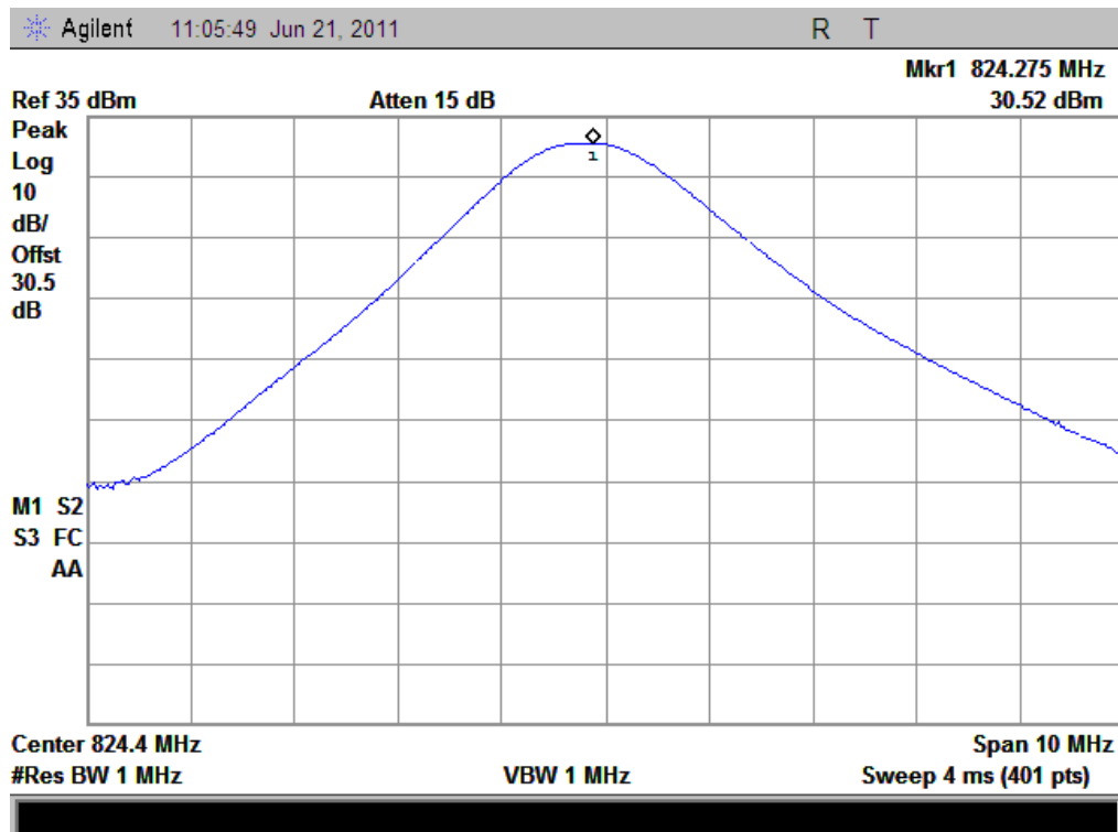
(Plot C1: GPRS 850MHz Channel = 128 Multislot Config: 2 Down, 3Up)
