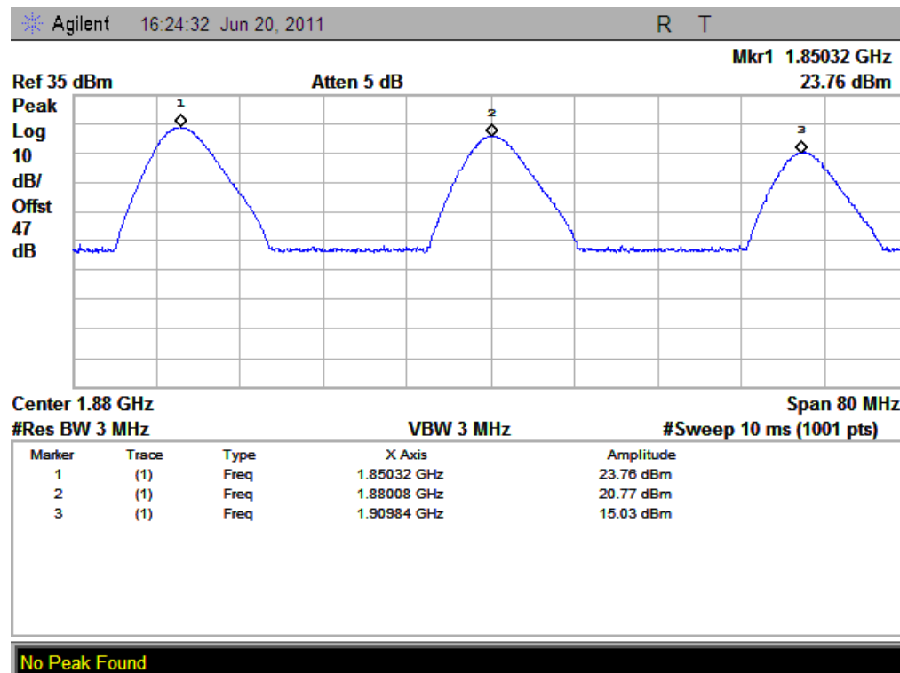
(Plot B: GPRS 1900MHz Channel = 512, 661, 810 Multislot Config: 1 Down, 4Up)
