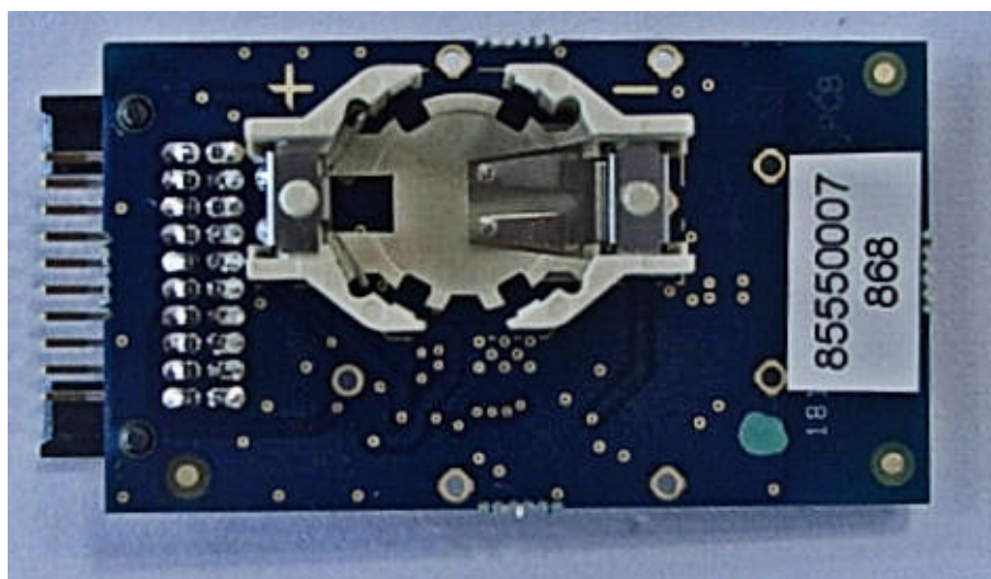
RF Module – Bottom View
