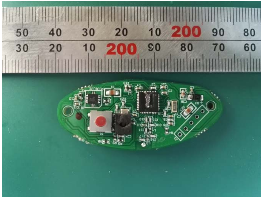
EUT (PicoBong Egg) - Mainboard Front View
