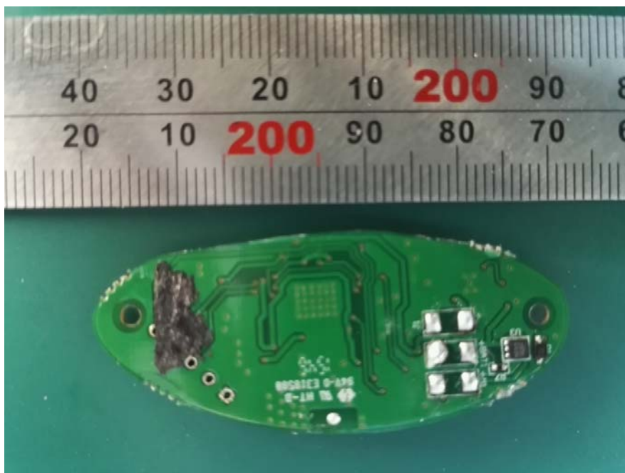
EUT(PicoBong Egg) - Mainboard Rear View
