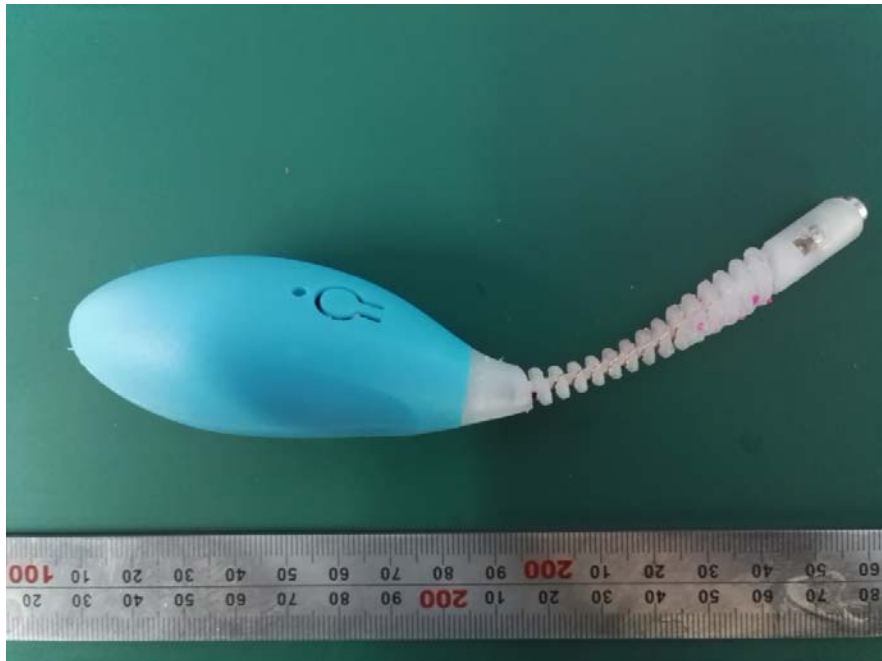
EUT (PicoBong Egg) - Cover Off View -3
