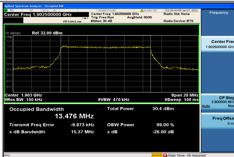
Band2-15MHz-QPSK-19125-75RB#0-13.476
