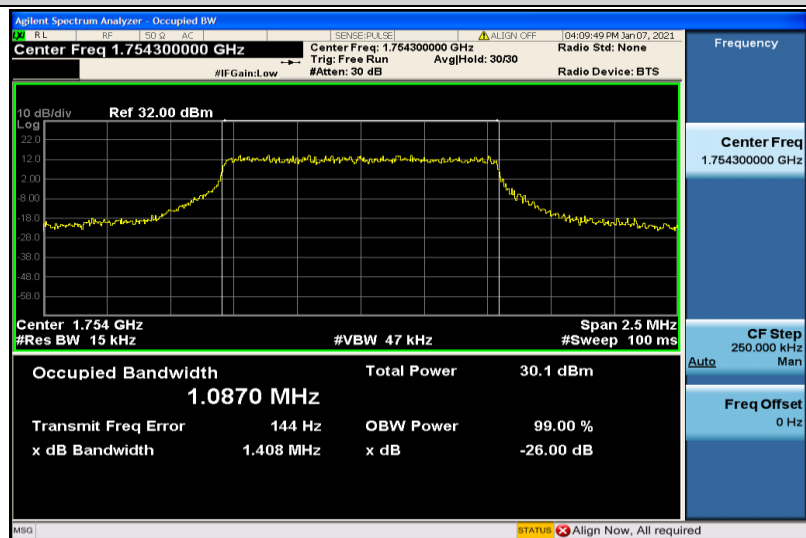
Band4-1.4MHz-QPSK-20393-6RB#0-1.0870
