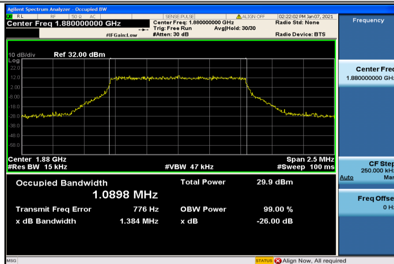
Band2-1.4MHz-QPSK-18900-6RB#0-1.0898
