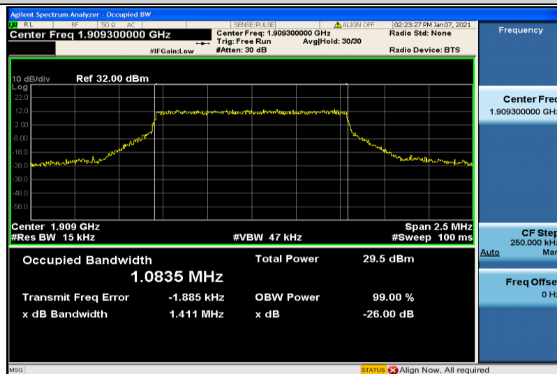
Band2-1.4MHz-QPSK-19193-6RB#0-1.0835
