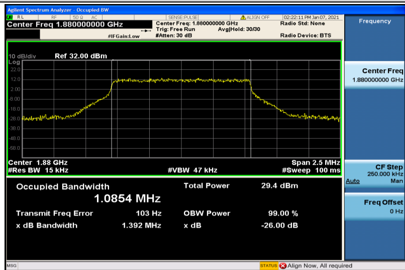
Band2-1.4MHz-16QAM-18900-6RB#0-1.0854
