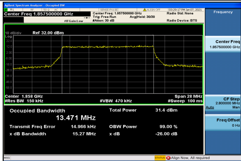
Band2-15MHz-16QAM-18675-75RB#0-13.471
