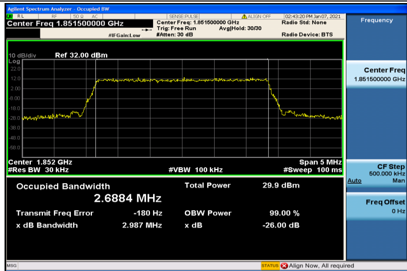
Band2-3MHz-16QAM-18615-15RB#0-2.6884
