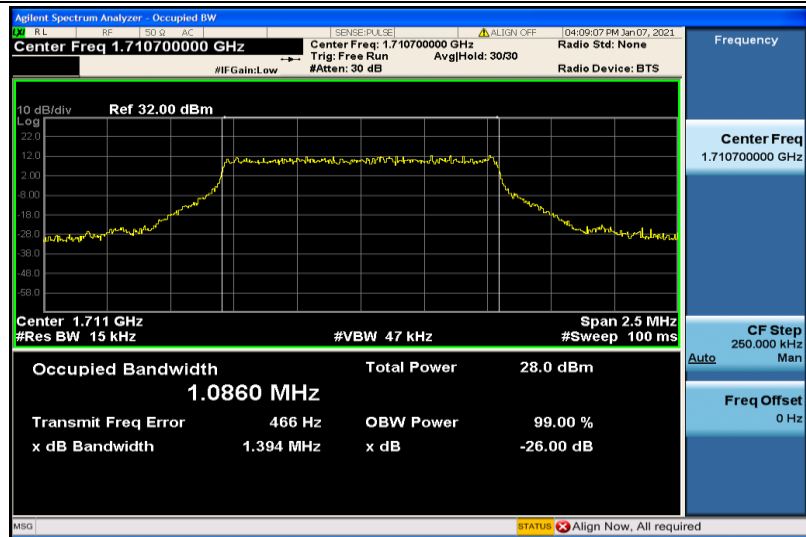
Band4-1.4MHz-QPSK-19957-6RB#0-1.0860
