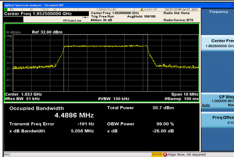
Band2-5MHz-16QAM-18625-25RB#0-4.4886
