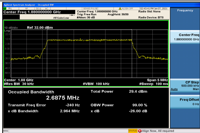
Band2-3MHz-16QAM-18900-15RB#0-2.6875
