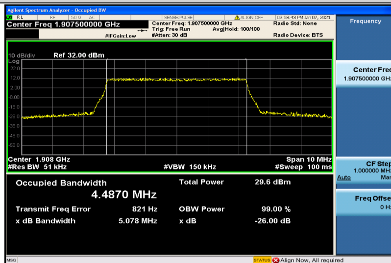
Band2-5MHz-16QAM-19175-25RB#0-4.4870
