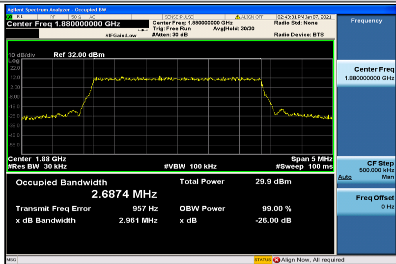
Band2-3MHz-QPSK-18900-15RB#0-2.6874
