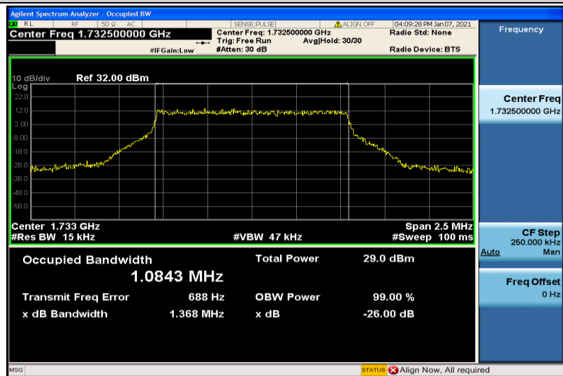
Band4-1.4MHz-QPSK-20175-6RB#0-1.0843
