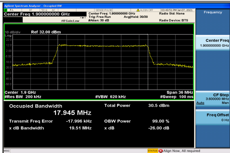
Band2-20MHz-16QAM-19100-100RB#0-17.945
