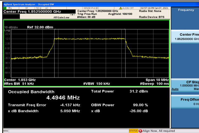
Band2-5MHz-QPSK-18625-25RB#0-4.4946
