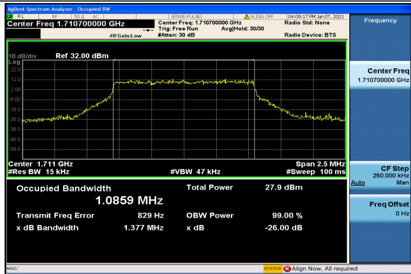
Band4-1.4MHz-16QAM-19957-6RB#0-1.0859
