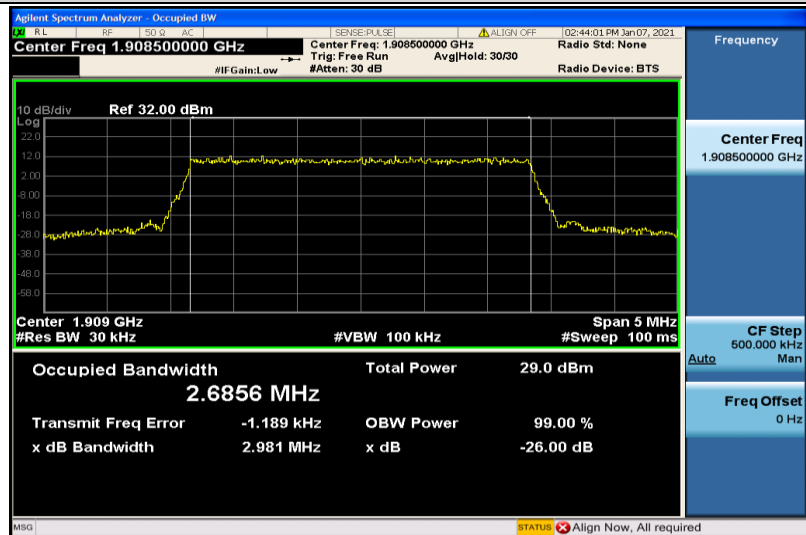
Band2-3MHz-16QAM-19185-15RB#0-2.6856
