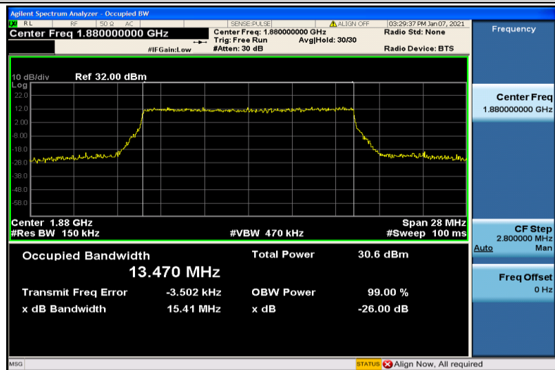
Band2-15MHz-16QAM-18900-75RB#0-13.470
