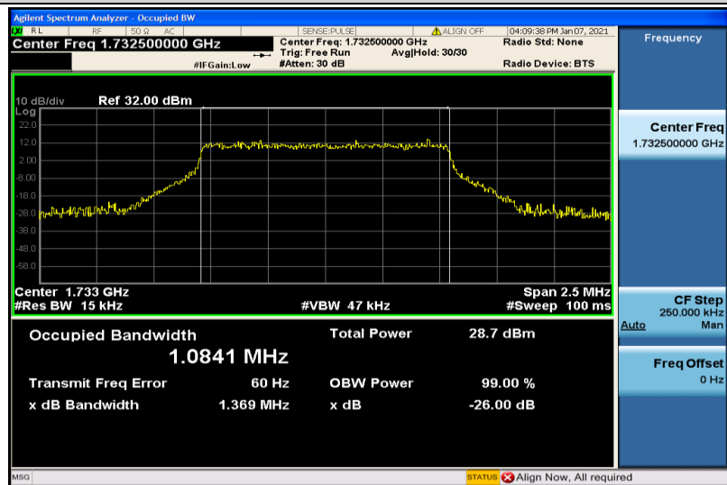
Band4-1.4MHz-16QAM-20175-6RB#0-1.0841
