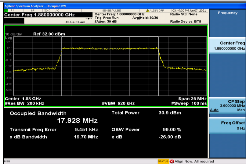
Band2-20MHz-16QAM-18900-100RB#0-17.928
