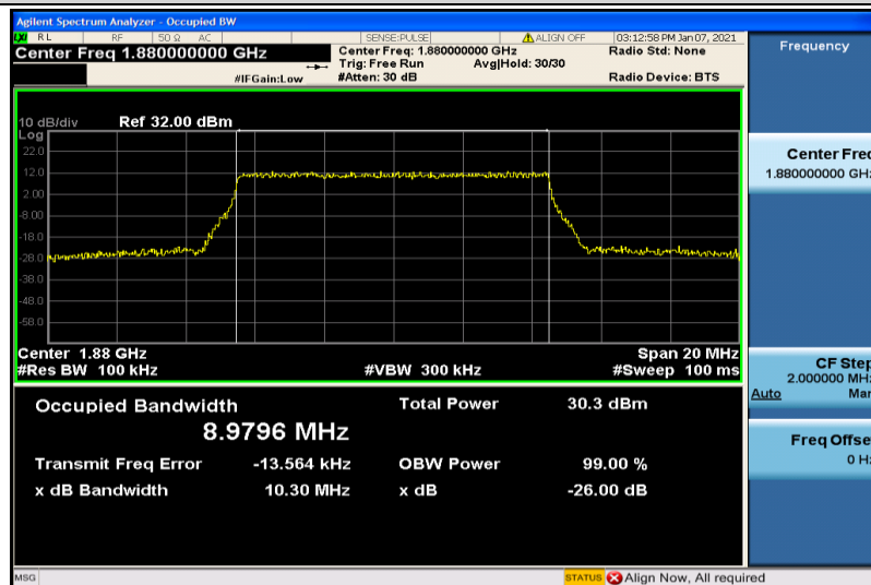
Band2-10MHz-16QAM-18900-50RB#0-8.9796
