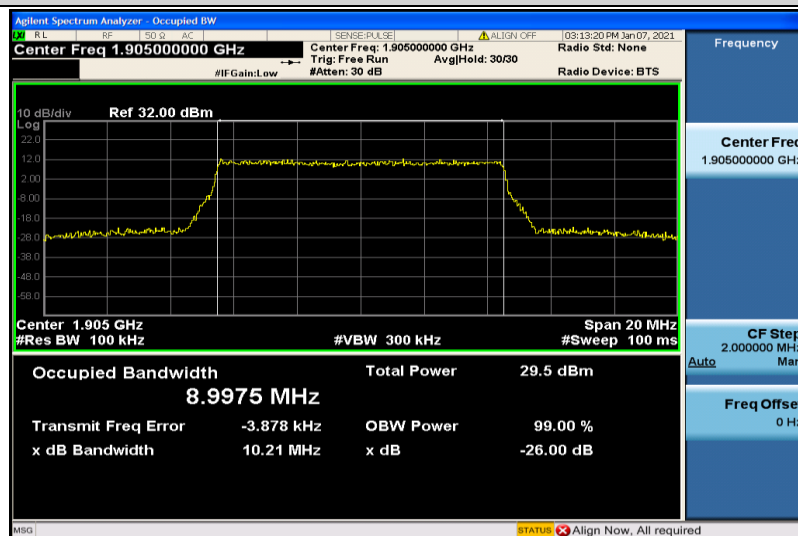
Band2-10MHz-16QAM-19150-50RB#0-8.9975
