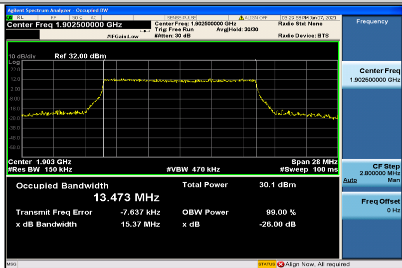
Band2-15MHz-16QAM-19125-75RB#0-13.473
