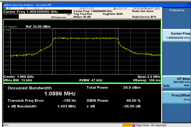
Band2-1.4MHz-16QAM-19193-6RB#0-1.0886
