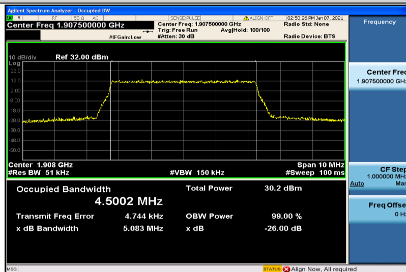
Band2-5MHz-QPSK-19175-25RB#0-4.5002
