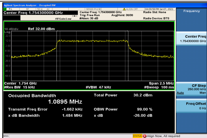
Band4-1.4MHz-16QAM-20393-6RB#0-1.0895
