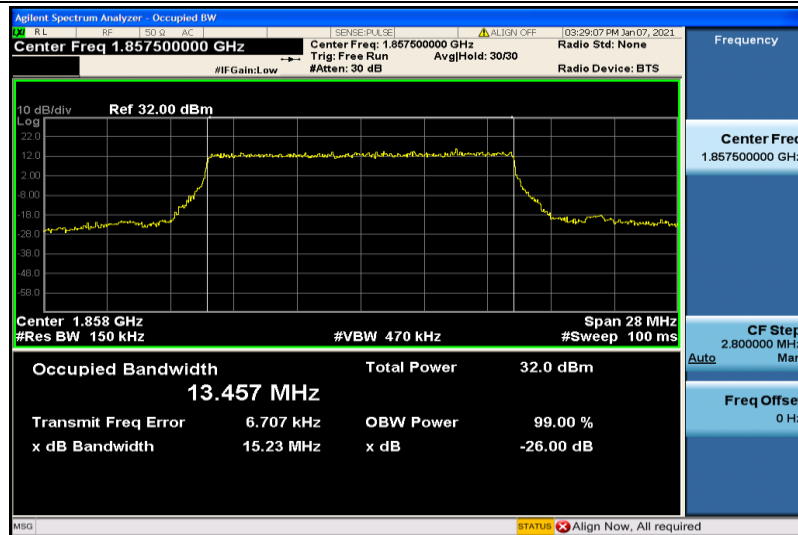
Band2-15MHz-QPSK-18675-75RB#0-13.457
