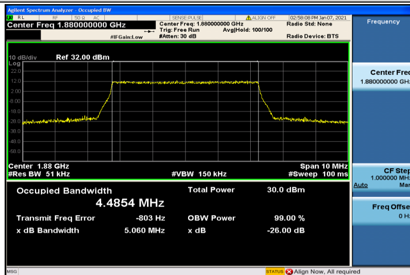
Band2-5MHz-16QAM-18900-25RB#0-4.4854
