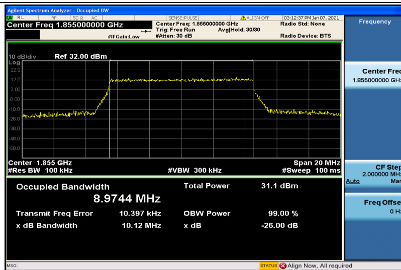
Band2-10MHz-16QAM-18650-50RB#0-8.9744
