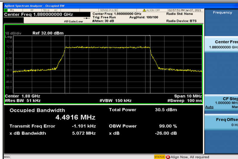
Band2-5MHz-QPSK-18900-25RB#0-4.4916
