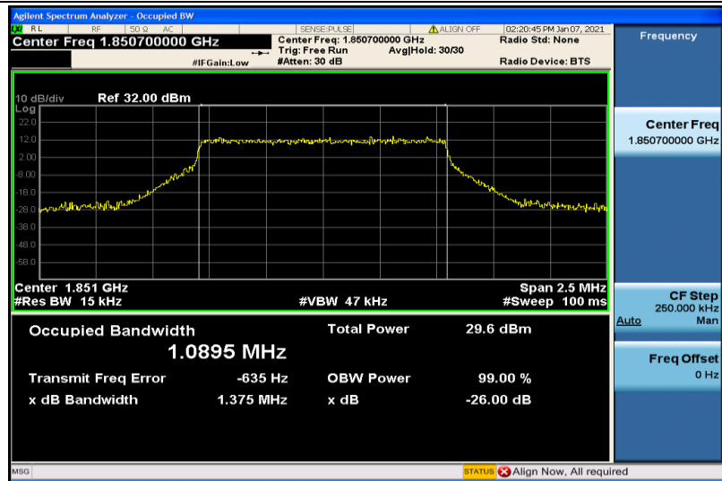
Band2-1.4MHz-16QAM-18607-6RB#0-1.0895
