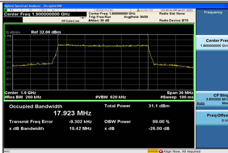
Band2-20MHz-QPSK-19100-100RB#0-17.923
