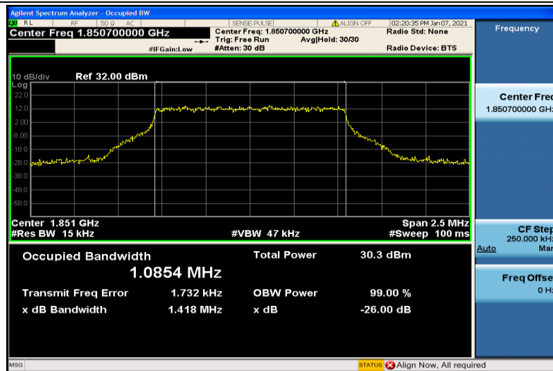
Band2-1.4MHz-QPSK-18607-6RB#0-1.0854
