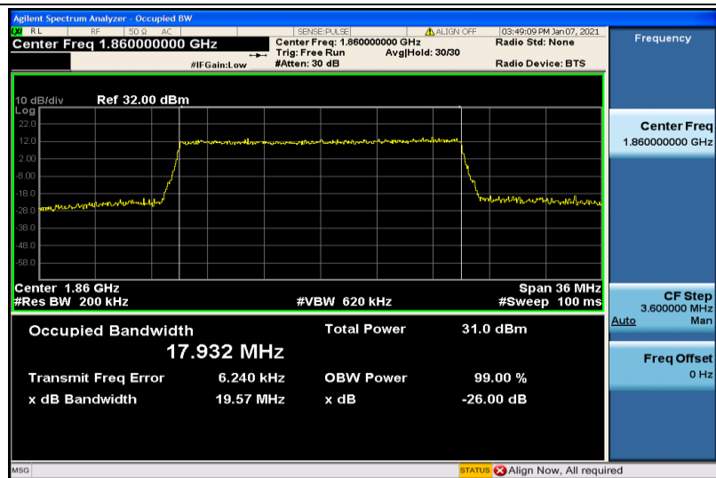
Band2-20MHz-16QAM-18700-100RB#0-17.932
