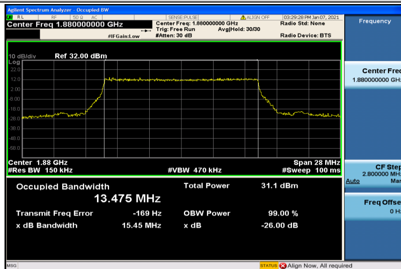
Band2-15MHz-QPSK-18900-75RB#0-13.475
