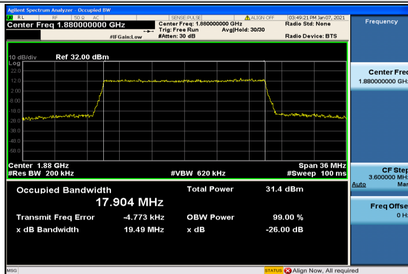
Band2-20MHz-QPSK-18900-100RB#0-17.904
