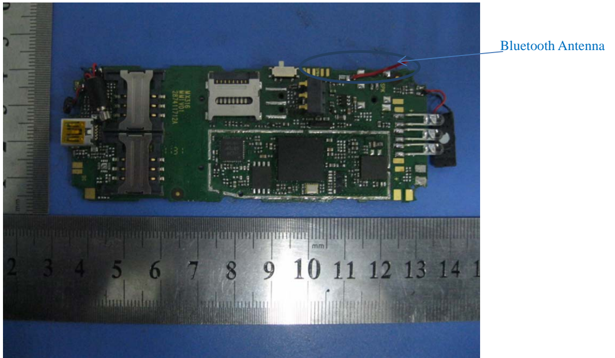
Bluetooth Antenna - Top View
