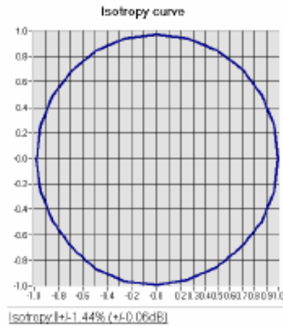
Isotropy at 1900 MHz
