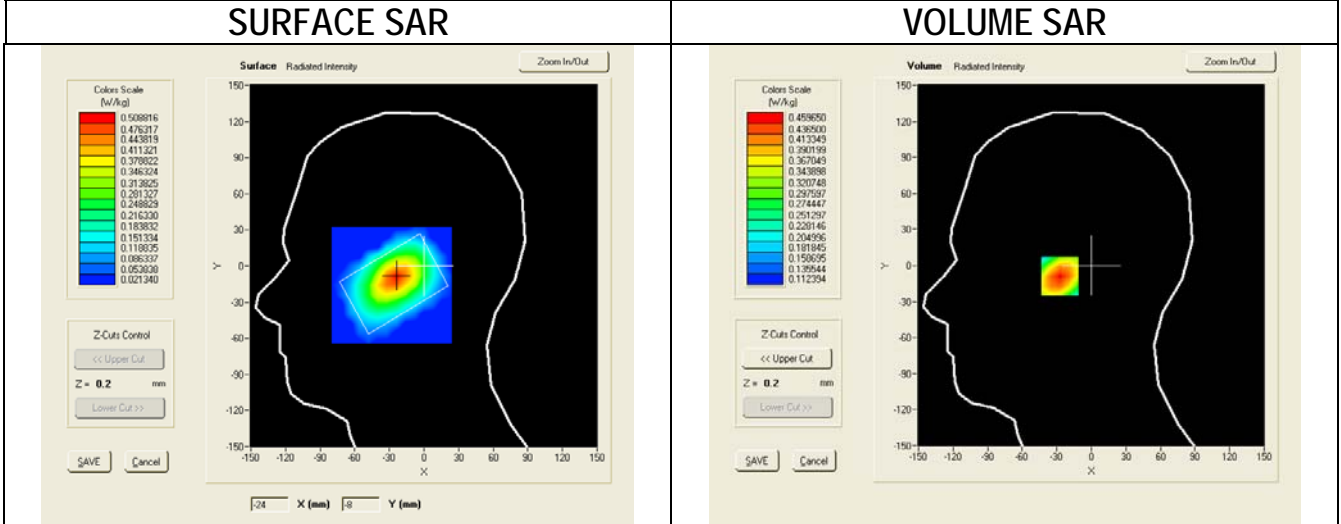
SAR, Z Axis Scan (X = -24, Y = -9)
