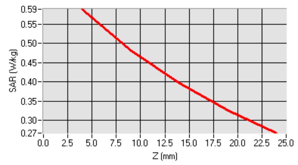
SAR, Z Axis Scan (X = 3, Y = -14)
