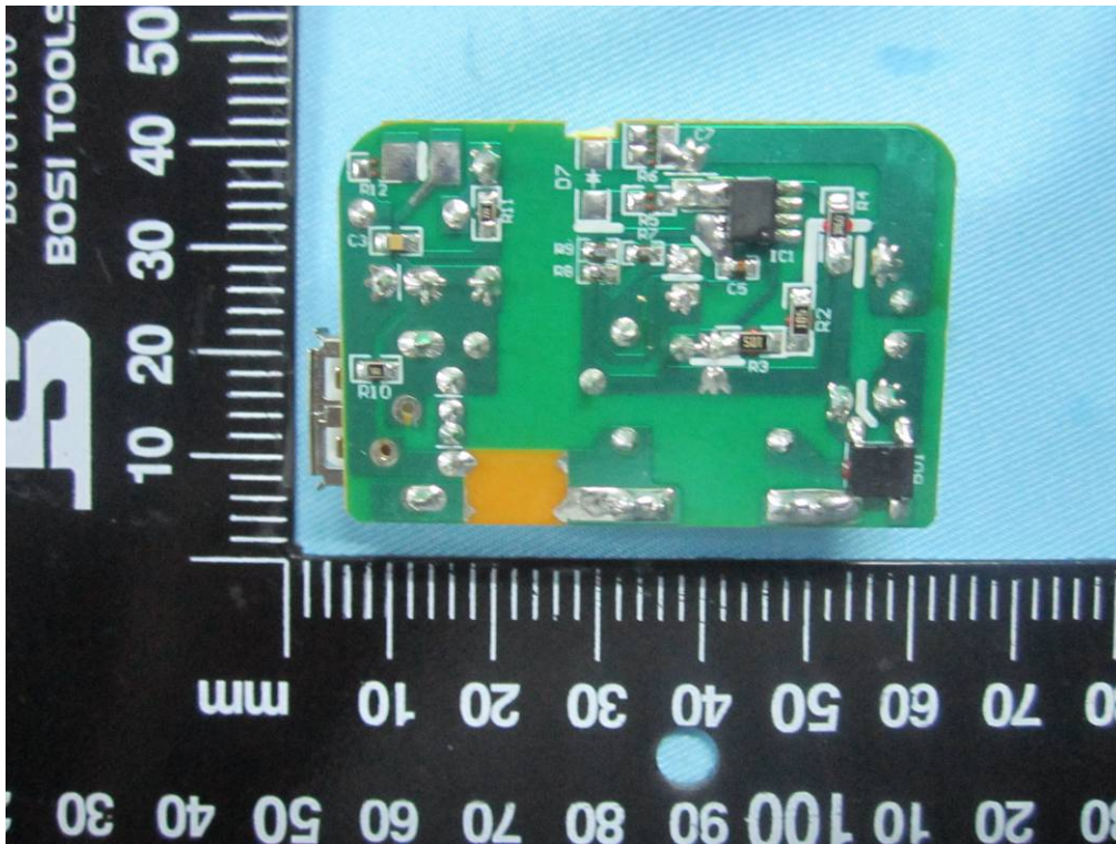
Adapter Mainborad - Rear View
