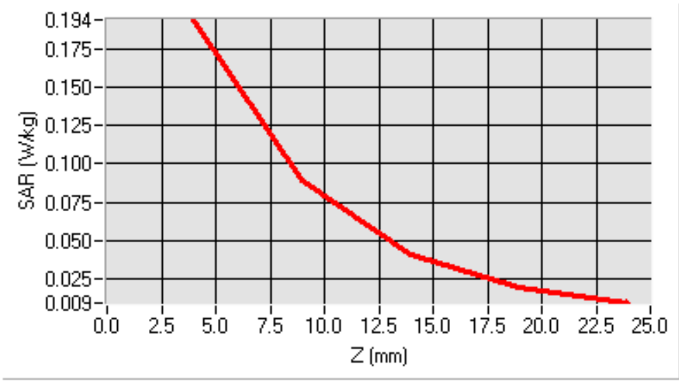
SAR, Z Axis Scan (X = 16, Y = -23)
