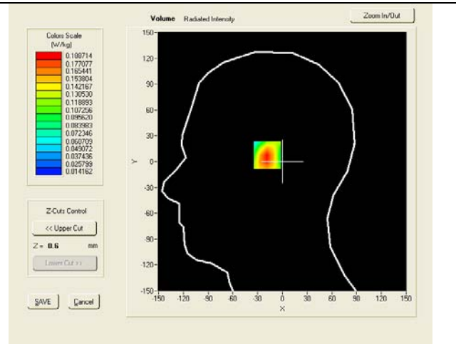
SAR, Z Axis Scan (X = -16, Y = 8)
