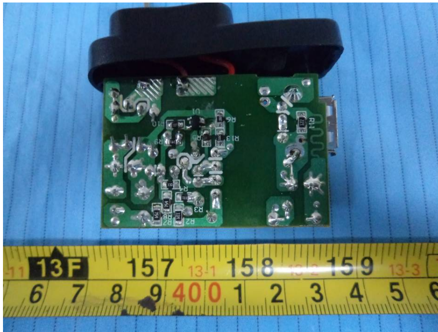
EUT – Adapter Board Bottom View
