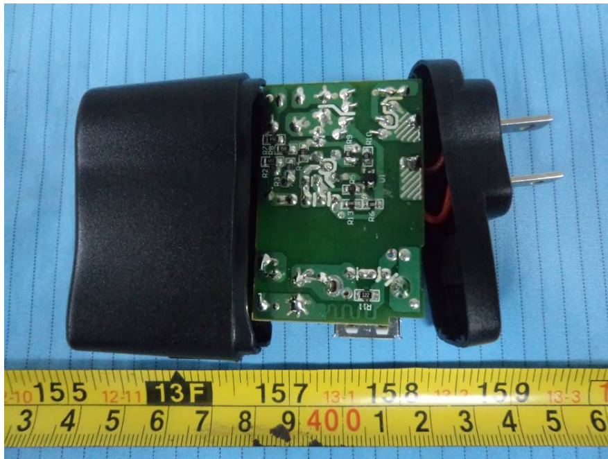
EUT – Adapter Cover off View
