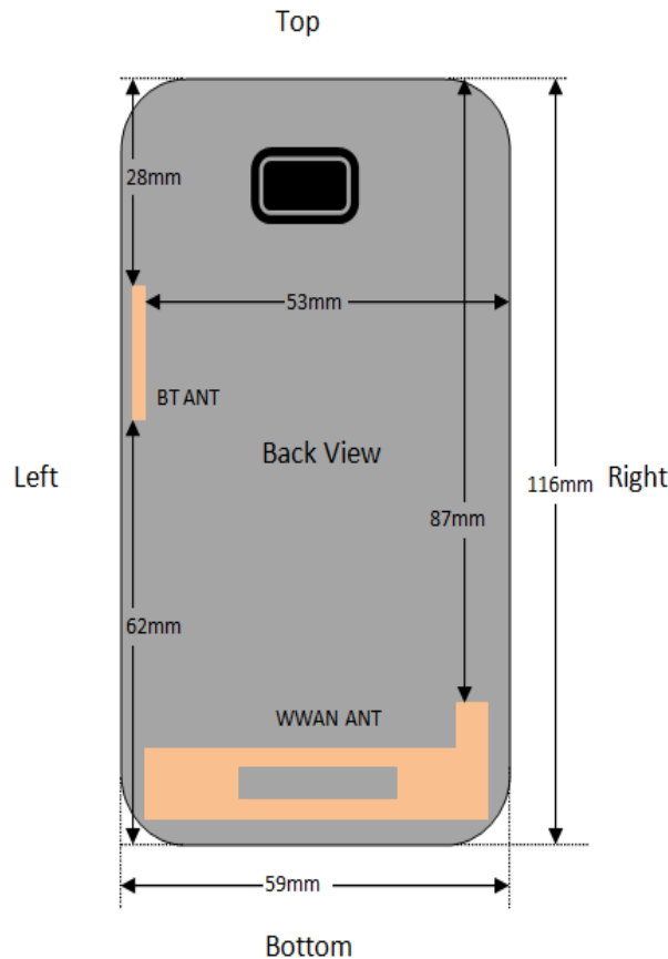
Fig.14.1 EUT Antenna Locations
