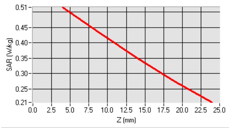
SAR, Z Axis Scan (X = 0, Y = -10)
