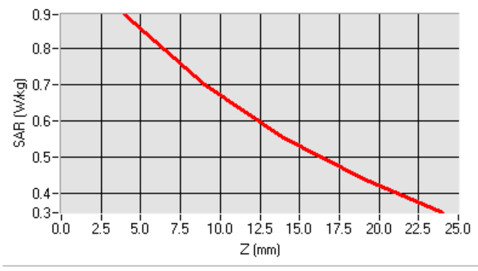
SAR, Z Axis Scan (X = -30, Y = -16)
