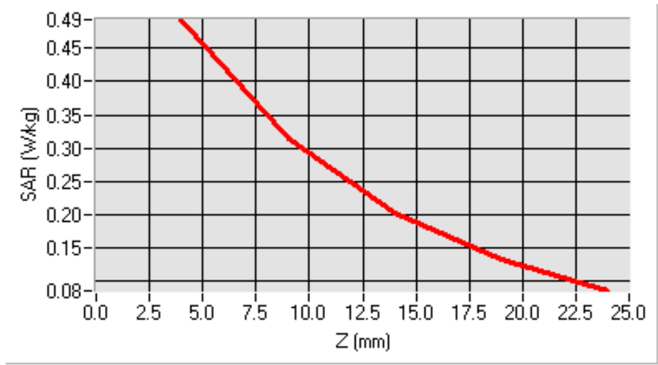
SAR, Z Axis Scan (X = -16, Y = 7)
