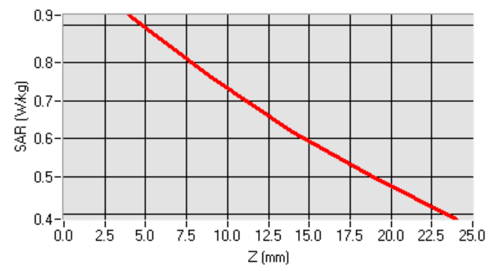
SAR, Z Axis Scan (X = 6, Y = -9)
