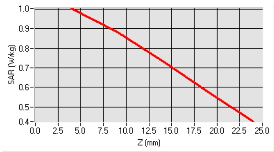
SAR, Z Axis Scan (X = -28, Y = -11)
