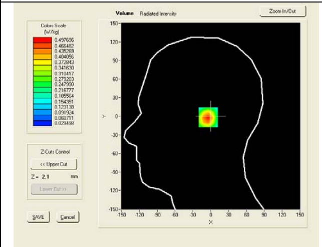
SAR, Z Axis Scan (X = 0, Y = -2)
