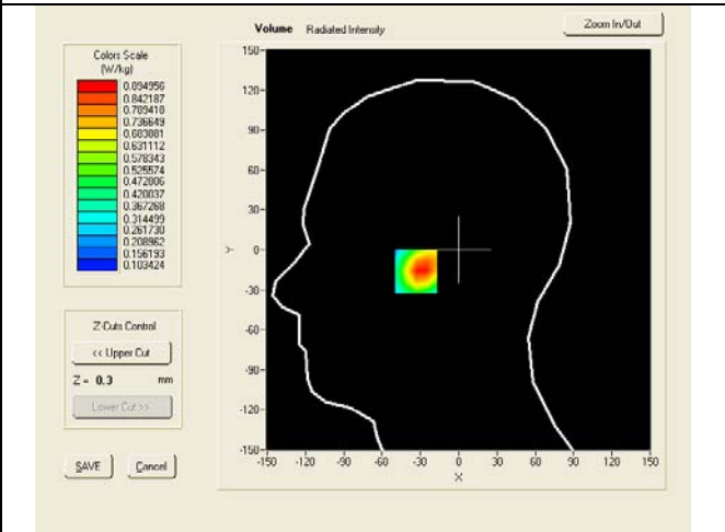
SAR, Z Axis Scan (X = -30, Y = -16)
