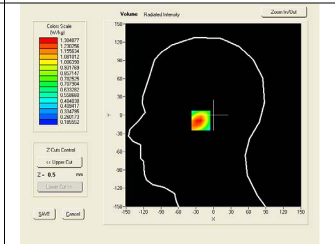
SAR, Z Axis Scan (X = -18, Y = -9)
