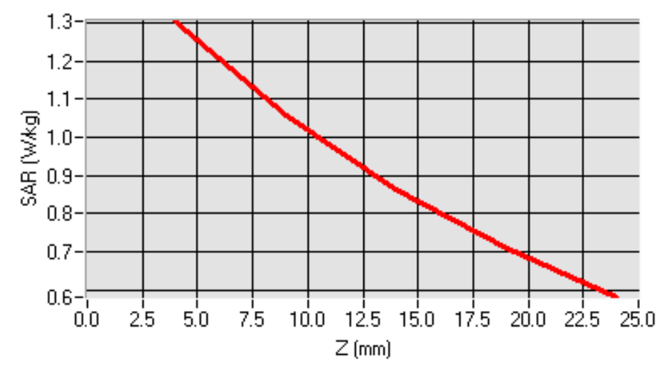
SAR, Z Axis Scan (X = -18, Y = -9)
