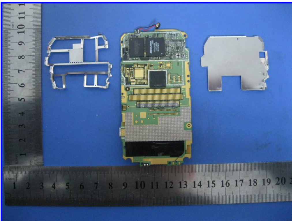
Main board unshielded top view 1
