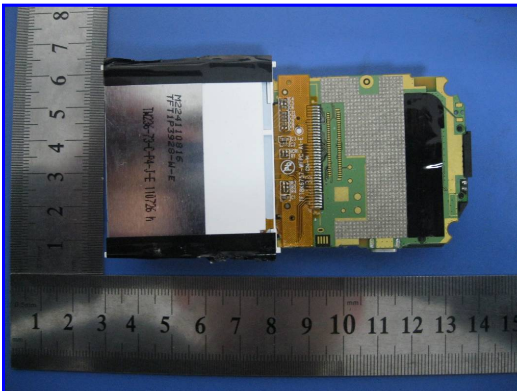
Key board and screen bottom view
