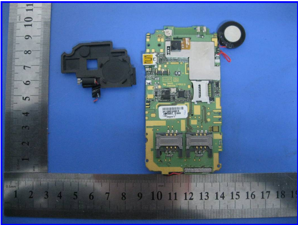
Main board bottom view 2
