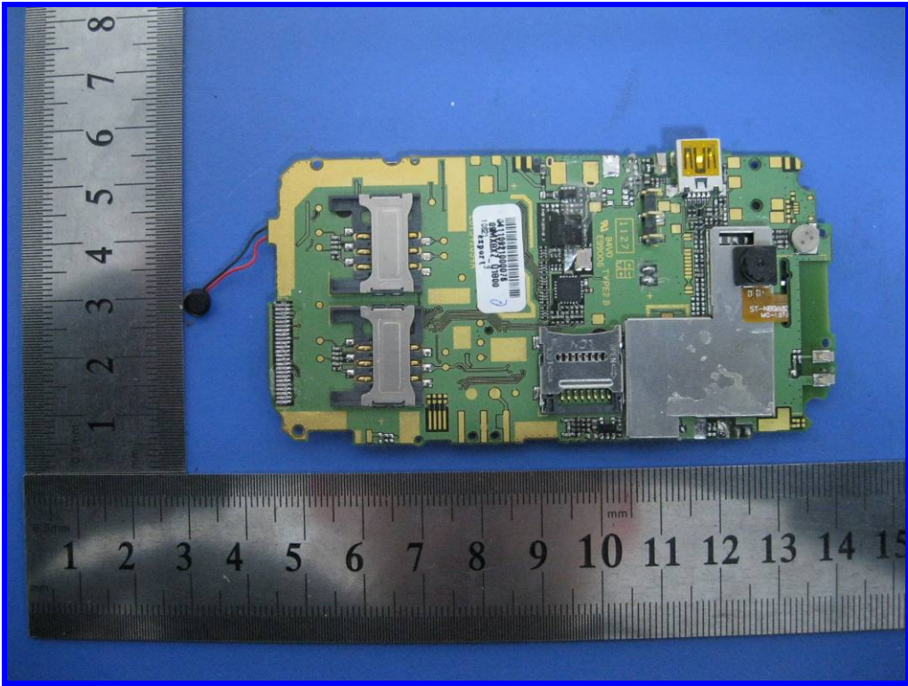
Main board bottom view 3
