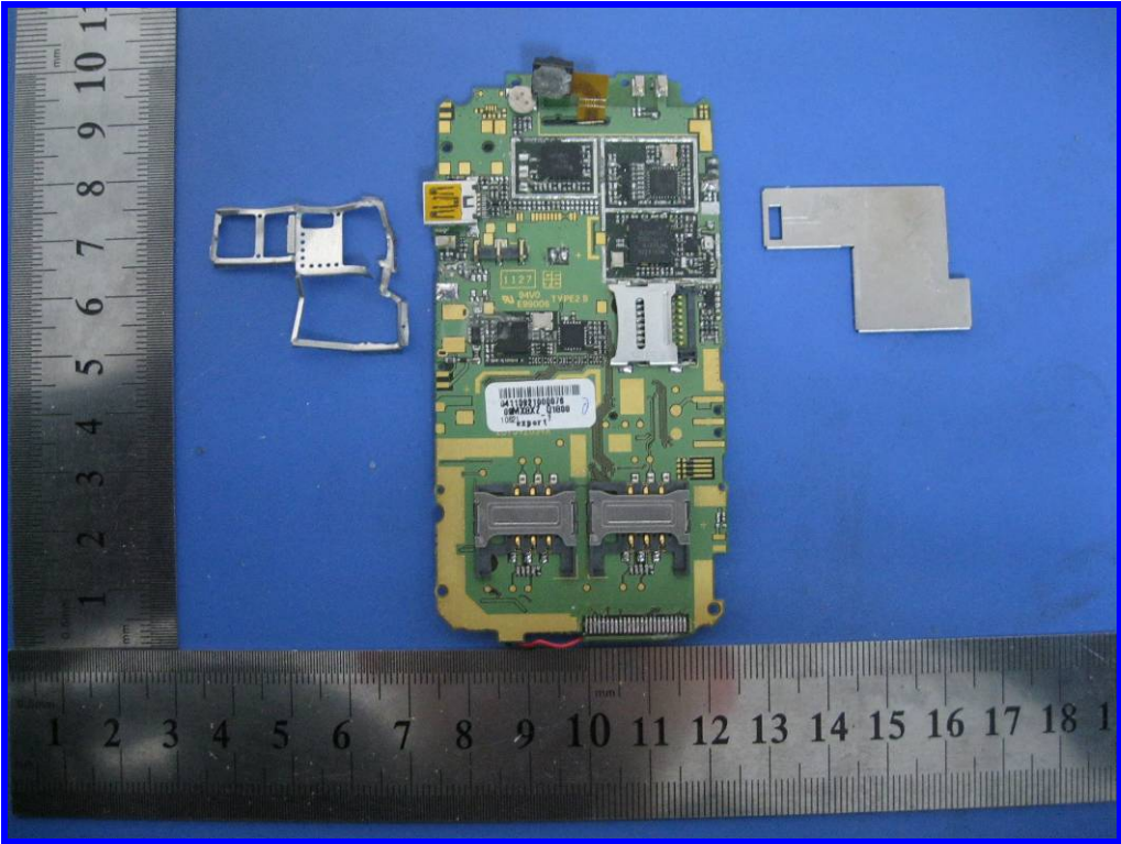
Main board unshielded top view 2
