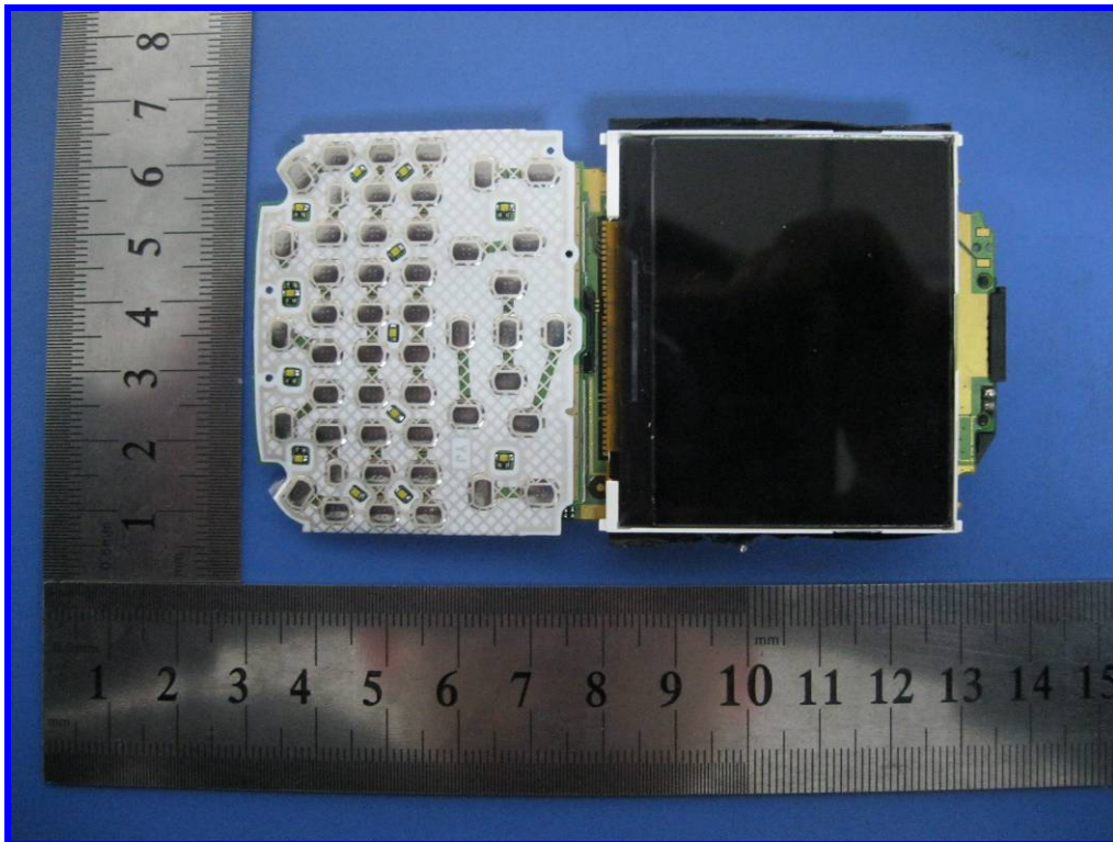
Key board and screen top view
