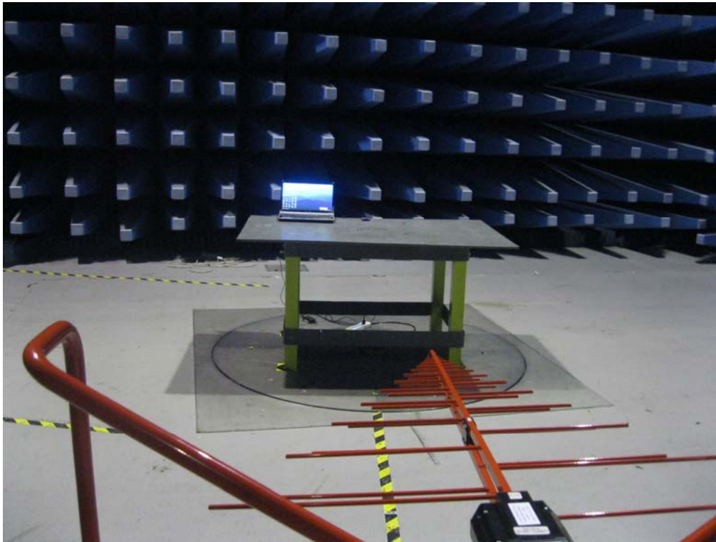
Radiated Spurious Emissions Test Setup Below 1GHz - Back View
