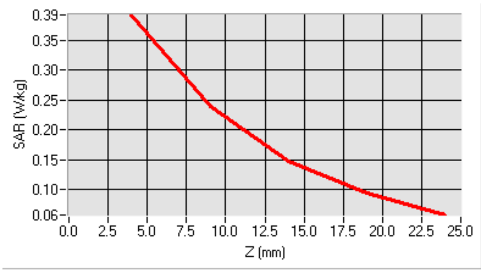
SAR, Z Axis Scan (X = -8, Y = 7)
