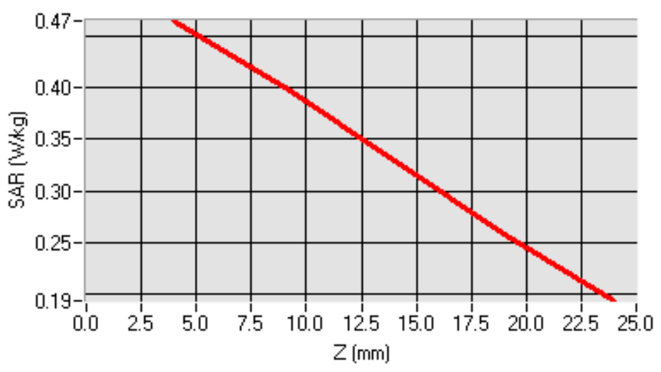
SAR, Z Axis Scan (X = -14, Y = 0)
