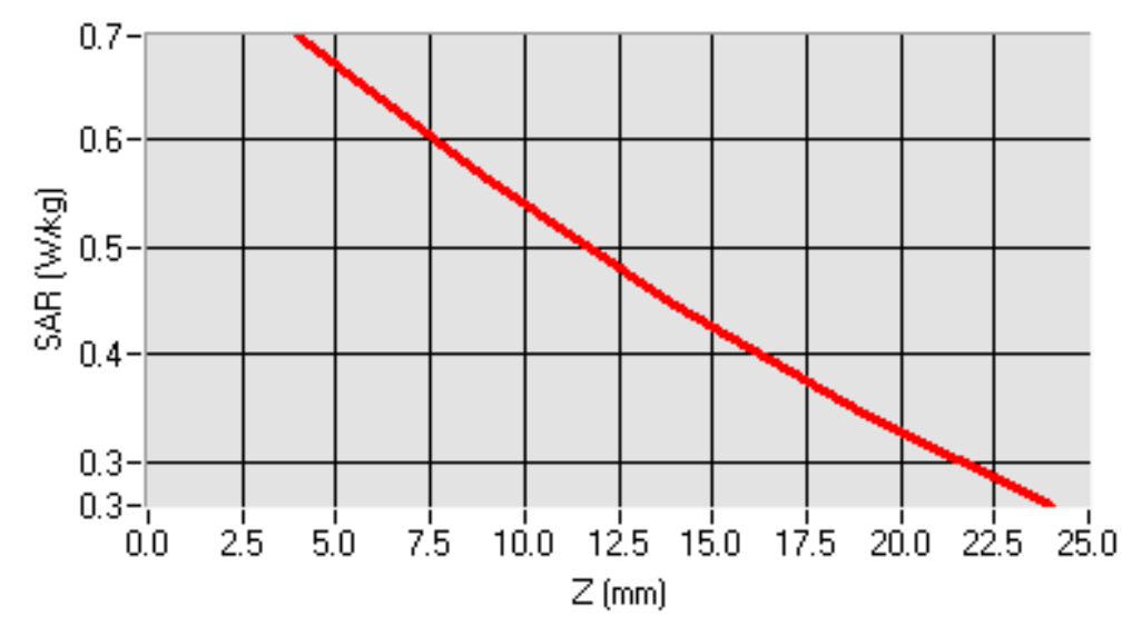
SAR, Z Axis Scan (X = -23, Y = -7)
