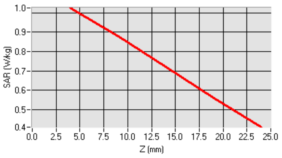
SAR, Z Axis Scan (X = -11, Y = 1)
