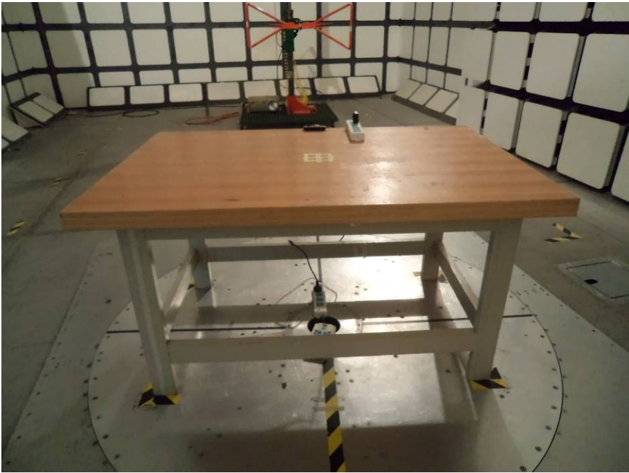
Radiated Emissions-Front View (Charging and play video&audio file mode)
